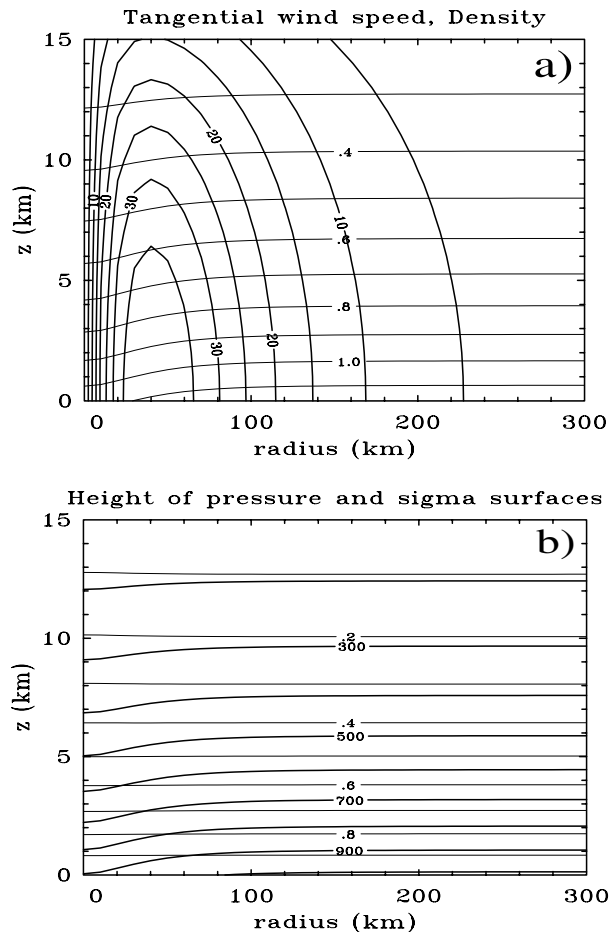
Fig. 2. (a) Isotachs of tangential wind speed v (thick solid lines, contour interval 5 \text{ m s}^{-1} ) and isopleths of constant density \rho (thin solid lines, contour interval 0.1 \text{ kg m}^{-3} ) in a vertical plane through the axis of a balanced, axisymmetric, tropical-cyclone-scale vortex. (b) Surfaces of constant pressure p (thick solid lines, contour interval 100 mb) and constant \sigma (thin solid lines, contour interval 0.1).
