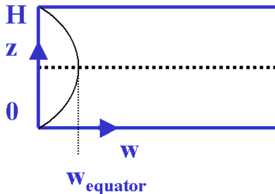
Figure 4.9: Vertical velocity structure in the solution of the Held-Hou model.
