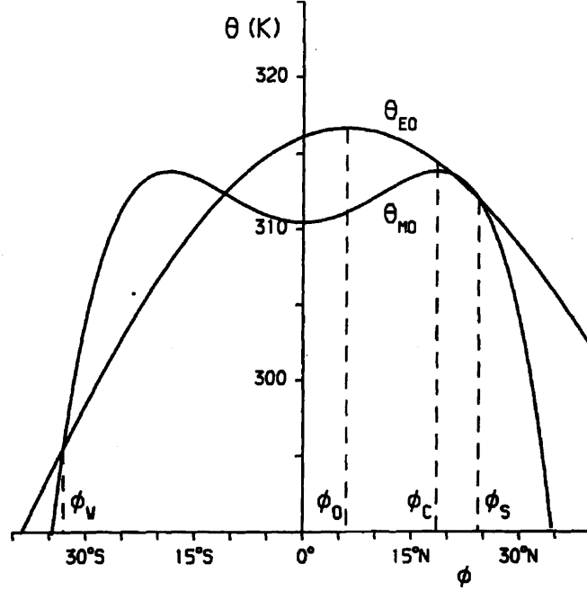
Figure 4.11: The Held-Hou model for asymmetric heating with maximum value at 6^\circ N. Here \phi_W, \phi_0, \phi_C and \phi_S correspond with y = Y_-, Y_0, Y_1 and Y_+ in Fig. (4.10). (From James, 1994)
