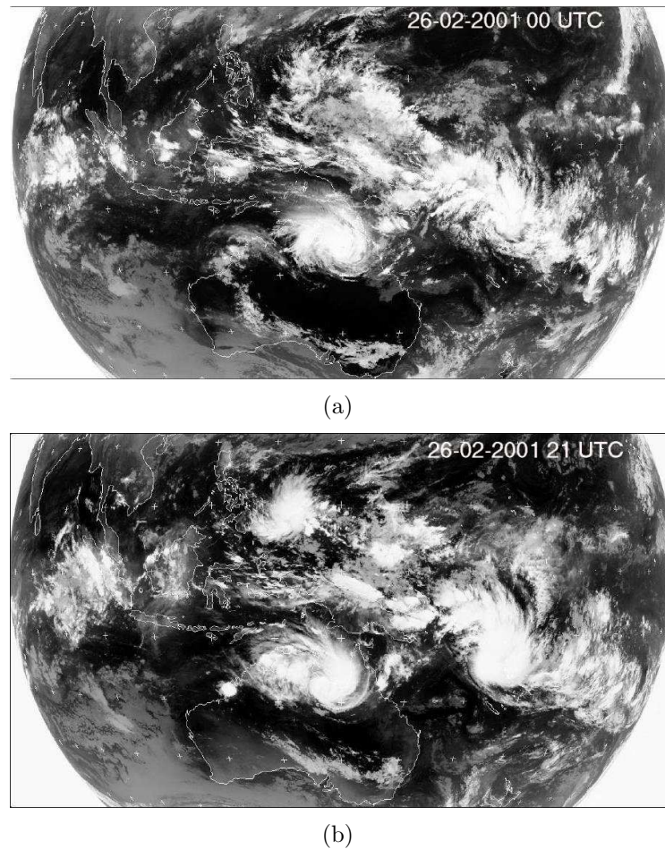
Figure 7.5: GMS-IR satellite images for 26 February 2001, (a) 0000 UTC, (b) 2100 UTC.
