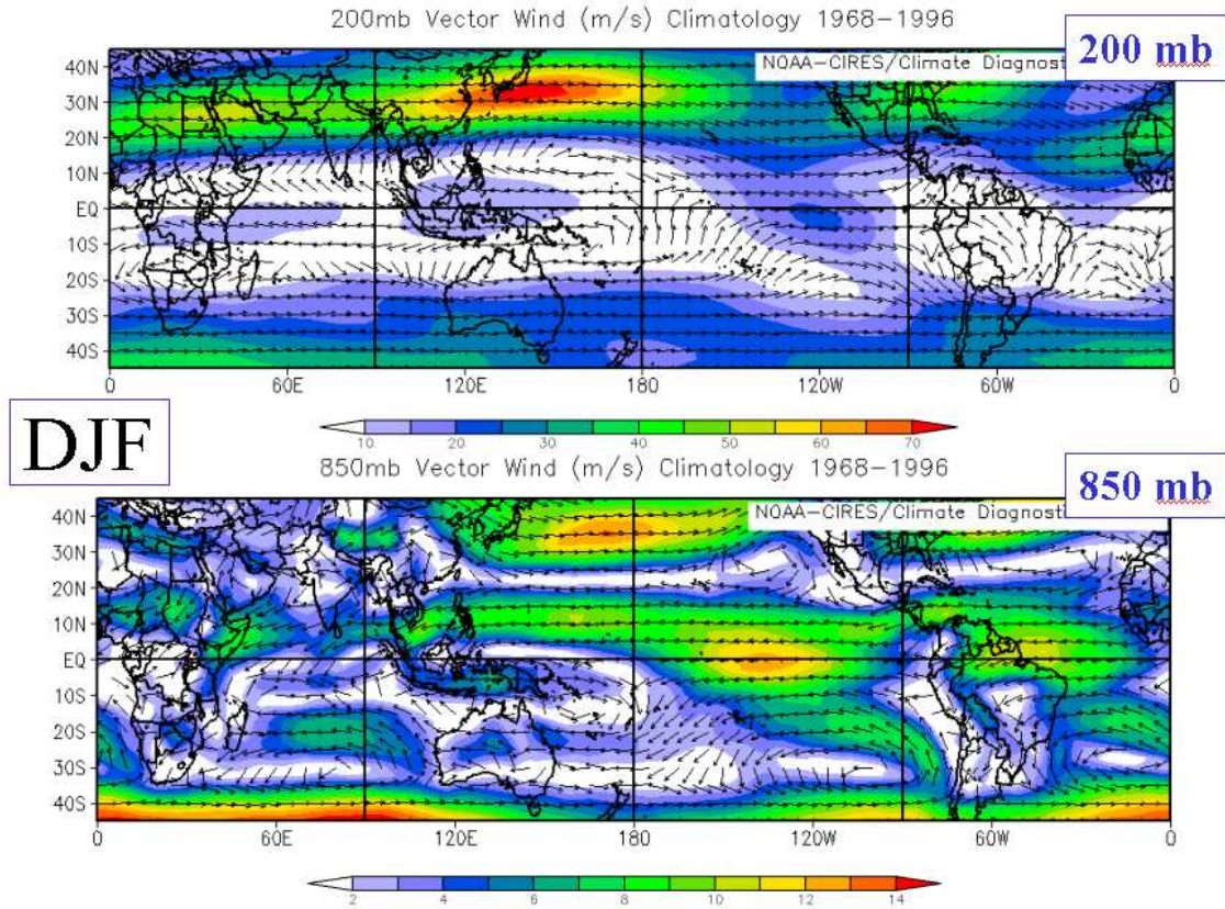
Figure 1.12: As in Fig. 1.11, but for DJF.
