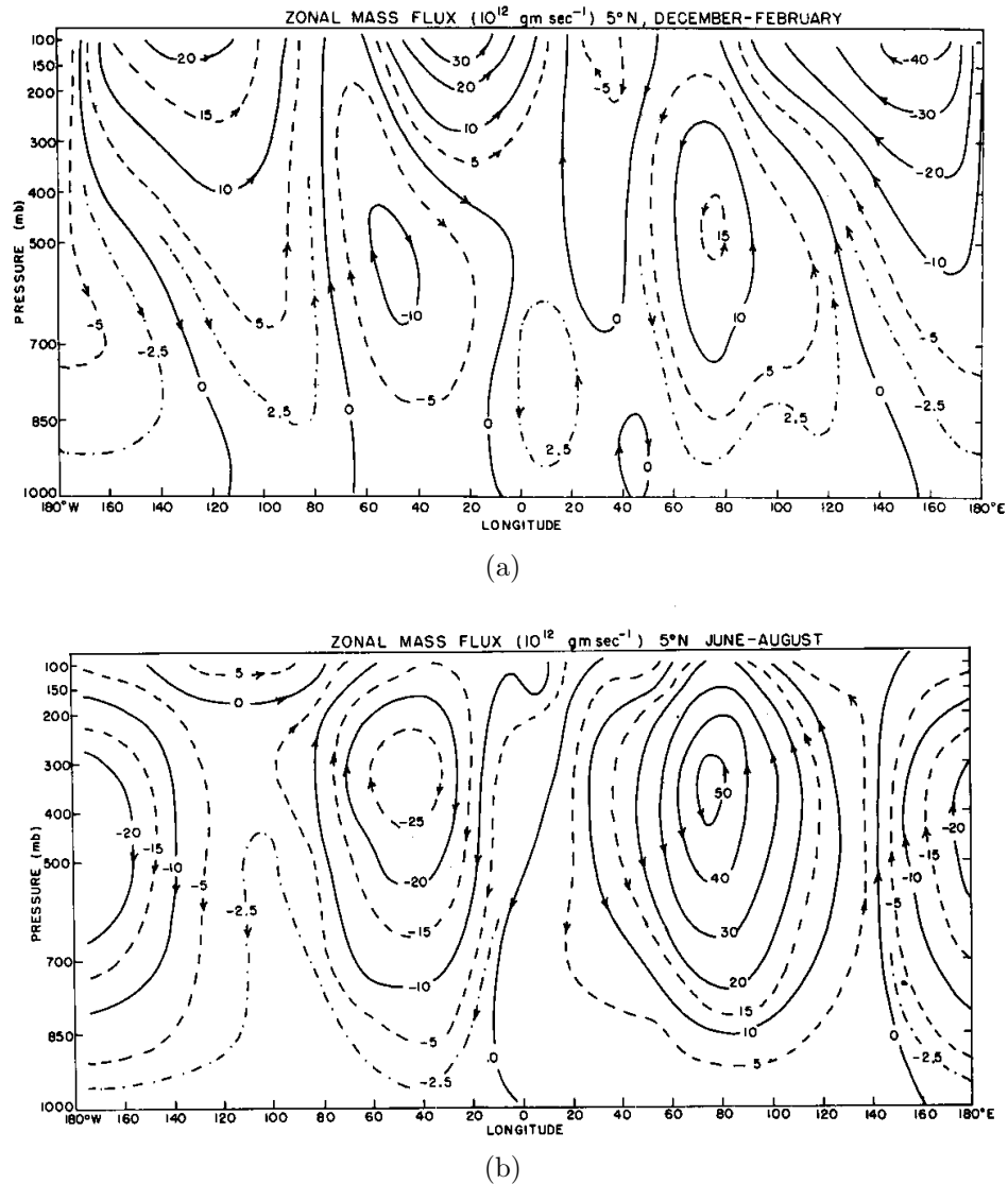
Figure 1.21: Deviations of the zonal mass flux, averaged over the latitude belt 0^{\circ} - 10^{\circ} N, from the zonal mean, for the periods (a) December - February, and (b) June - August calculated by Newell et al. (1974). Contours do not correspond with streamlines, but give a fairly good representation of the velocity field associated with the Walker Circulation.
