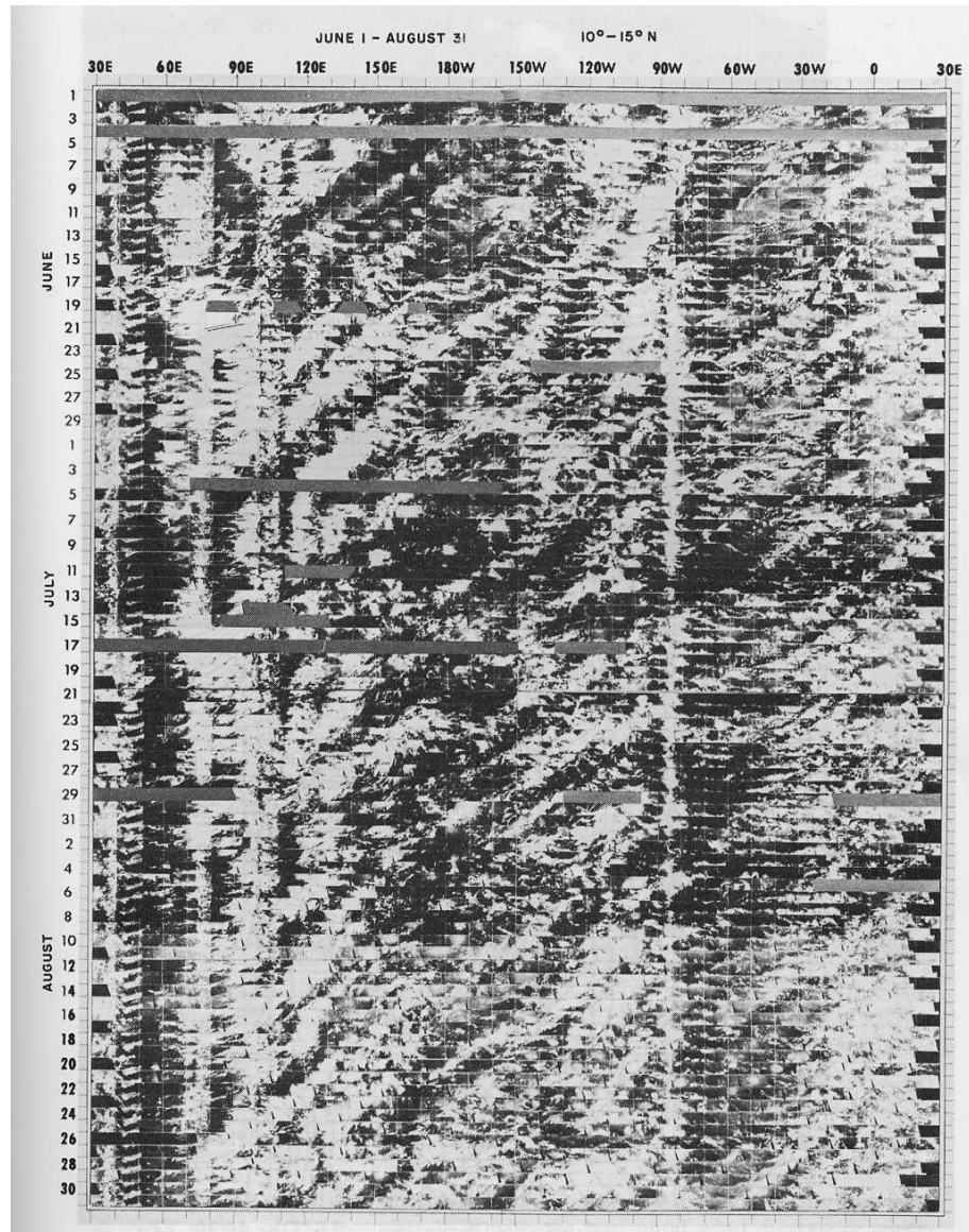
Figure 1.29: Time-longitude section of visible satellite imagery for the latitude band 10-15°N of the tropics. Cloud streaks moving from right to left with increasing time denotes westward propagation. Note that there is typically easterly flow at these latitudes. (From Wallace, 1970)
