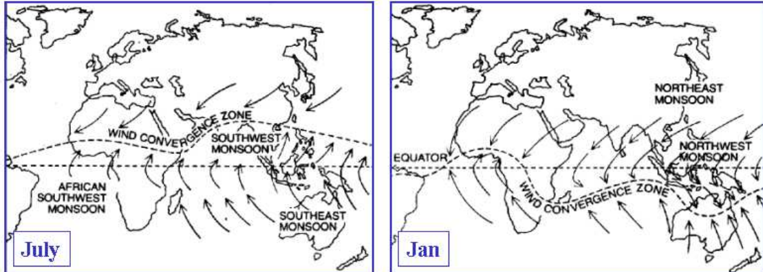
Figure 1.26: Schematic of low-level air flow patterns near the Equator in January and July showing the main regions of cross equatorial flow in the monsoon regions.
