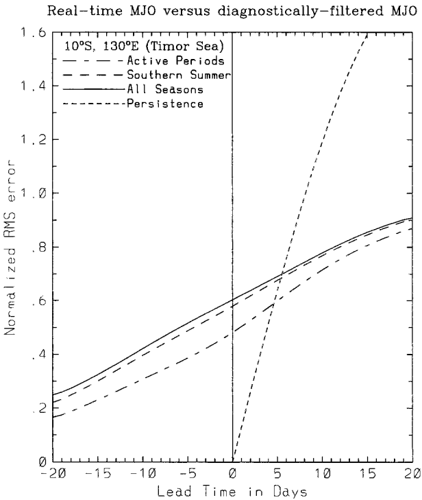
FIG. 9. As in Fig. 8 except for the normalized rms error between the real-time filtered MJO OLR and the diagnostically filtered MJO OLR at the point 10°S, 130°E. Also shown is the normalized rms error for a persistence (of the diagnostically filtered field) forecast. Note that this persistence forecast cannot be performed in real time.
