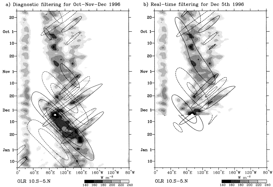
FIG. 3. (a) Time–longitude plot of the total OLR (with R21 spatial truncation, and a 1–2–1 filter applied in time) and filtered OLR anomalies averaged between 10°S and 5°N during late 1996 to early 1997. Shading is for the total OLR, and contours are for the diagnostically filtered anomalies of the MJO and n = 1 ER wave. Solid contours represent negative OLR anomalies, while dashed contours are for positive anomalies, with the contour interval for both wave filtered bands being 10 \text{ W m}^{-2} , and the zero contour omitted. (b) Same as in (a) except that the filtering was performed with the last day of data being on 5 Dec 1996. After 5 Dec, when the real-time filtered anomalies are continued into the future as a forecast, the contour interval is halved.
