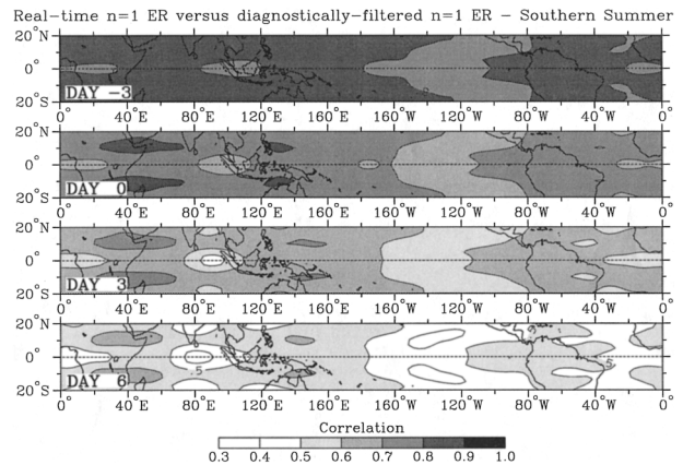
FIG. 12. As in Fig. 7 except for the correlations of the n = 1 ER wave real-time filtered OLR for southern summer only.
