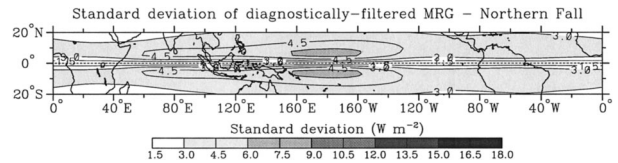
FIG. 19. As in Fig. 6 except for the MRG wave, and for the season of northern fall (defined as Aug–Jan) only.
