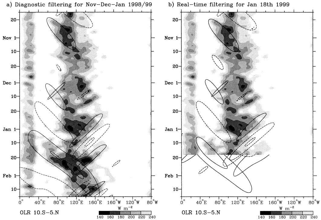
FIG. 5. (a) Same as in Fig. 3a except for the 1998/99 period. (b) Same as in Fig. 3b except for the real-time filtering of 18 Jan 1999.
