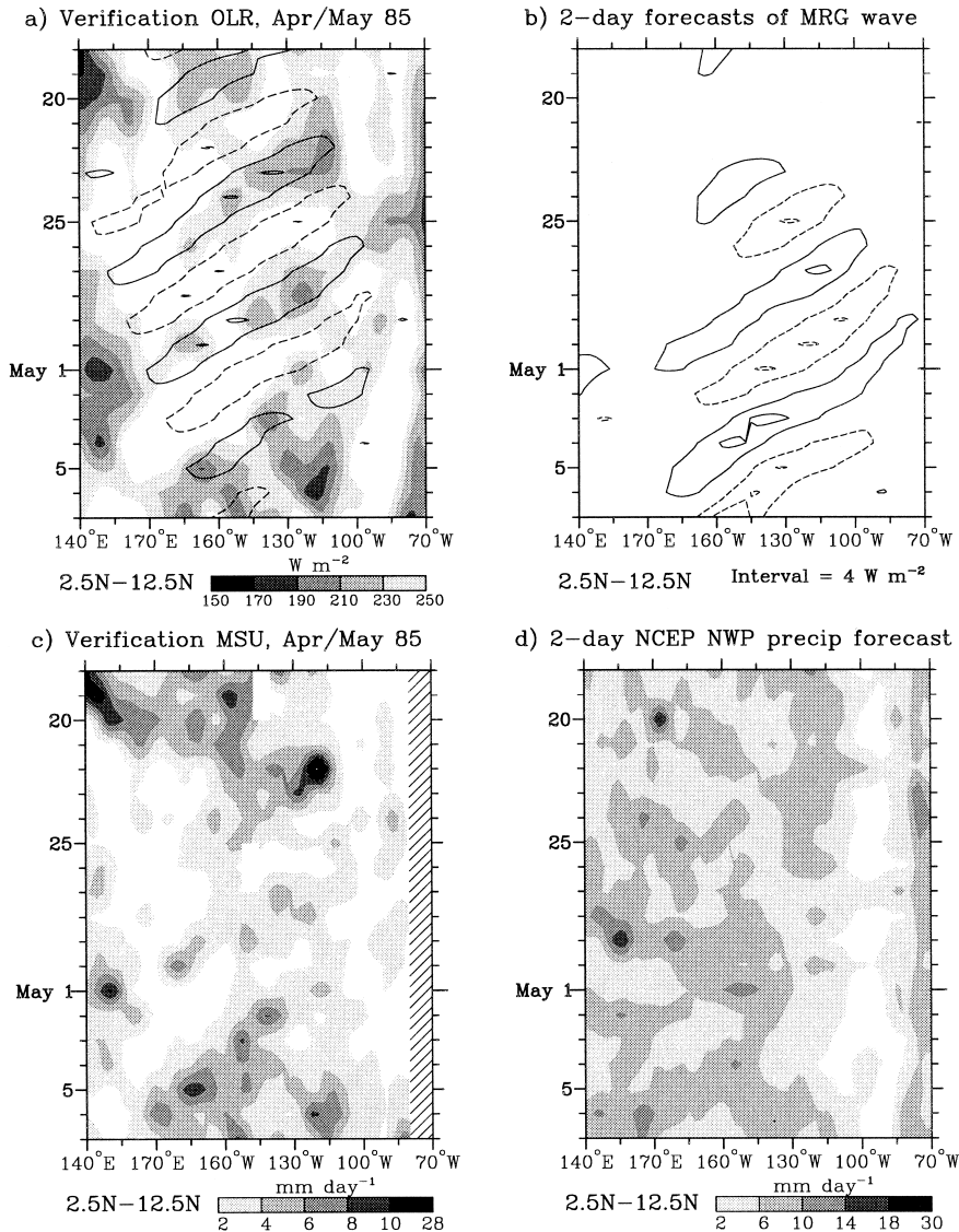
FIG. 24. (a) As in Fig. 23a except for the period, latitudes, and longitudes as specified, showing the MRG wave diagnostic filtering, and without a 1–2–1 filter applied in time. Contour interval for the MRG wave filtering is 7 W m^{-2} . (b) Time–longitude plot of the 2-day real-time filtering forecasts of the MRG wave OLR that verify on the days as specified. Contour interval is as specified. (c) Time–longitude plot of the verifying MSU precipitation. Missing data is left blank and land areas hatched. Spatial smoothing applied to mimic that of the OLR in (a). (d) As in (b) except for the 2-day forecasts of precipitation from the NCEP model in mm day^{-1} , and spatial smoothing applied to match (a).
