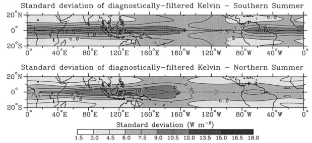
FIG. 15. As in Fig. 6 except for the Kelvin wave.
