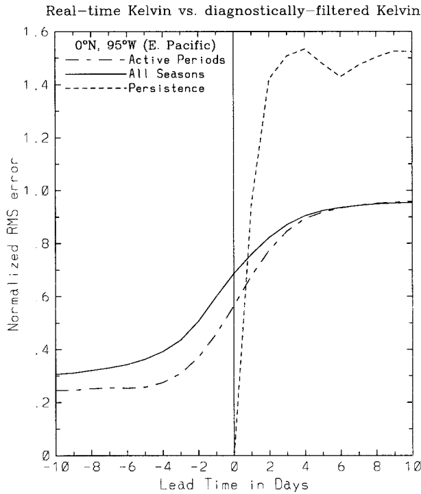
FIG. 17. As in Fig. 9 except for the Kelvin wave OLR real-time filtering at the point 0°N, 95°W.
