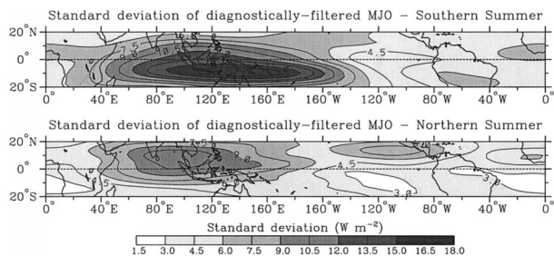
FIG. 6. Standard deviation of the diagnostically filtered MJO OLR for the 10-yr period of 1985–94, separately for southern summer (above) and northern summer (below).
