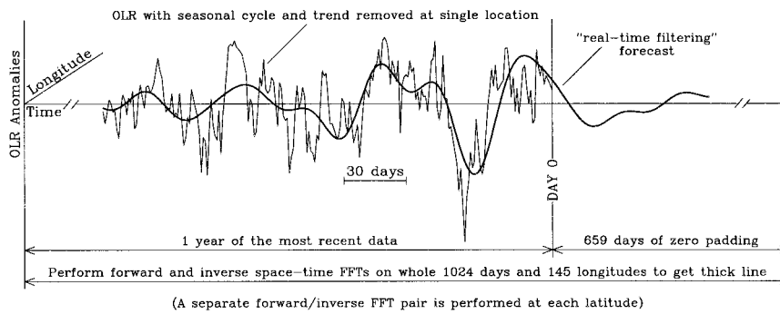
FIG. 2. Schematic of the procedure of real-time filtering for monitoring and prediction, as applied to a time series with an MJO-like signal.
