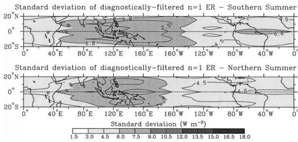
FIG. 11. As in Fig. 6 except for the n = 1 ER wave.
