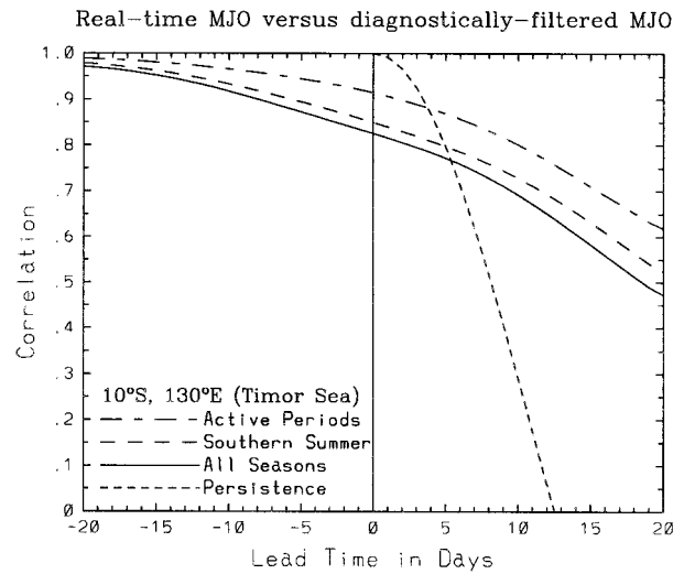
FIG. 8. Correlations of the MJO real-time filtered OLR with the validating diagnostically filtered MJO OLR at the point 10°S, 130°E as a function of lead time. The correlations were calculated using all seasons, southern summer only, and “active” periods only of the 10 yr of sample forecasts, as labeled. Additionally shown are correlations for a persistence forecast with the diagnostically filtered MJO OLR at this point, equivalent to its autocorrelation function at this point. Note that this “persistence forecast” cannot be performed in real time.
