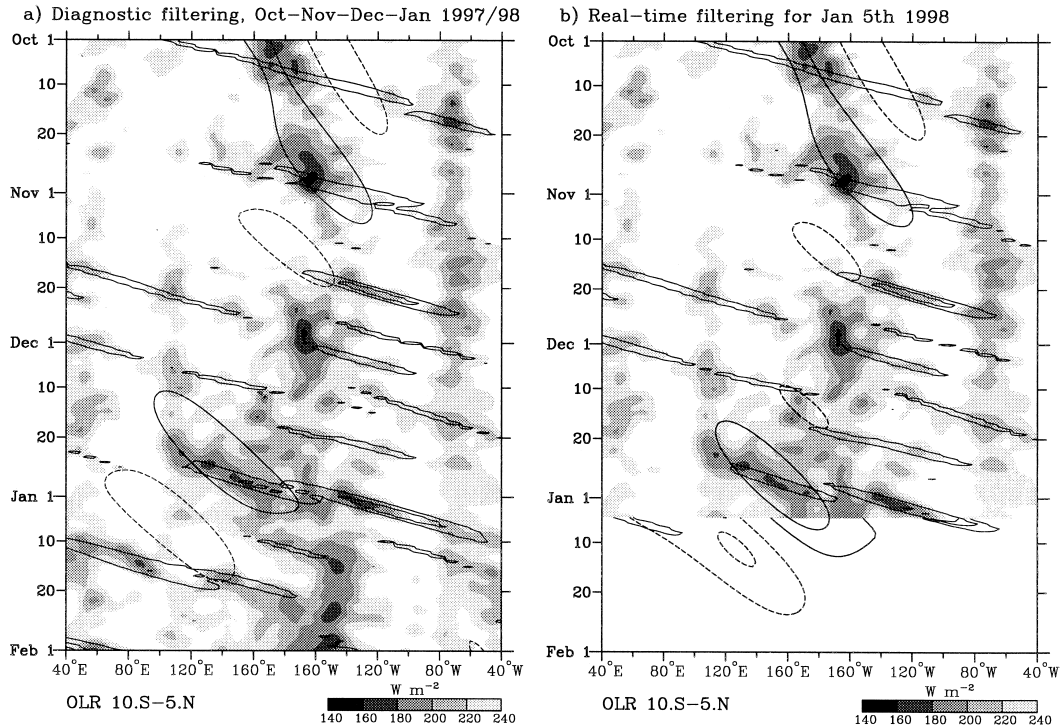
FIG. 4. (a) Same as in Fig. 3a except for the 1997/98 period, and the MJO and Kelvin wave filtering are displayed. The range of longitudes has also been shifted by 40^\circ . Contour interval for the MJO filtered anomalies is 10 \text{ W m}^{-2} , and for the Kelvin wave anomalies is 15 \text{ W m}^{-2} . Positive contours of the Kelvin wave anomalies are omitted. (b) Same as in Fig. 3b except for the real-time filtering of 5 Jan 1998, and only the MJO and Kelvin wave anomalies are displayed.
