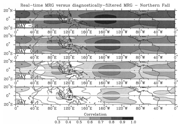
FIG. 20. As in Fig. 7 except for the correlations of the MRG wave real-time filtered OLR for northern fall only. The correlation is not shown at the equator as the defined antisymmetric OLR field of the MRG waves is zero there.
