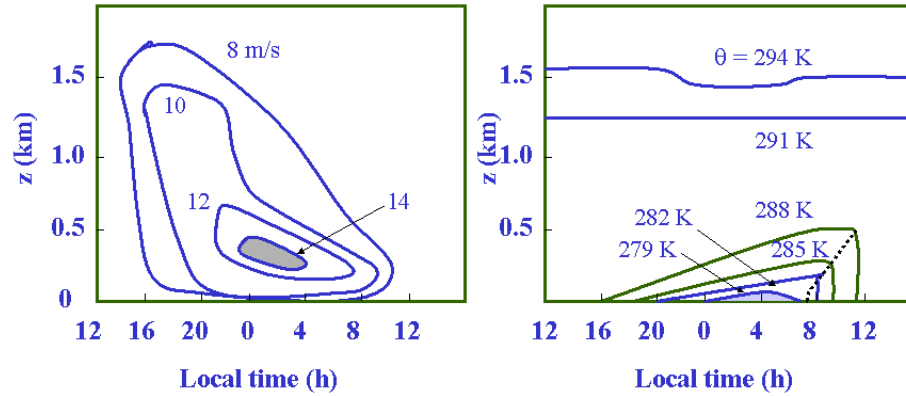
Figure 11.6: (a) wind speed and (b) potential temperature evolution during Night 13-14 of the Wangara experiment. Adapted from (Malcher and Krauss, 1983).
