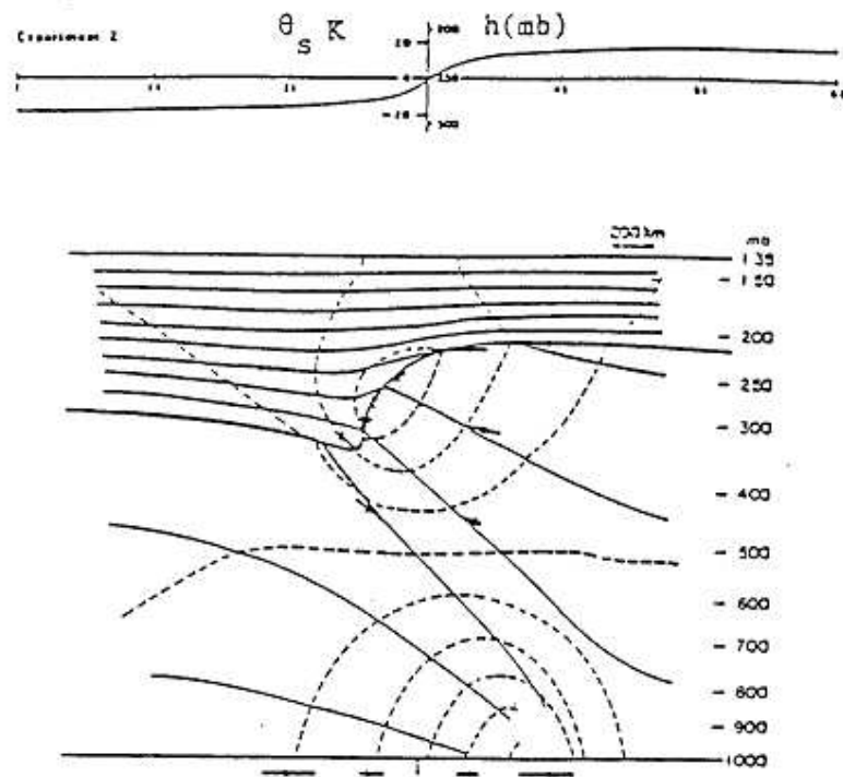
Figure 14.18: (a) Surface temperature distribution \theta_s (K) and tropopause height h (mb) if there were no induced geostrophic motion. (b) Two-layer model of frontal development in the large scale deformation field (14.1). Thick continuous lines denote isentropes of potential temperature, broken lines denote isotachs of long front velocity and a cross denotes the point of maximum wind. The arrows above 1000 mb denote particle motions; those below the diagram represent the basic deformation motion. (from (Hoskins, 1971))
