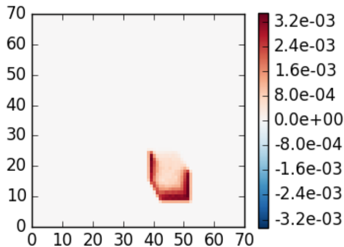
SPARTA case 3, \theta_0=20 , z=0 , \theta=40 , \phi=120
