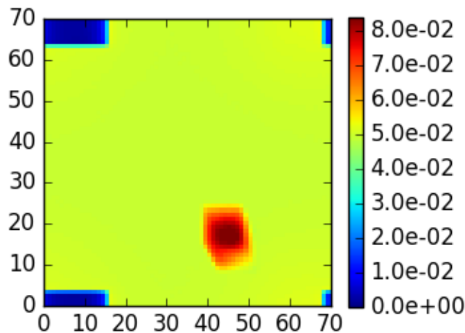
SPARTA case 8, \theta_0=40 , z=5 , \theta=140 , \phi=120
