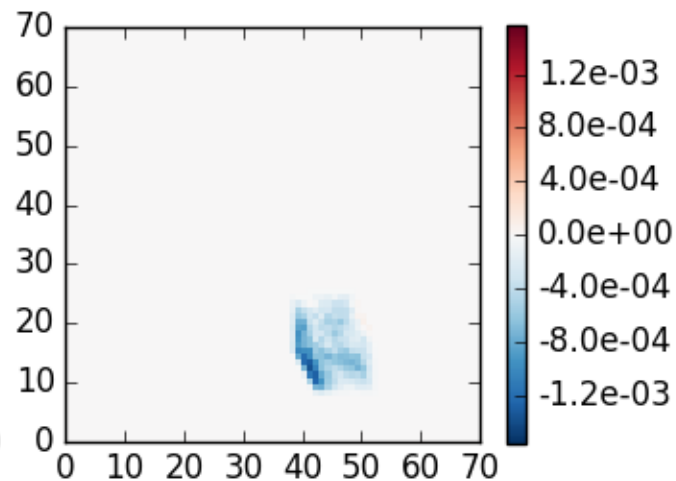
SPARTA case 8, \theta_0=40 , z=5 , \theta=140 , \phi=120
