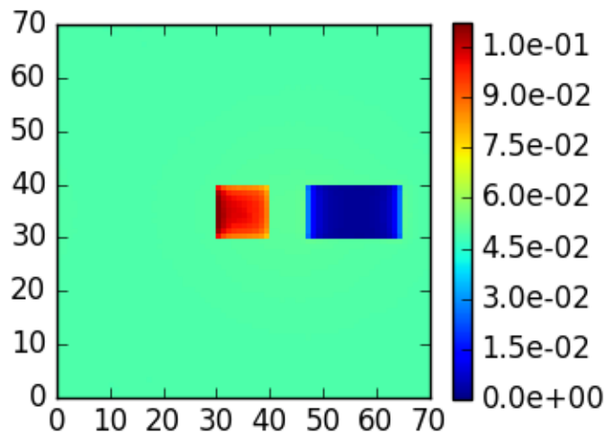
SPARTA case 5, \theta_0=40 , z=5 , \theta=180 , \phi=0
