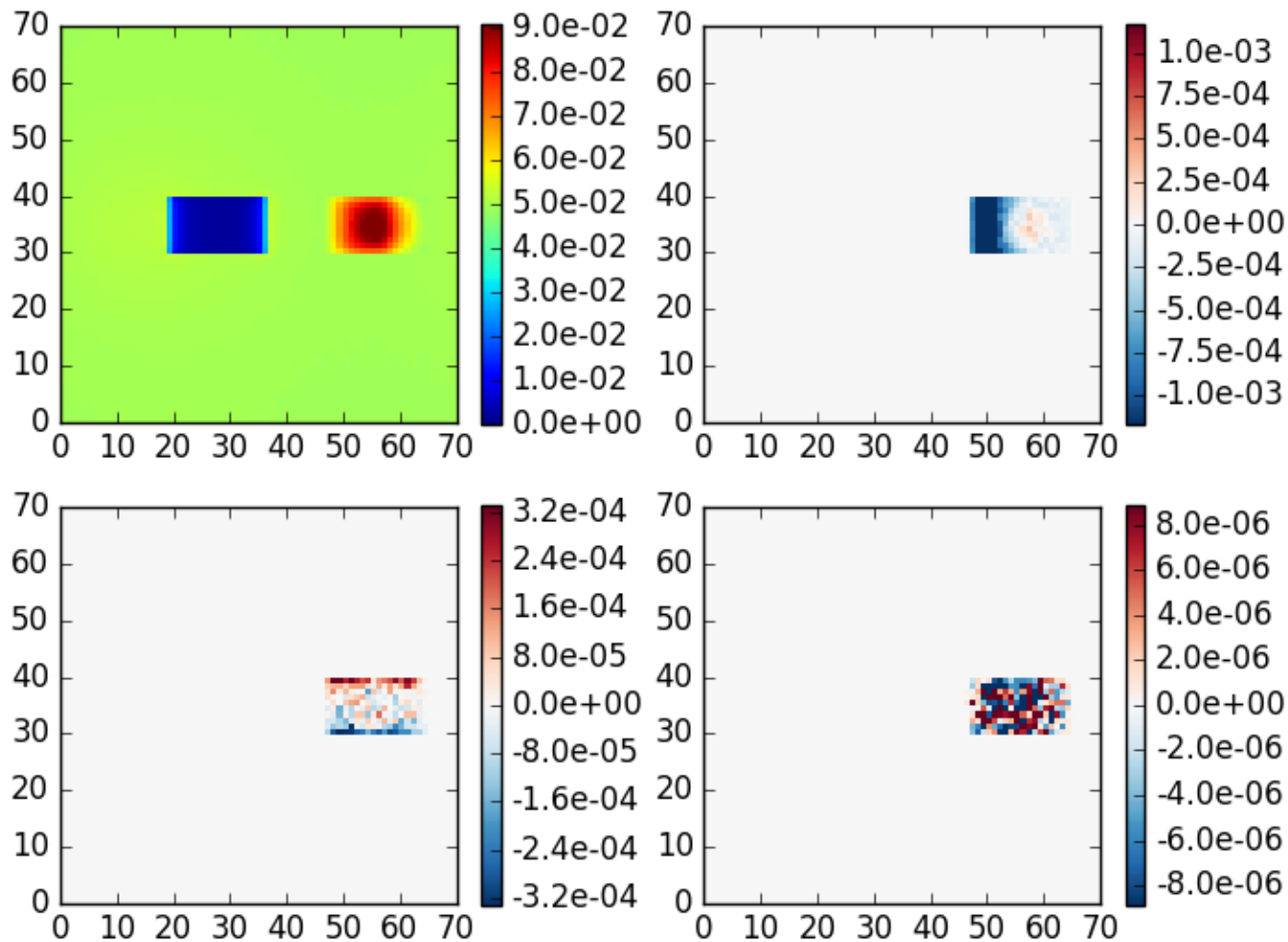
SPARTA case 9, \theta_0=40 , z=5 , \theta=140 , \phi=180
