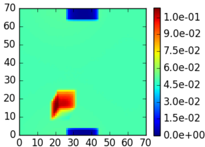
SPARTA case 7, \theta_0=40 , z=5 , \theta=140 , \phi=60
