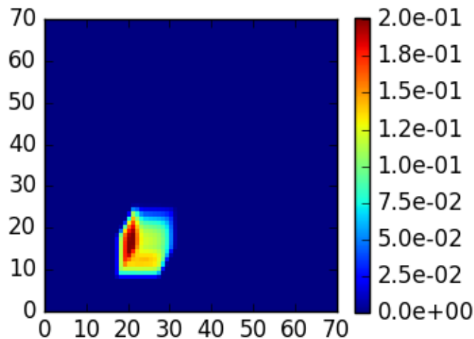
SPARTA case 2, \theta_0=20 , z=0 , \theta=40 , \phi=60
