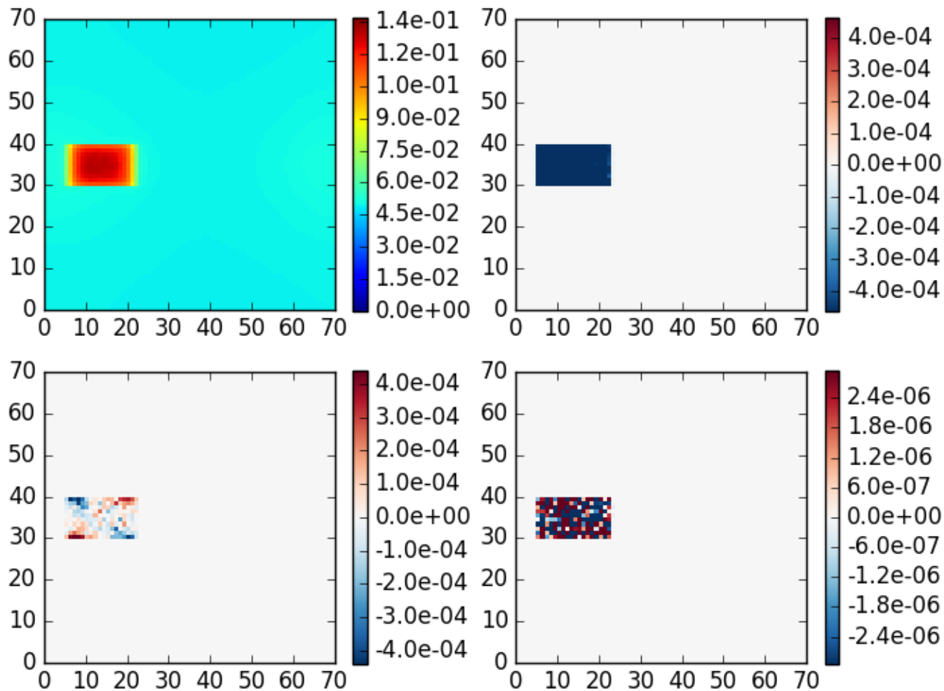
SPARTA case 6, \theta_0=40 , z=5 , \theta=140 , \phi=0
