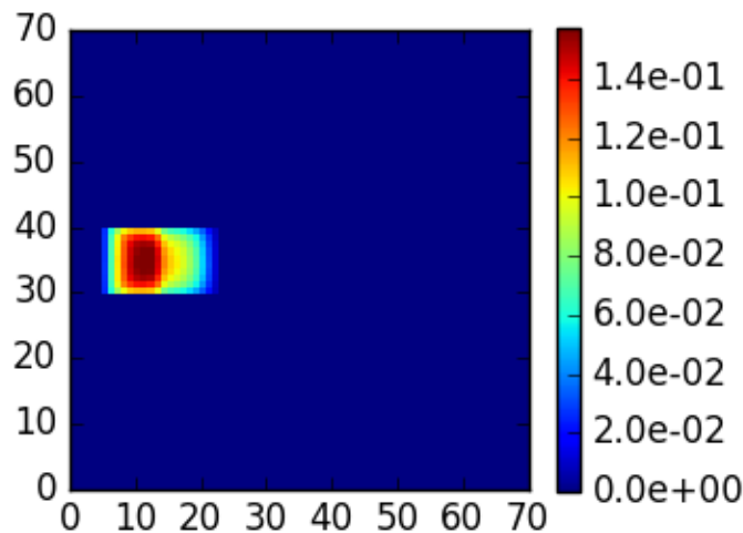
SPARTA case 1, \theta_0=20 , z=0 , \theta=40 , \phi=0
