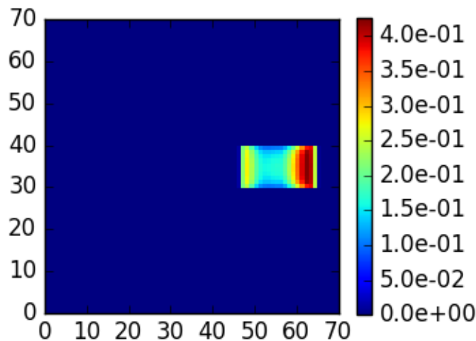
SPARTA case 4, \theta_0=20 , z=0 , \theta=40 , \phi=180
