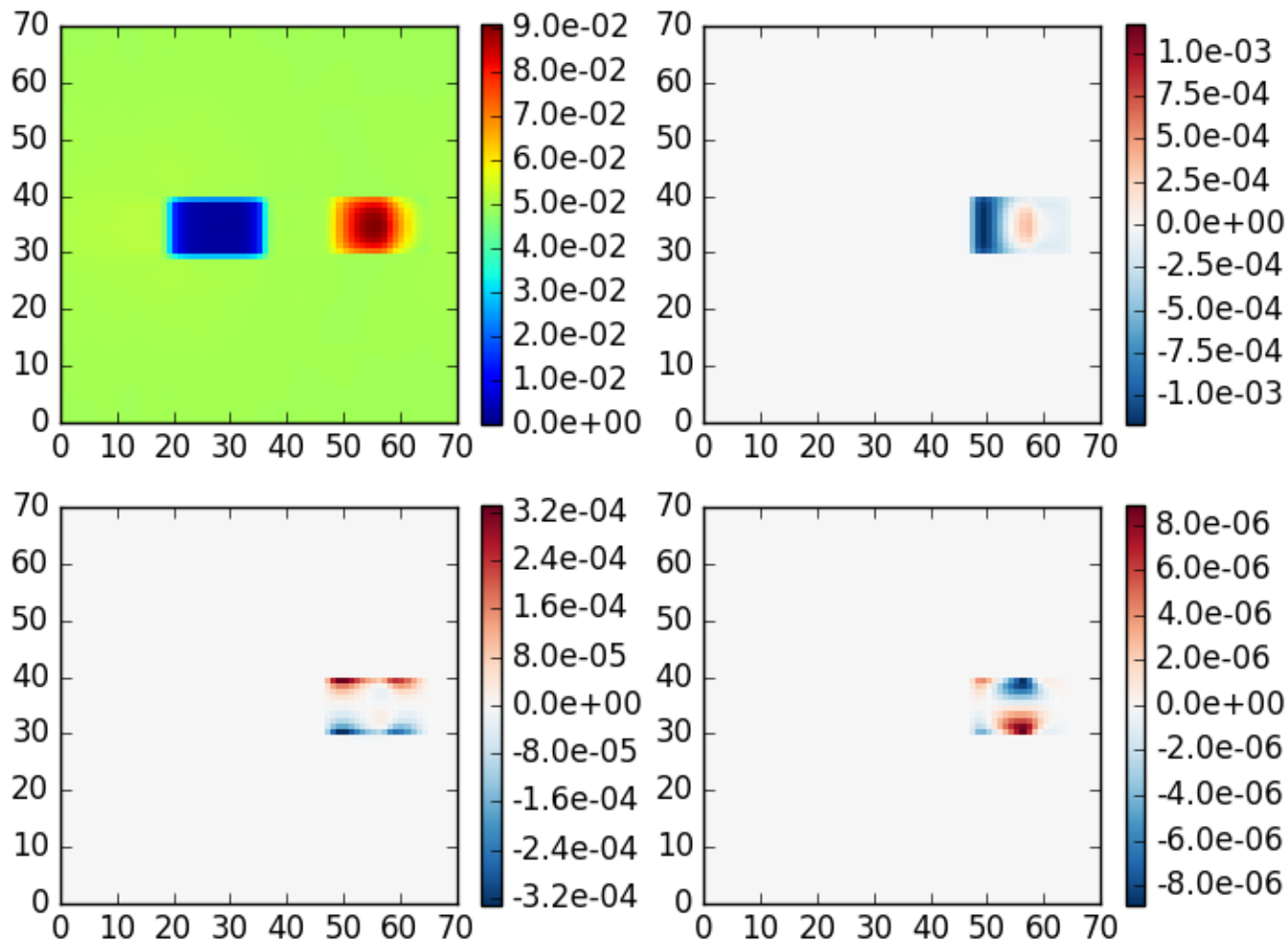
shdom3 case 9, \theta_0=40 , z=5 , \theta=140 , \phi=180
