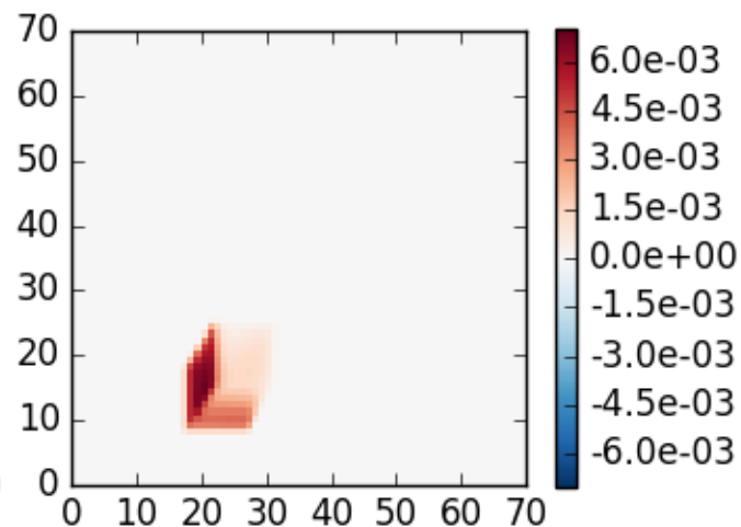
mystic case 2, \theta_0=20 , z=0 , \theta=40 , \phi=60
