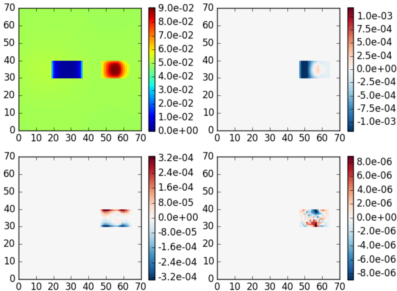
mystic case 9, \theta_0=40 , z=5 , \theta=140 , \phi=180
