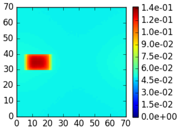
mystic case 6, \theta_0=40 , z=5 , \theta=140 , \phi=0
