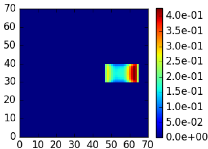
mystic case 4, \theta_0=20 , z=0 , \theta=40 , \phi=180
