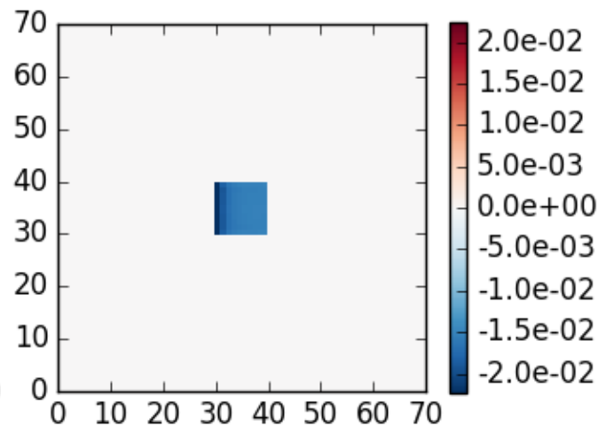
mystic case 5, \theta_0=40 , z=5 , \theta=180 , \phi=0
