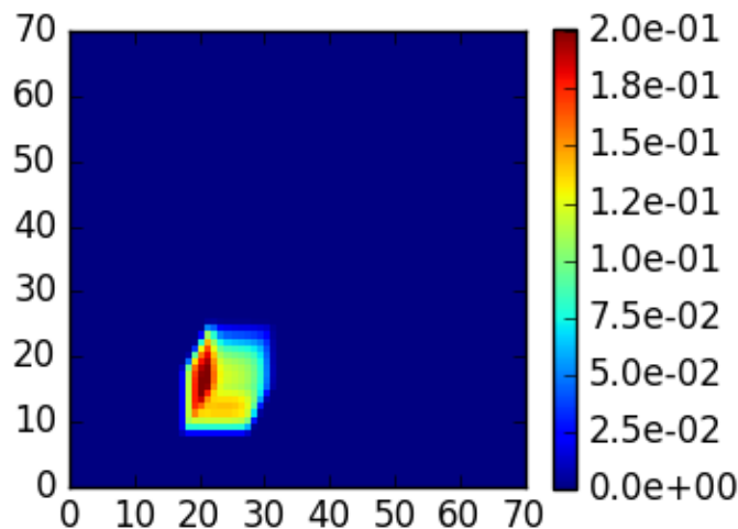
mystic case 2, \theta_0=20 , z=0 , \theta=40 , \phi=60
