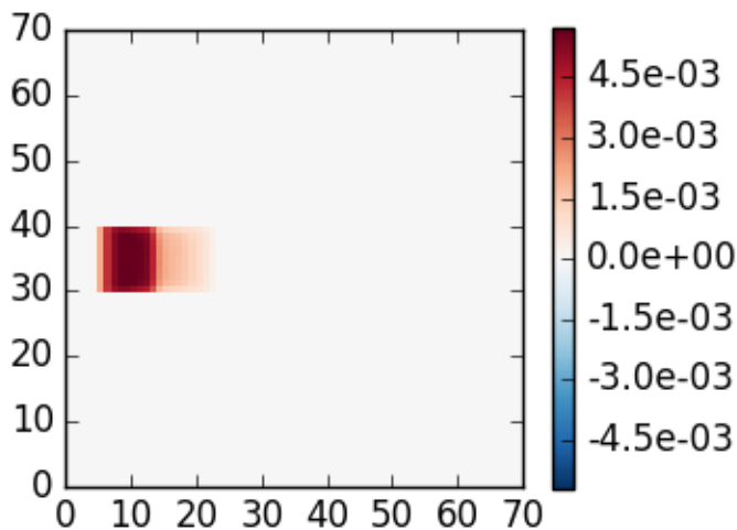
mystic case 1, \theta_0=20 , z=0 , \theta=40 , \phi=0
