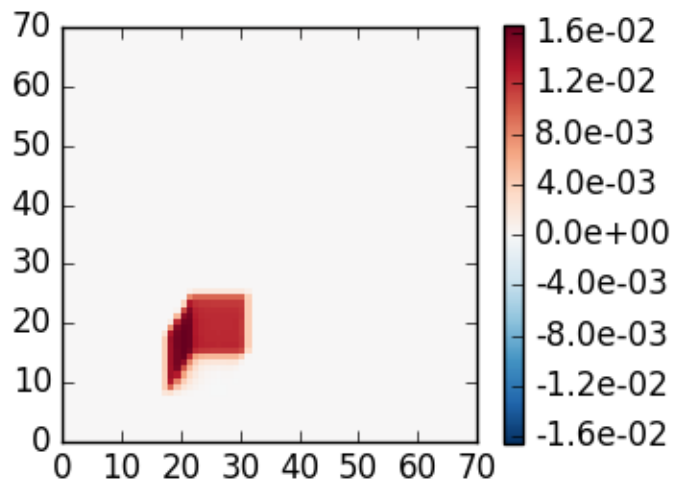
mystic case 7, \theta_0=40 , z=5 , \theta=140 , \phi=60
