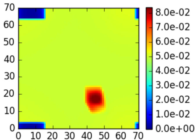
mystic case 8, \theta_0=40 , z=5 , \theta=140 , \phi=120
