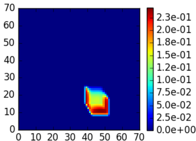
mystic case 3, \theta_0=20 , z=0 , \theta=40 , \phi=120
