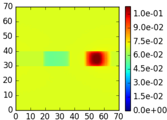
mystic case 9, \theta_0=40 , z=5 , \theta=140 , \phi=180
