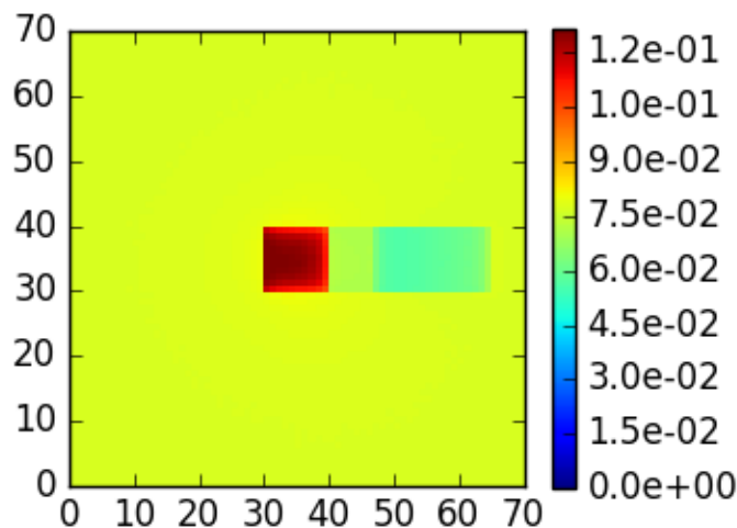
mscart_fmc case 5, \theta_0=40 , z=5 , \theta=180 , \phi=0
