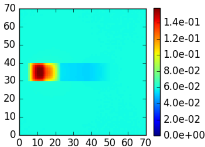
mcart_fmccase 1, \theta_0=20 , z=0 , \theta=40 , \phi=0
