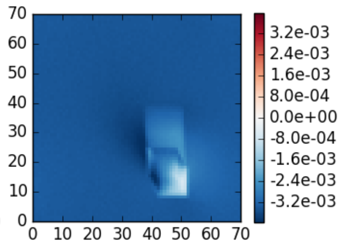
mscart_fmc case 3, \theta_0=20 , z=0 , \theta=40 , \phi=120
