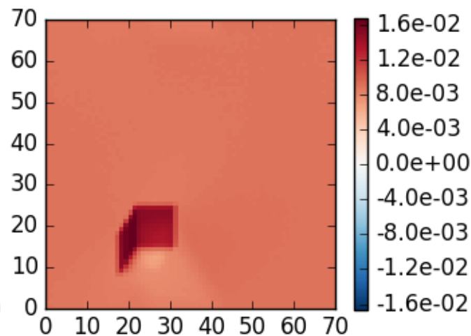
mscart_fmc case 7, \theta_0=40 , z=5 , \theta=140 , \phi=60
