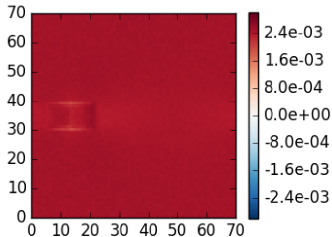
mcart_bmc case 6, \theta_0=40 , z=5 , \theta=140 , \phi=0
