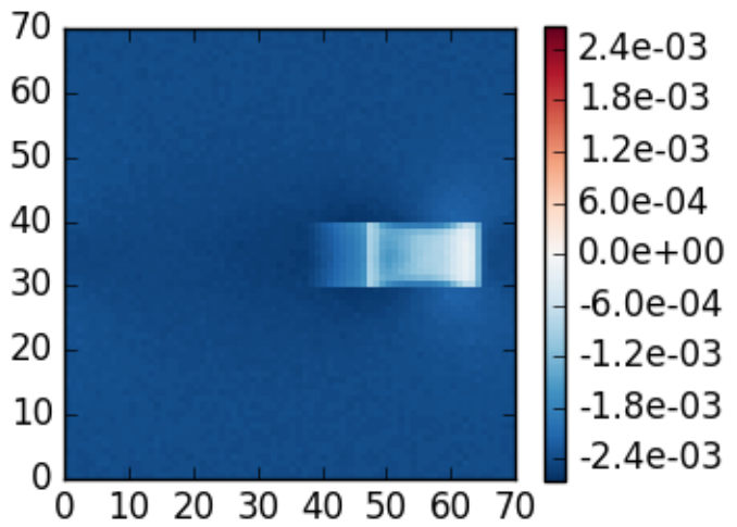
mscart_bmc case 4, \theta_0=20 , z=0 , \theta=40 , \phi=180
