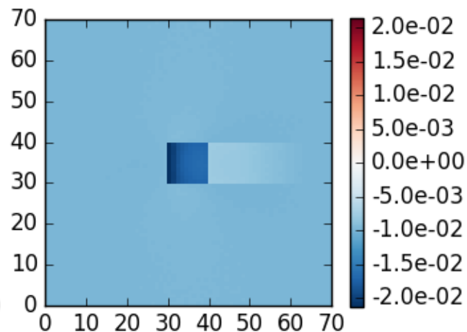
mscart_bmc case 5, \theta_0=40 , z=5 , \theta=180 , \phi=0
