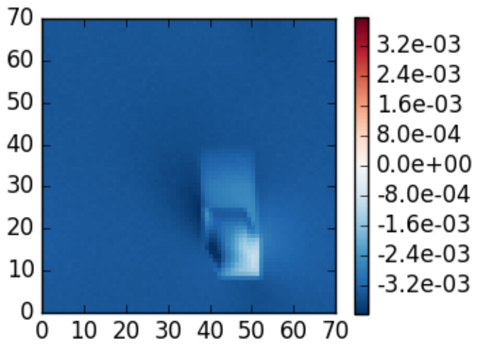
mscart_bmc case 3, \theta_0=20 , z=0 , \theta=40 , \phi=120
