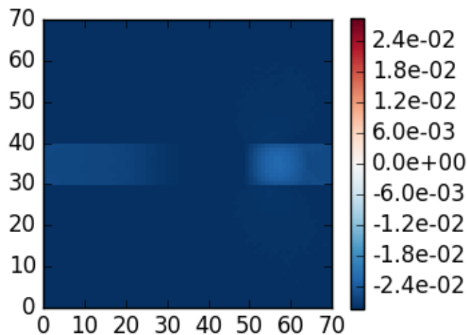
mscart_bmc case 9, \theta_0=40 , z=5 , \theta=140 , \phi=180
