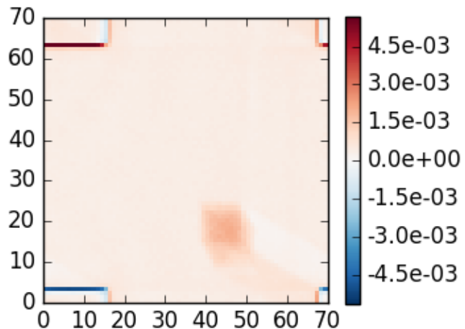
absolute difference case 8, \theta_0=40 , z=5 , \theta=140 , \phi=120
