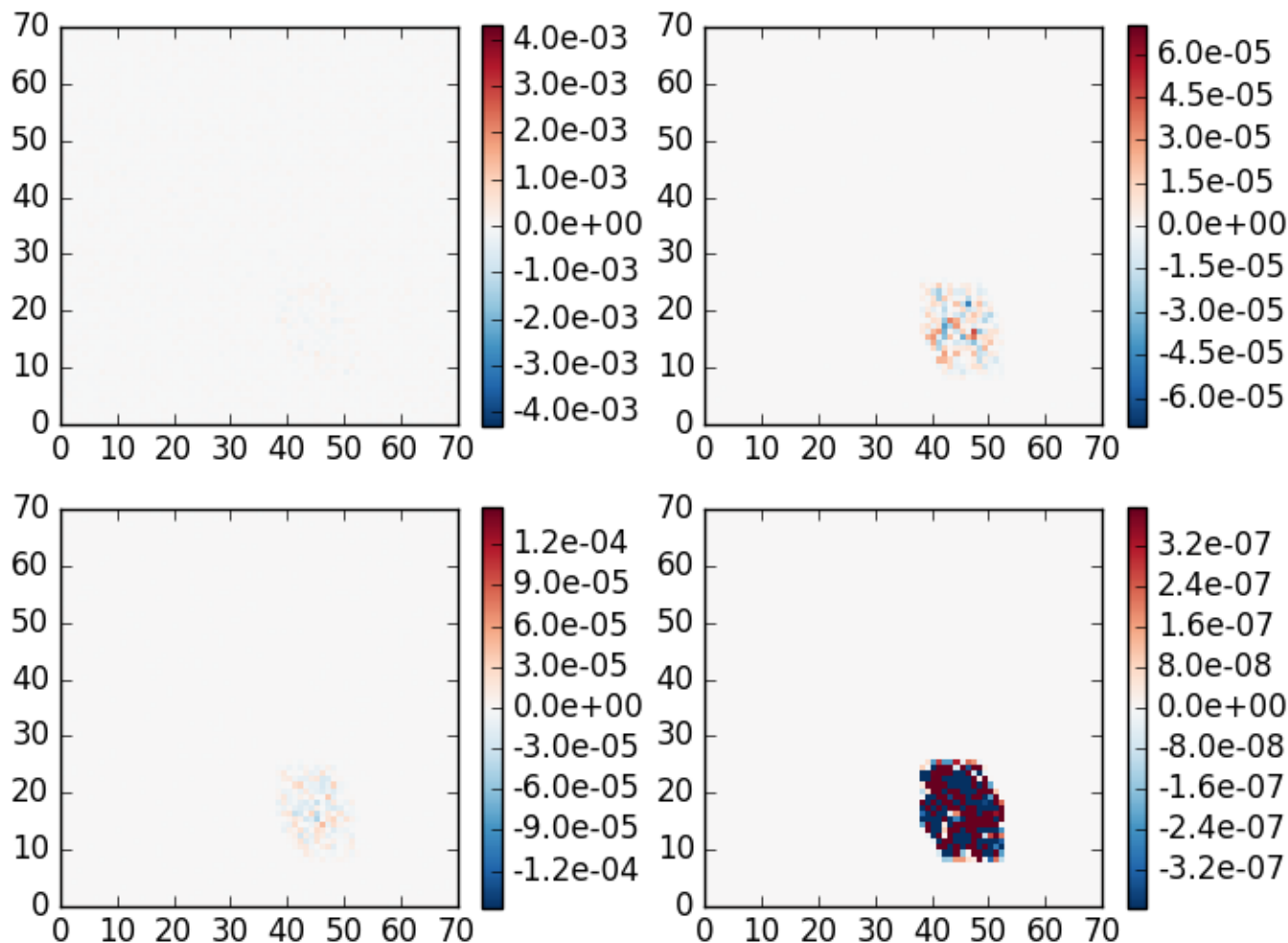
absolute difference case 8, \theta_0=40 , z=5 , \theta=140 , \phi=120
