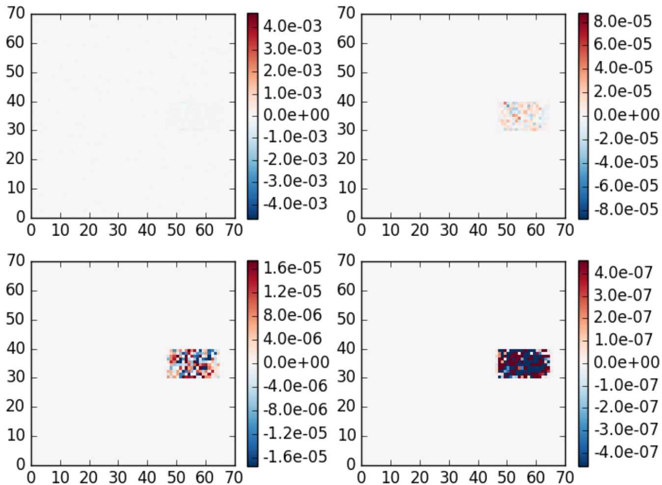
absolute difference case 9, \theta_0=40 , z=5 , \theta=140 , \phi=180
