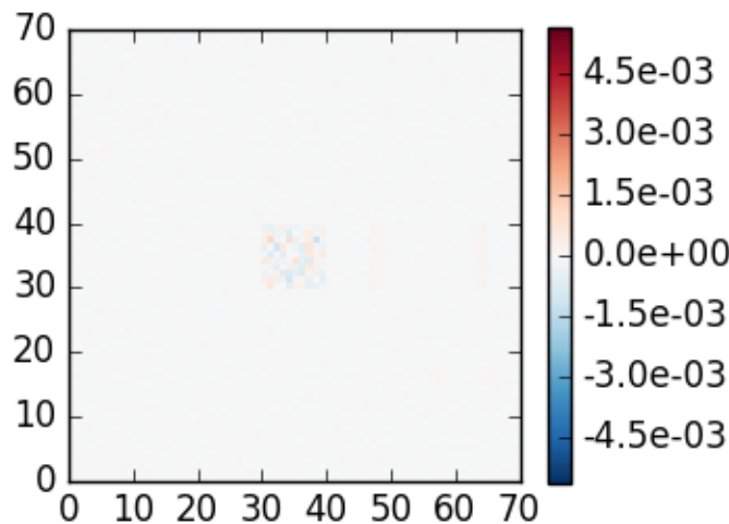
absolute difference case 5, \theta_0=40 , z=5 , \theta=180 , \phi=0
