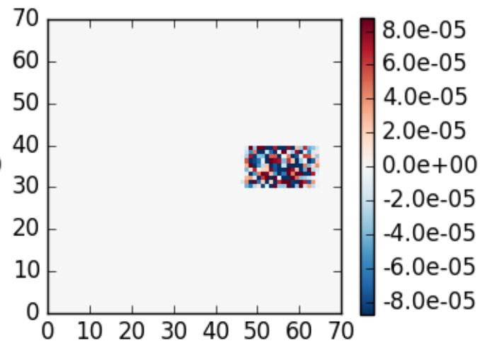
absolute difference case 9, \theta_0=40 , z=5 , \theta=140 , \phi=180
