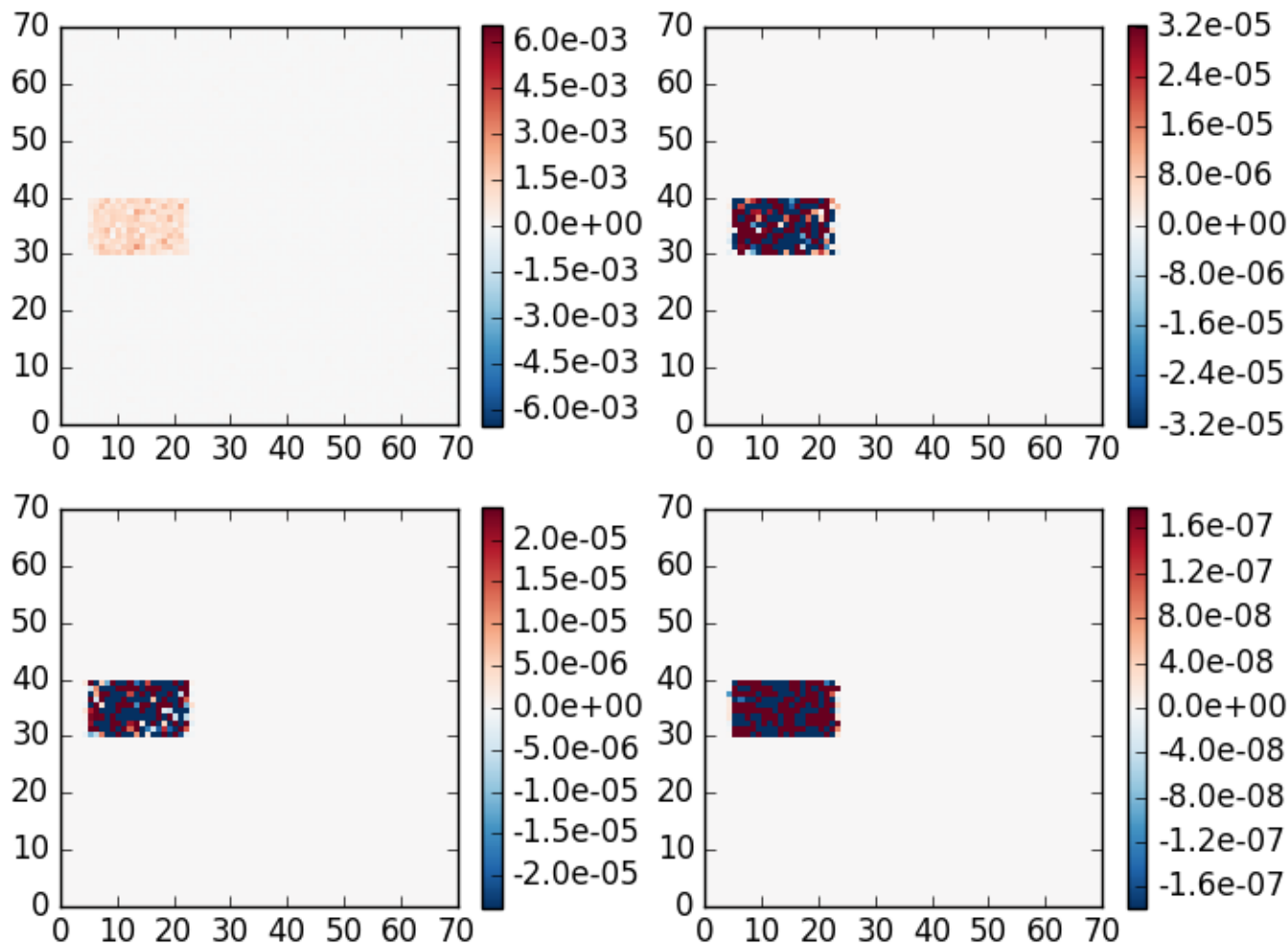
absolute difference case 6, \theta_0=40 , z=5 , \theta=140 , \phi=0
