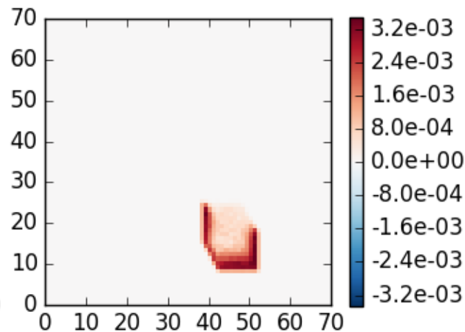
3DMCPOL case 3, \theta_0=20 , z=0 , \theta=40 , \phi=120
