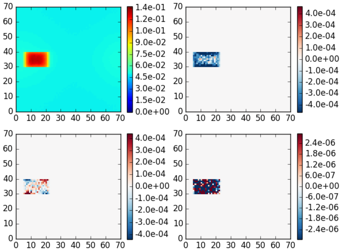
3DMCPOL case 6, \theta_0=40 , z=5 , \theta=140 , \phi=0
