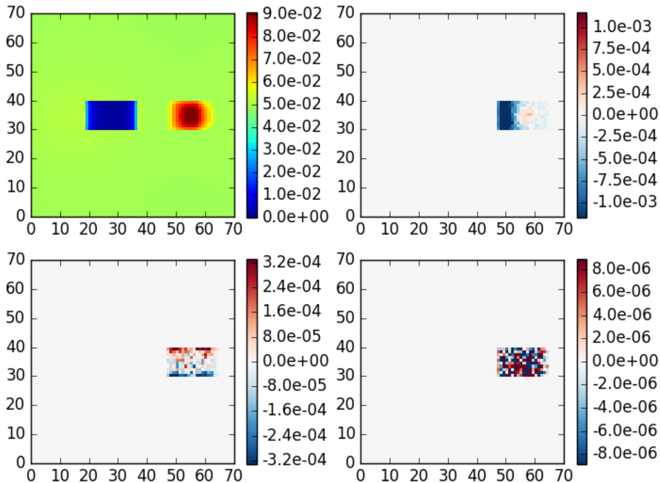
3DMCPOL case 9, \theta_0=40 , z=5 , \theta=140 , \phi=180
