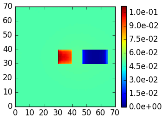
3DMCPOL case 5, \theta_0=40 , z=5 , \theta=180 , \phi=0
