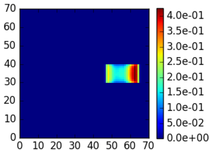
3DMCPOL case 4, \theta_0=20 , z=0 , \theta=40 , \phi=180
