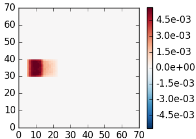
3DMCPOL case 1, \theta_0=20 , z=0 , \theta=40 , \phi=0
