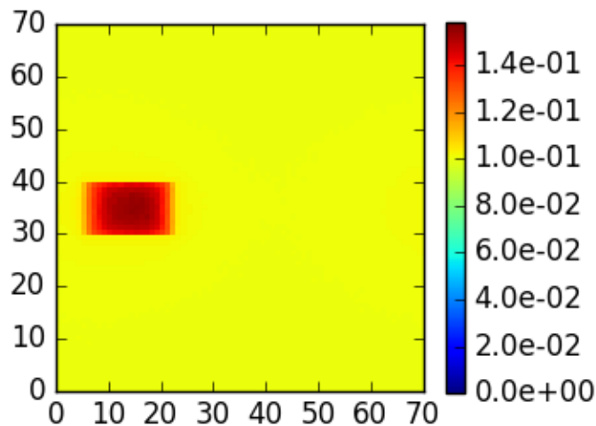
3DMCPOL case 6, \theta_0=40 , z=5 , \theta=140 , \phi=0
