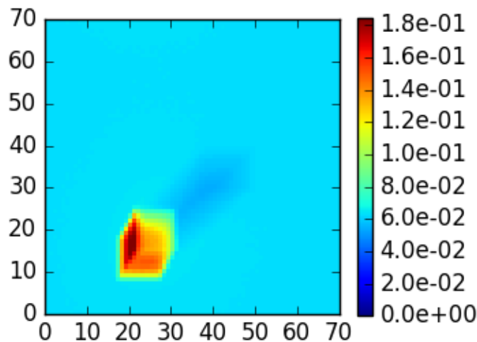
3DMCPOL case 2, \theta_0=20 , z=0 , \theta=40 , \phi=60
