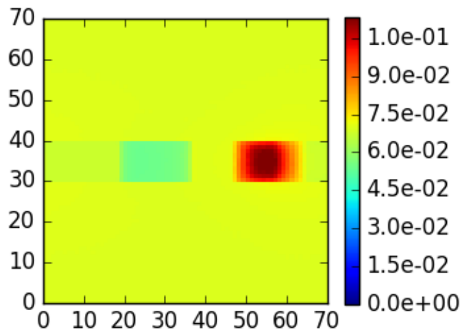
3DMCPOL case 9, \theta_0=40 , z=5 , \theta=140 , \phi=180
