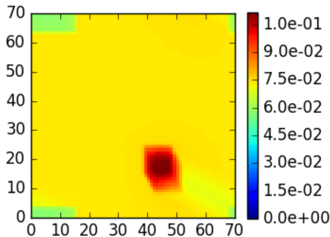
3DMCPOL case 8, \theta_0=40 , z=5 , \theta=140 , \phi=120
