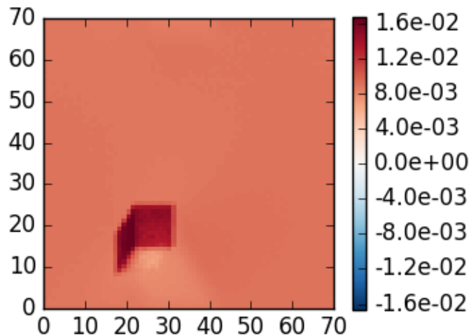
3DMCPOL case 7, \theta_0=40 , z=5 , \theta=140 , \phi=60
