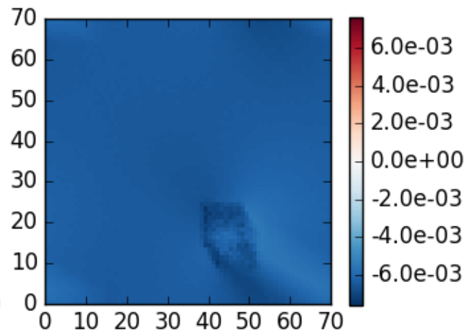
3DMCPOL case 8, \theta_0=40 , z=5 , \theta=140 , \phi=120
