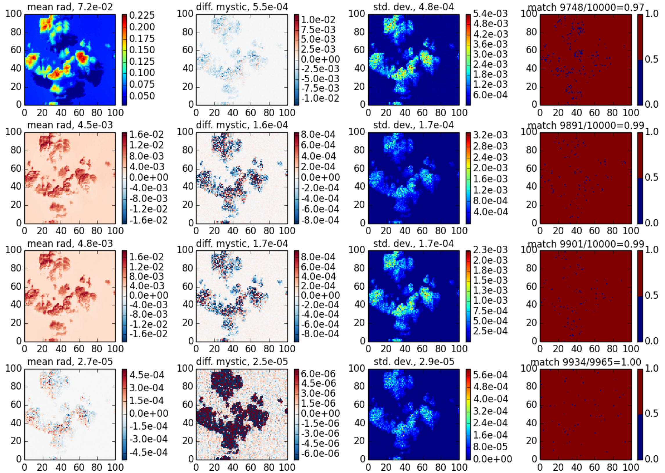
SPARTA case 7, \theta_0=40 , z=30 , \theta=140 , \phi=60
