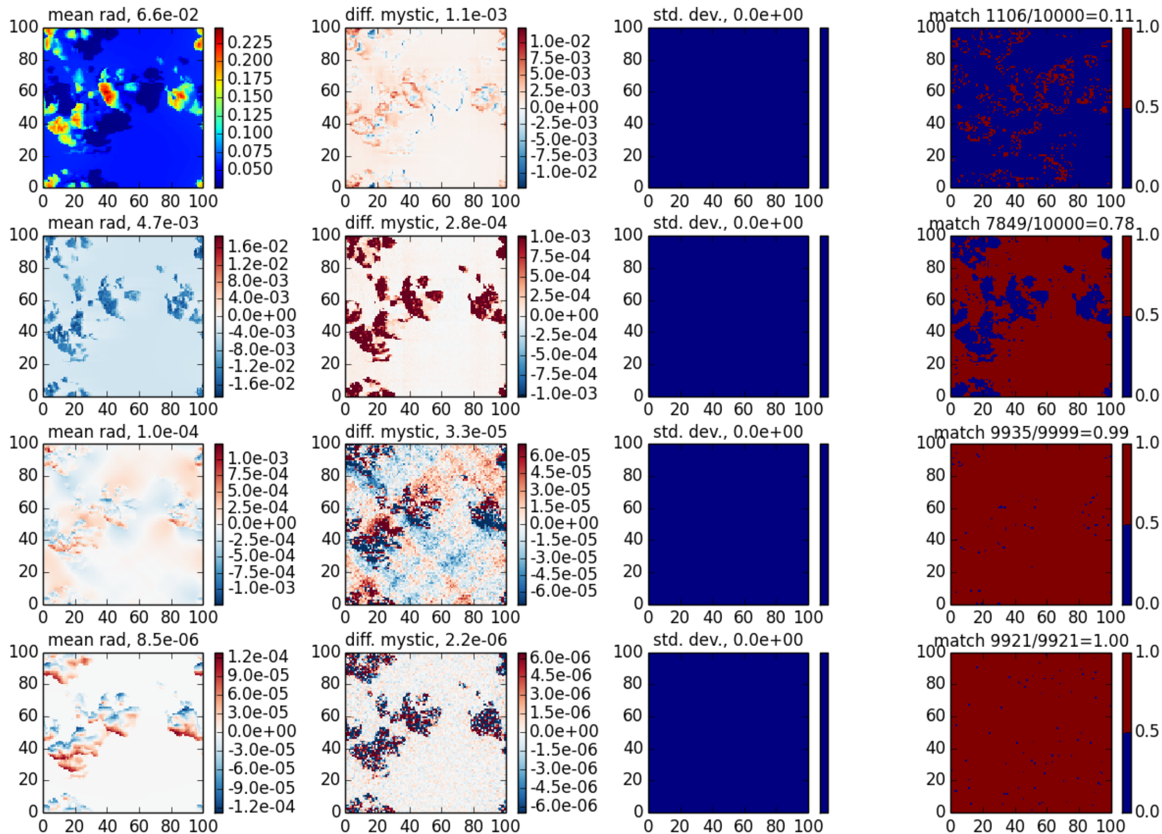
shdom3 case 5, \theta_0=40 , z=30 , \theta=180 , \phi=0
