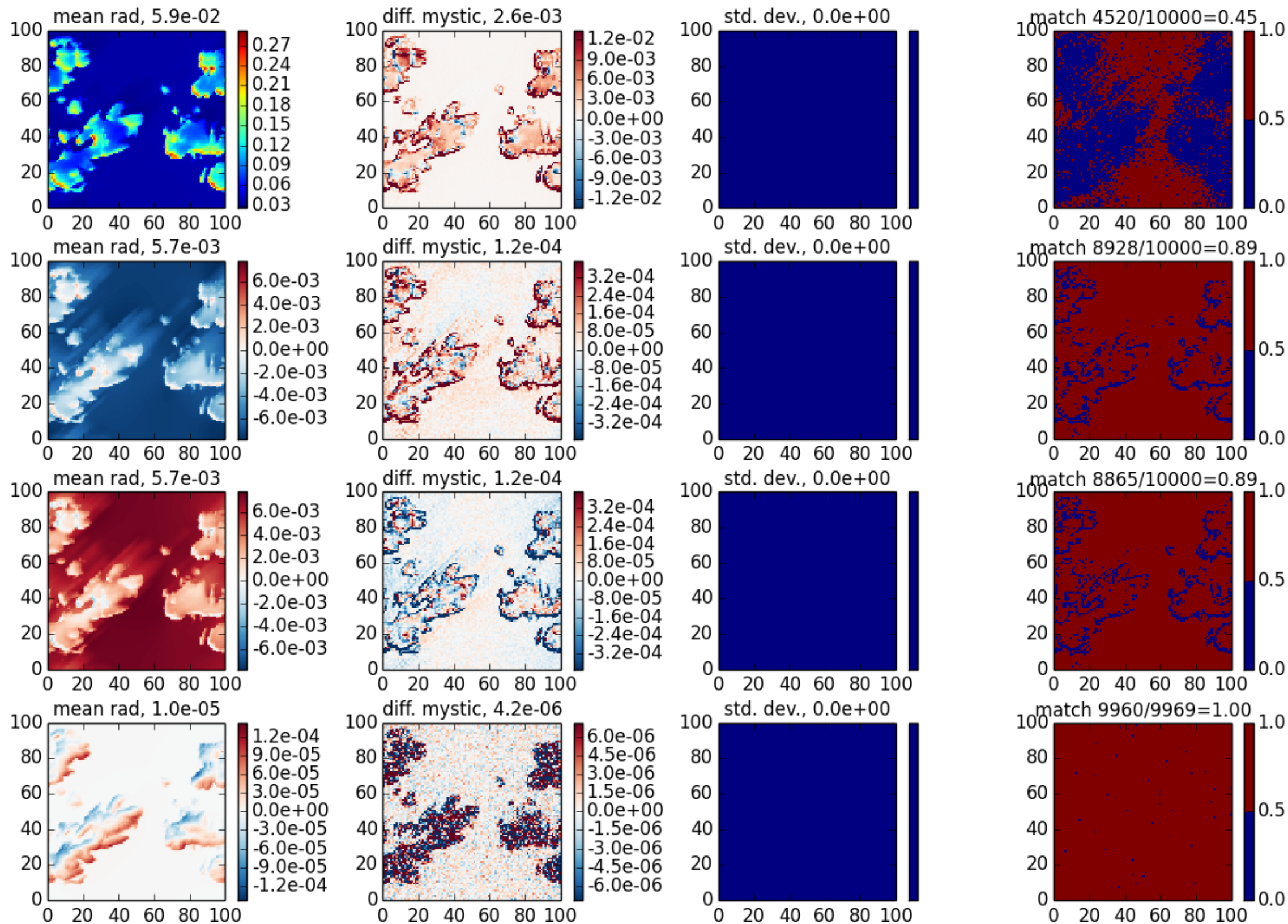
shdom3 case 2, \theta_0=20 , z=0 , \theta=40 , \phi=60
