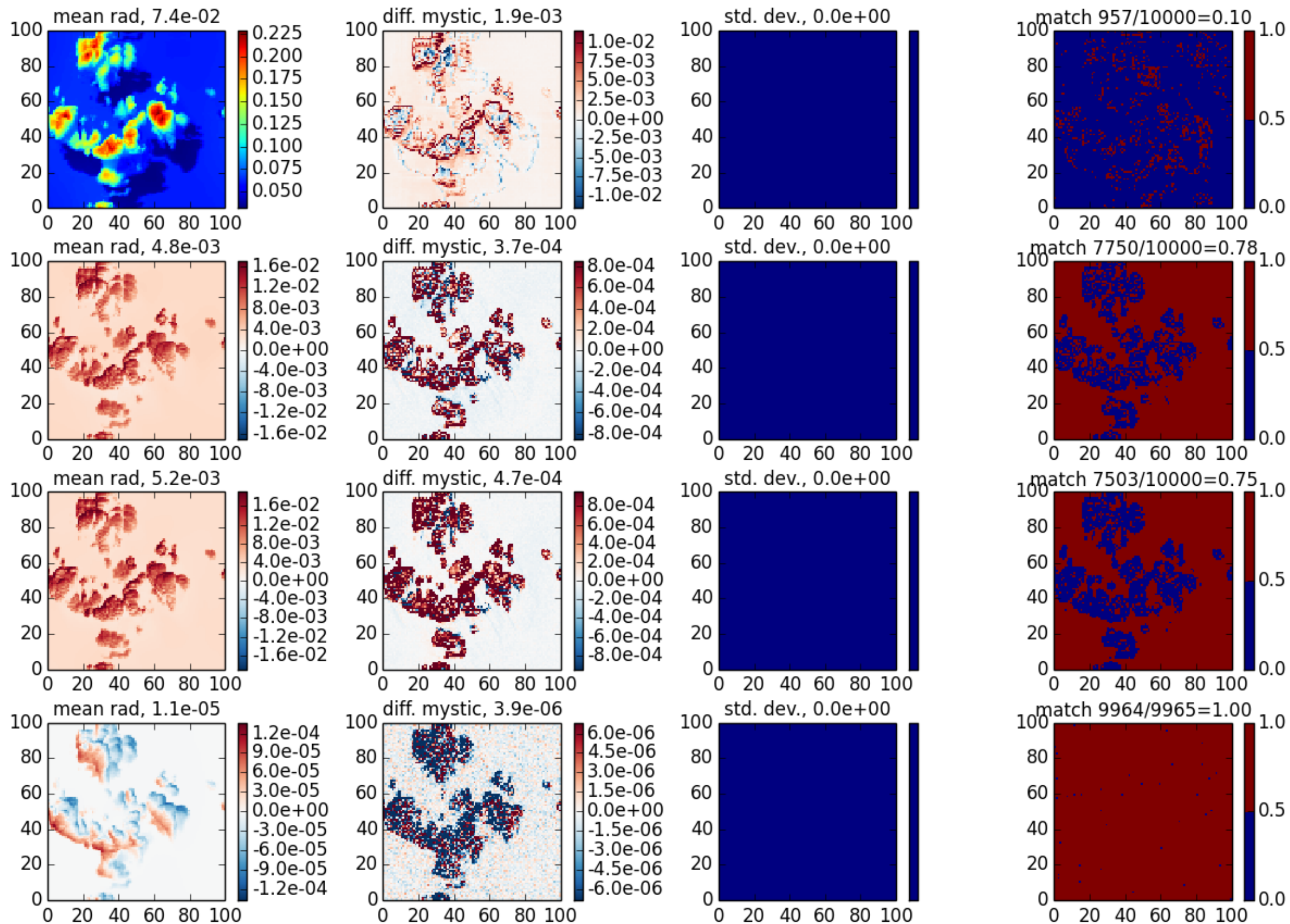
shdom3 case 7, \theta_0=40 , z=30 , \theta=140 , \phi=60
