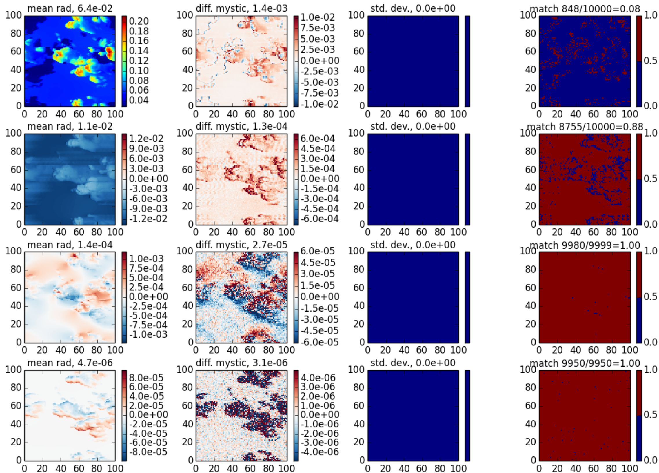
shdom3 case 9, \theta_0=40 , z=30 , \theta=140 , \phi=180
