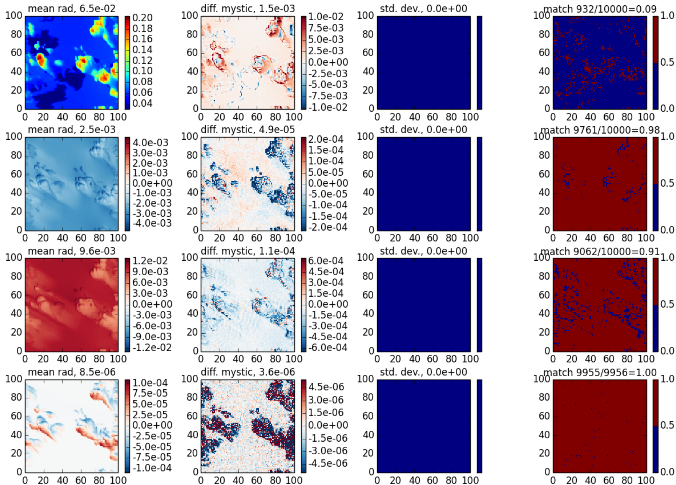
shdom3 case 8, \theta_0=40 , z=30 , \theta=140 , \phi=120
