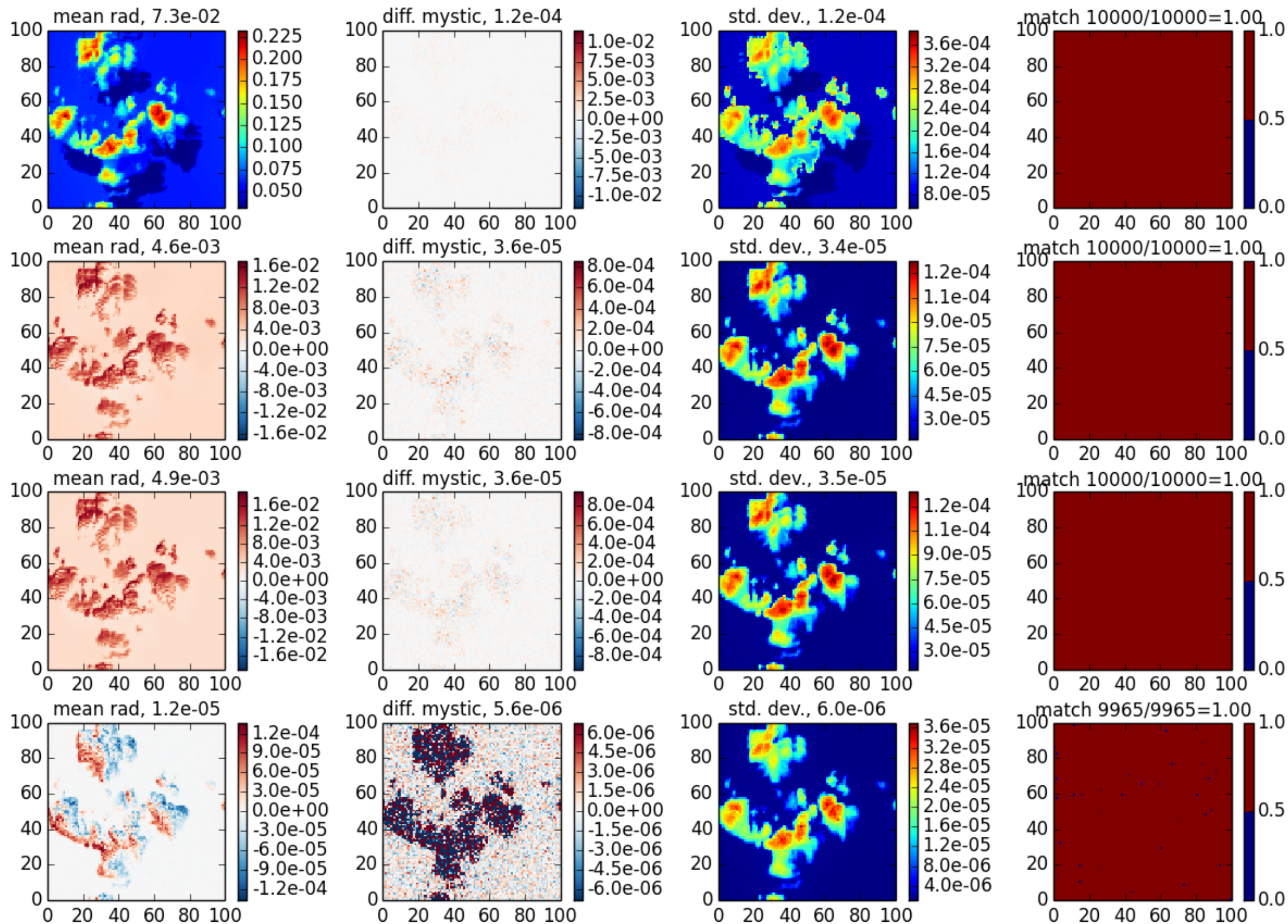
mscart_fmc case 7, \theta_0=40 , z=30 , \theta=140 , \phi=60
