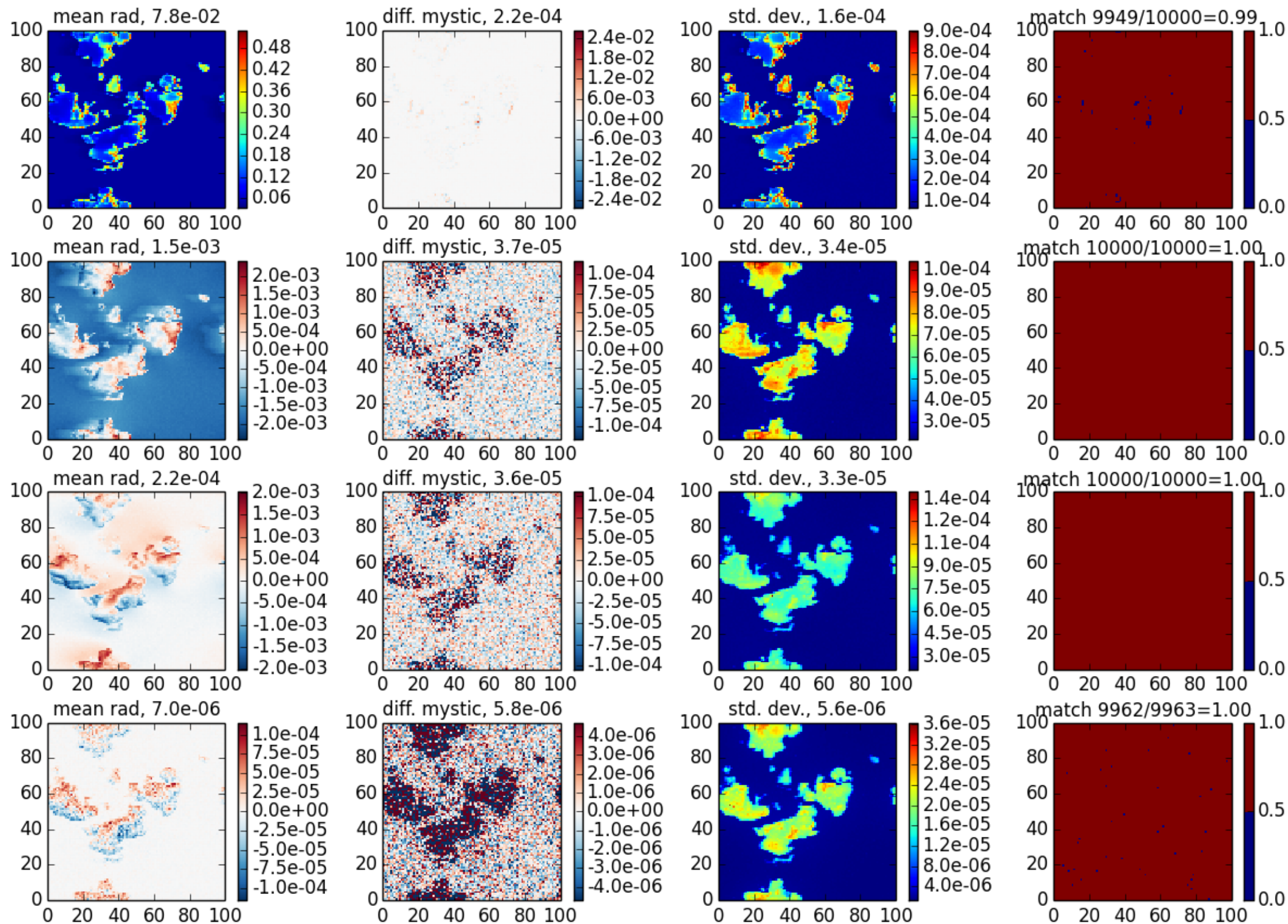
mscart_fmc case 4, \theta_0=20 , z=0 , \theta=40 , \phi=180
