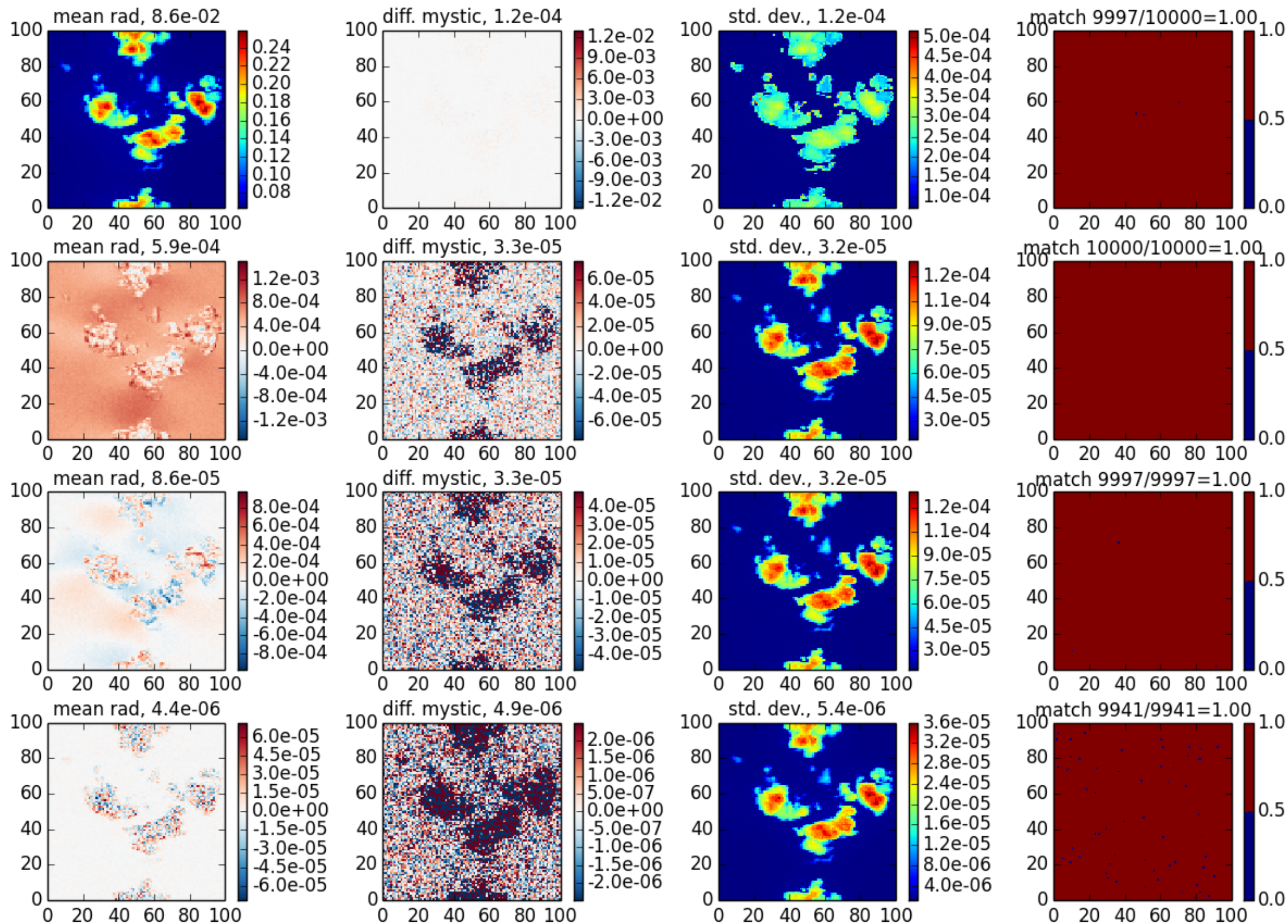
mscart_fmc case 6, \theta_0=40 , z=30 , \theta=140 , \phi=0
