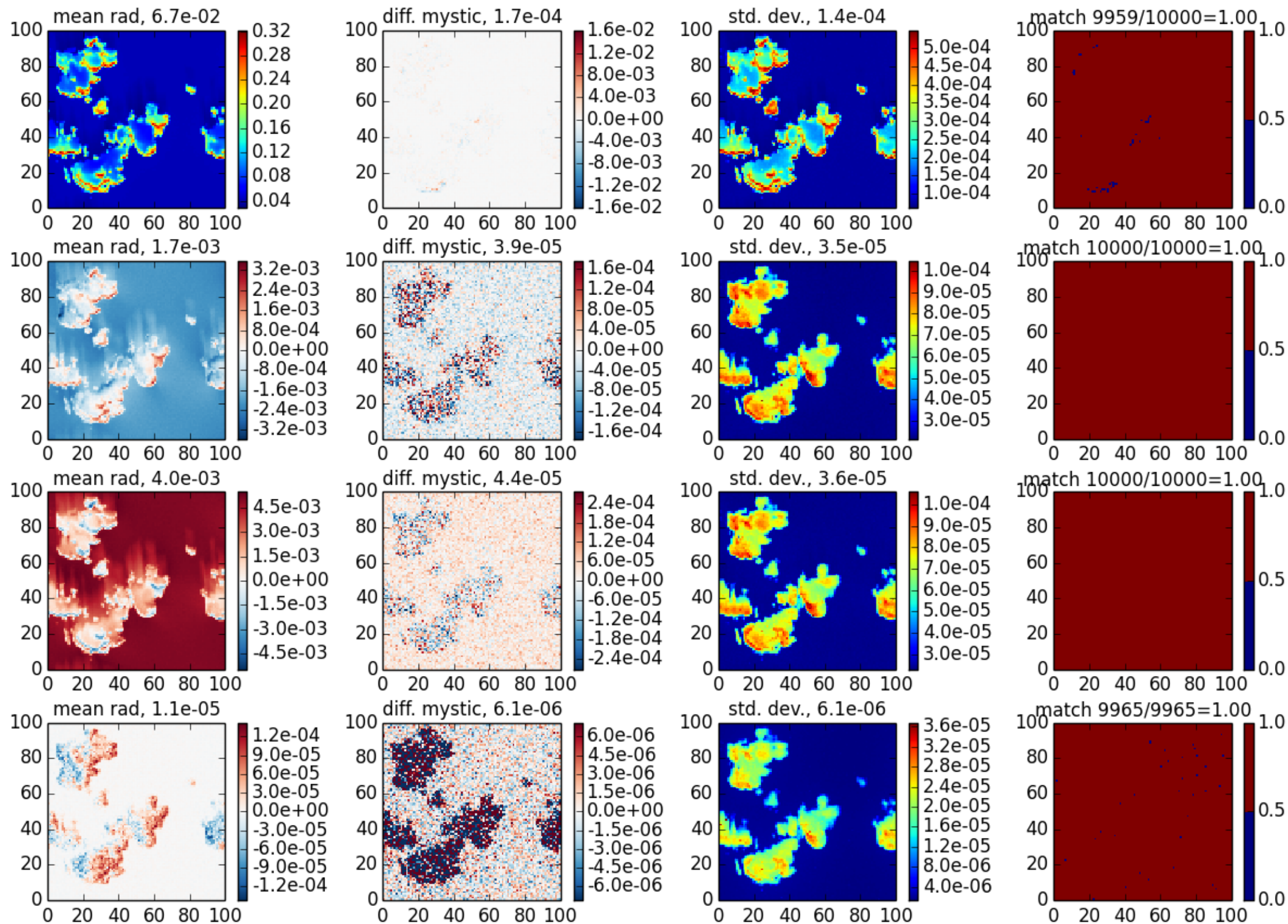
mscart_fmc case 3, \theta_0=20 , z=0 , \theta=40 , \phi=120
