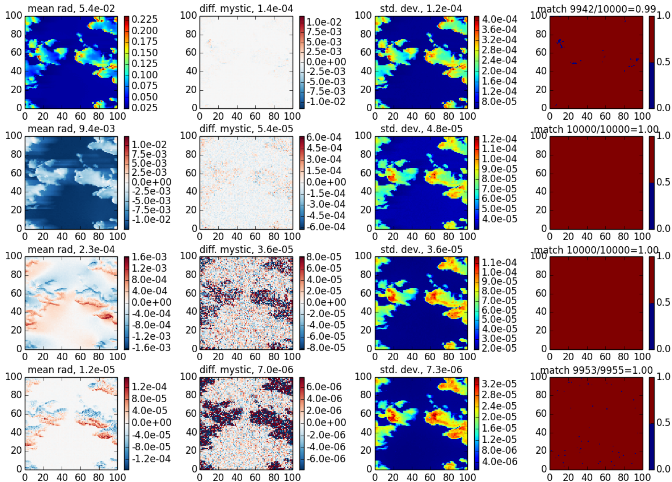
mscart_fmc case 1, \theta_0=20 , z=0 , \theta=40 , \phi=0
