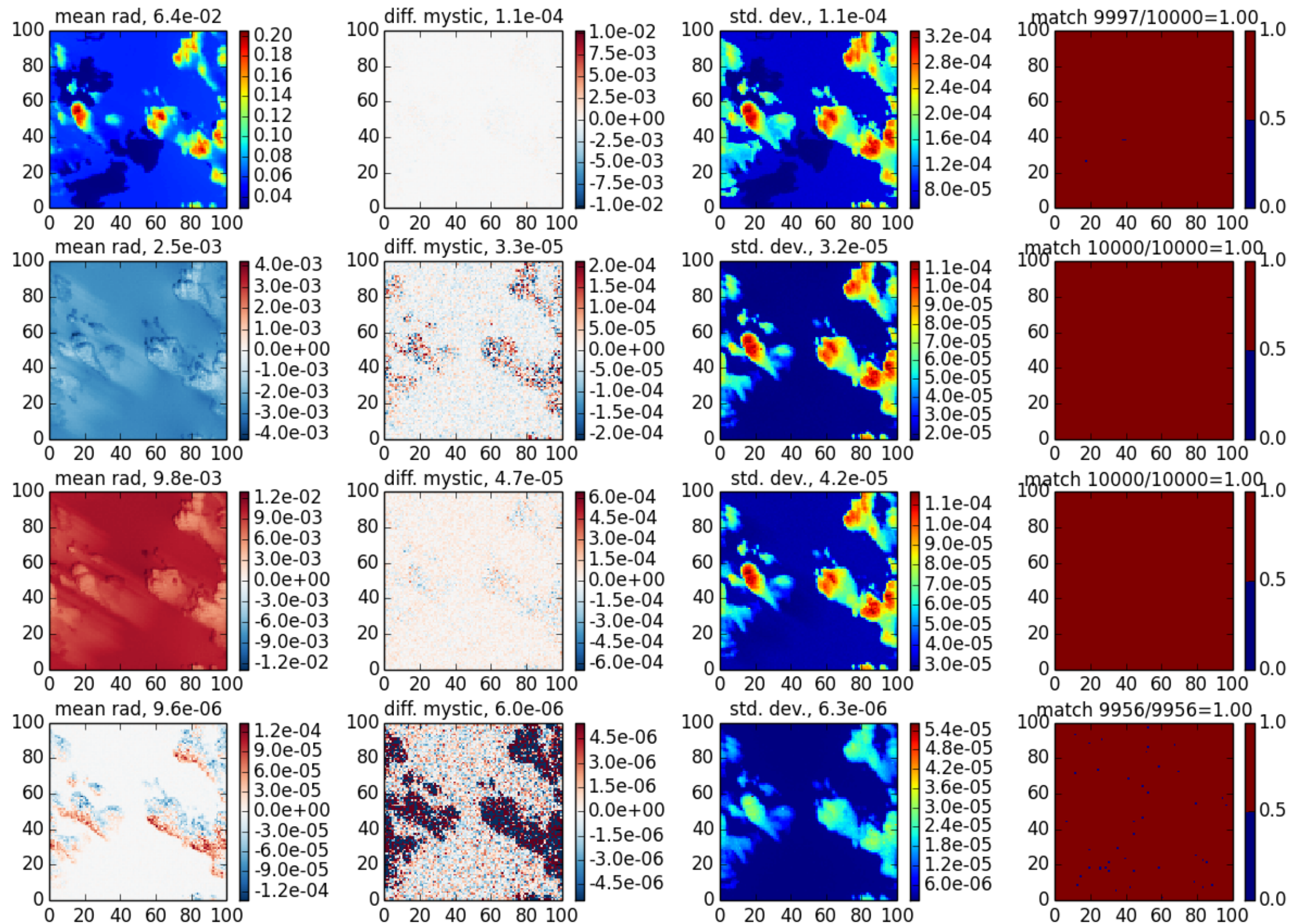
mscart_fmc case 8, \theta_0=40 , z=30 , \theta=140 , \phi=120
