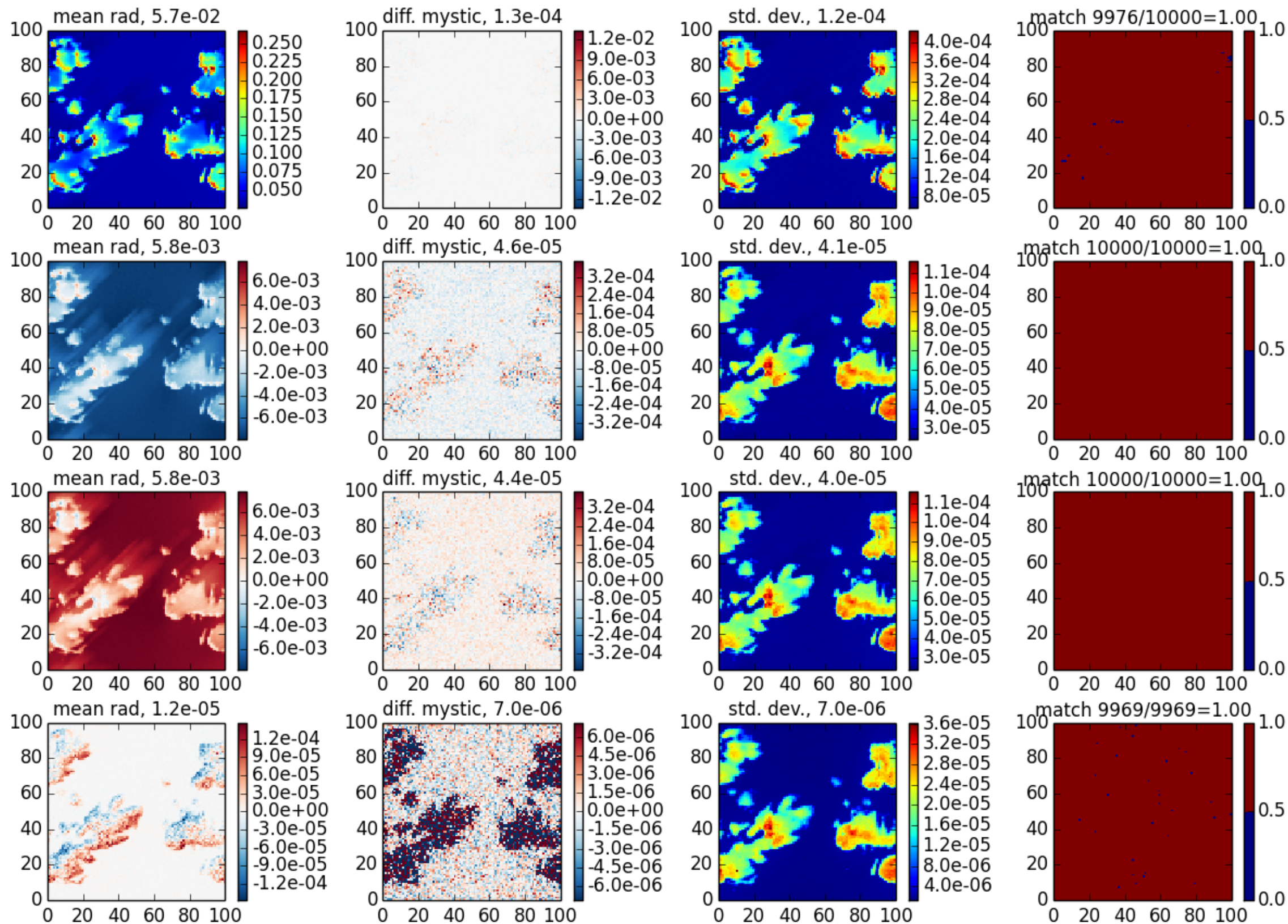
mscart_fmc case 2, \theta_0=20 , z=0 , \theta=40 , \phi=60
