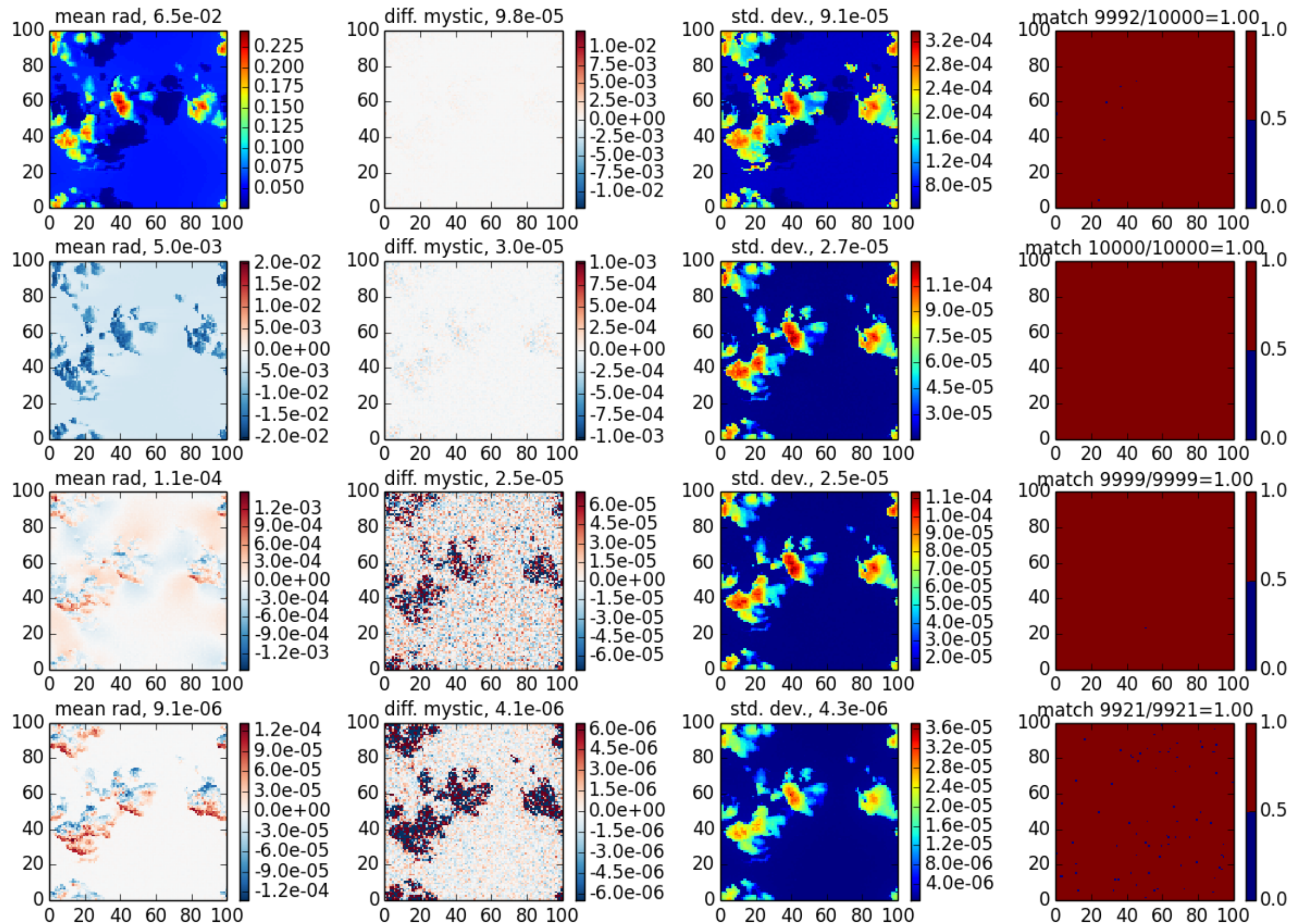
mscart_fmc case 5, \theta_0=40 , z=30 , \theta=180 , \phi=0
