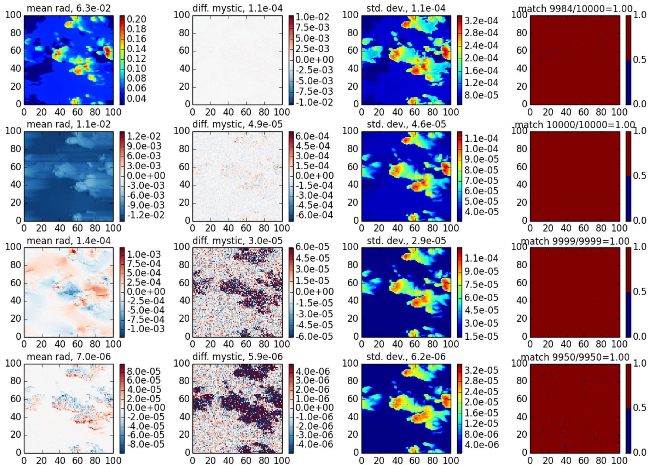
mscart_fmc case 9, \theta_0=40 , z=30 , \theta=140 , \phi=180
