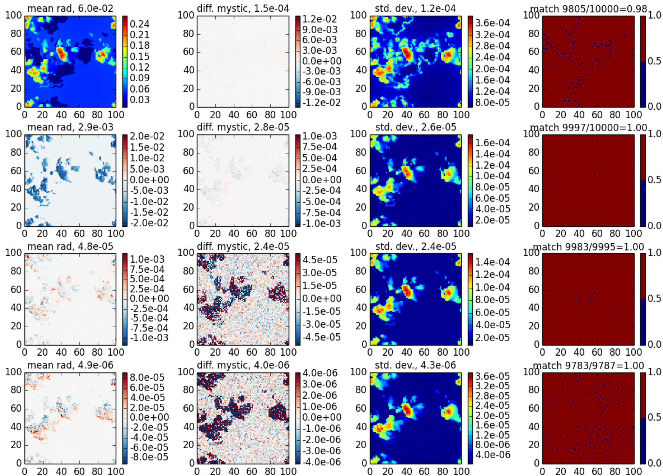
mscart_bmc case 5, \theta_0=40 , z=30 , \theta=180 , \phi=0
