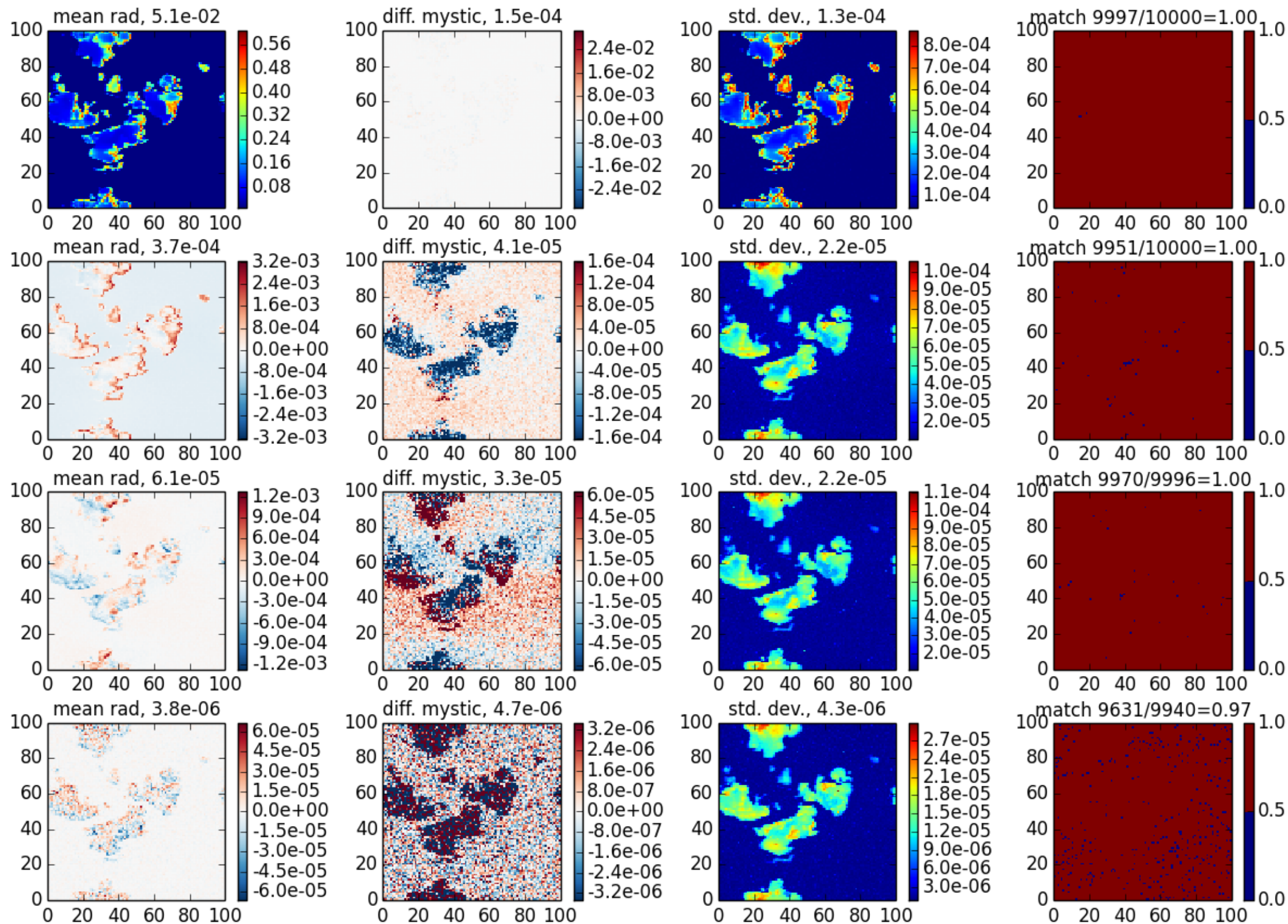
mscart_bmc case 4, \theta_0=20 , z=0 , \theta=40 , \phi=180
