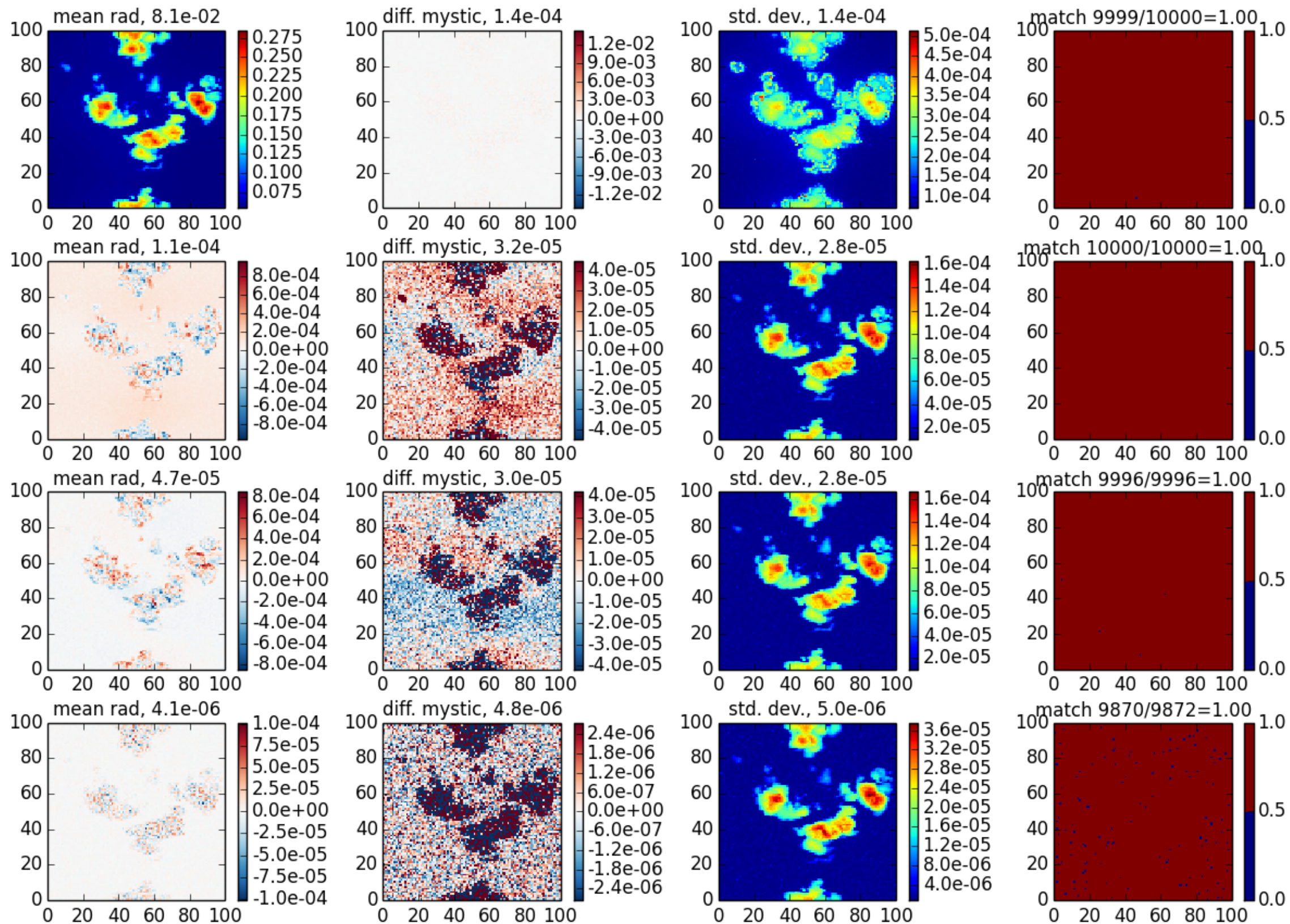
mscart_bmc case 6, \theta_0=40 , z=30 , \theta=140 , \phi=0
