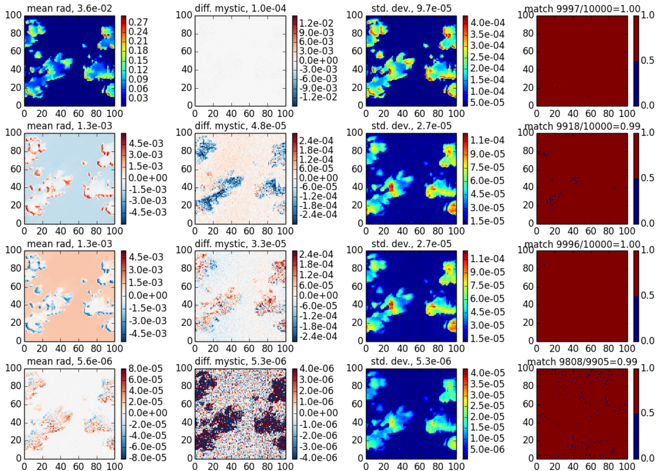
mscart_bmc case 2, \theta_0=20 , z=0 , \theta=40 , \phi=60
