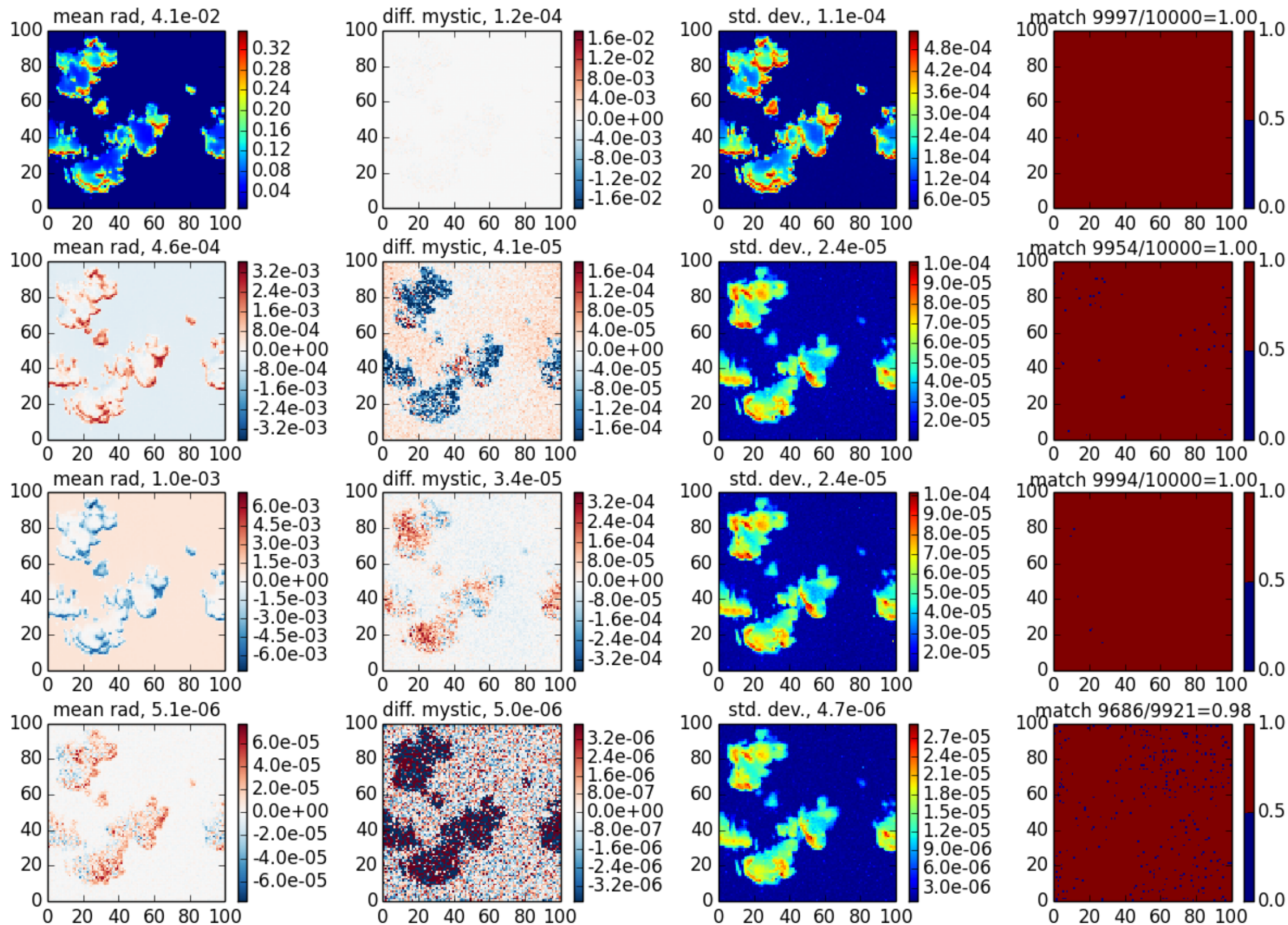
mscart_bmc case 3, \theta_0=20 , z=0 , \theta=40 , \phi=120
