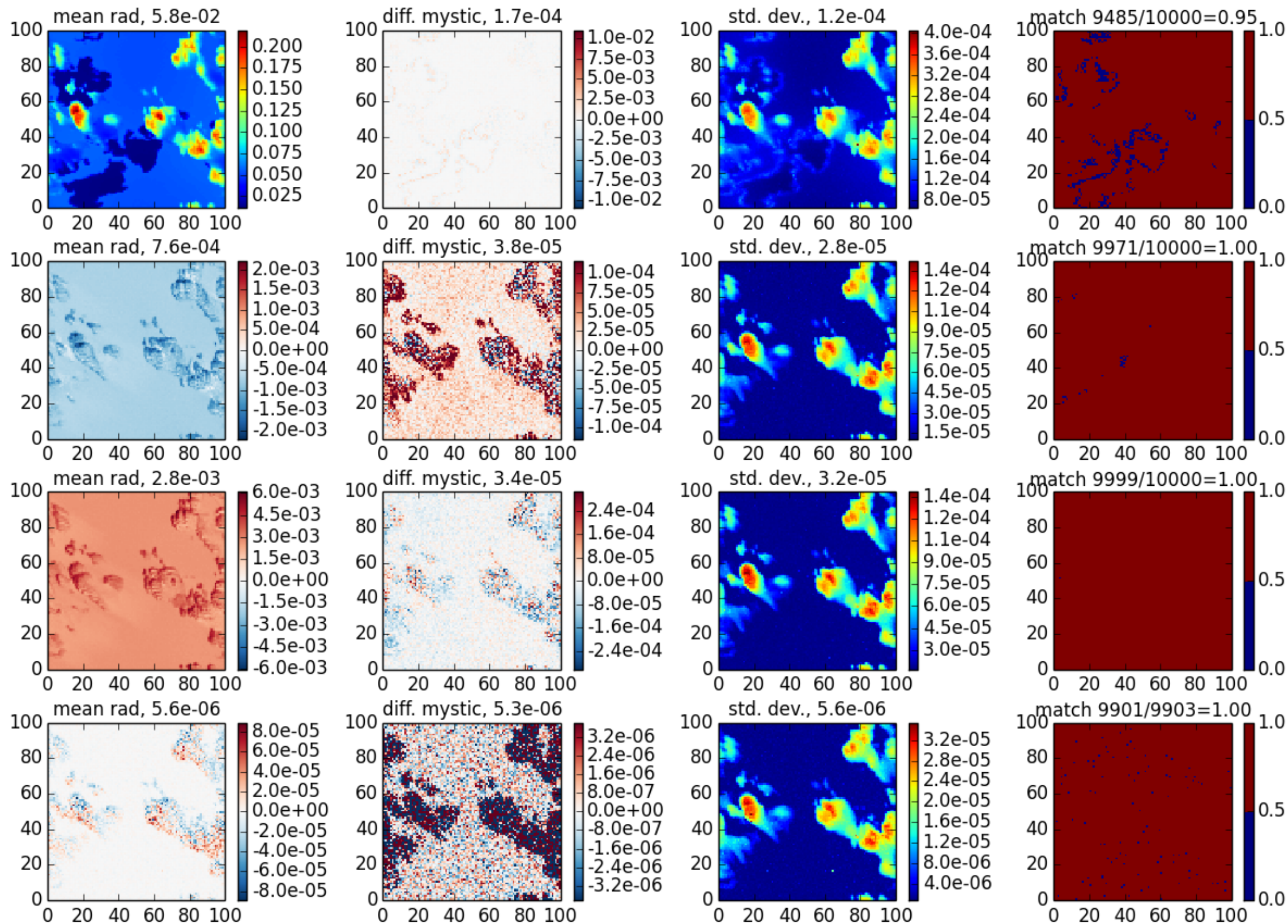
mscart_bmc case 8, \theta_0=40 , z=30 , \theta=140 , \phi=120
