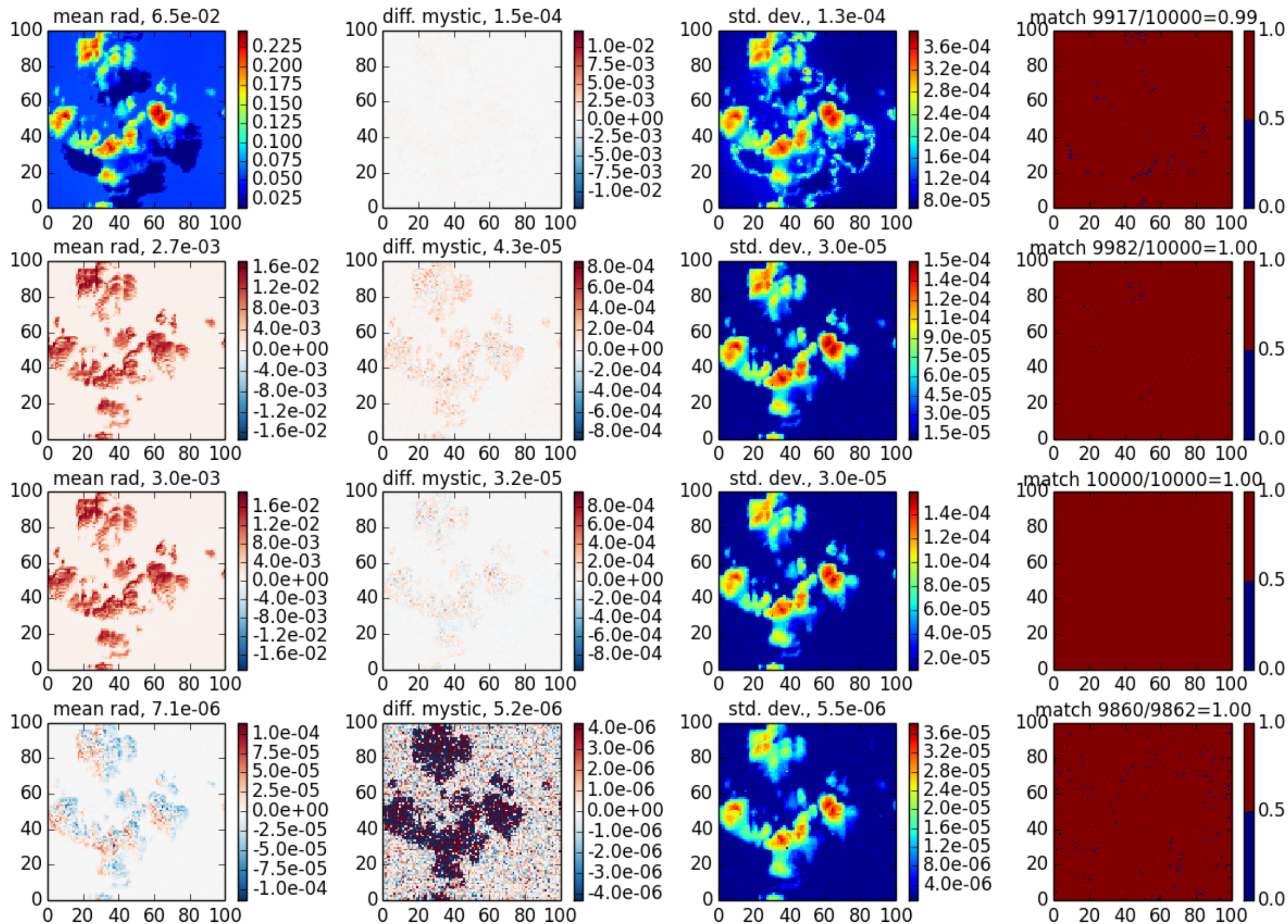
mscart_bmc case 7, \theta_0=40 , z=30 , \theta=140 , \phi=60
