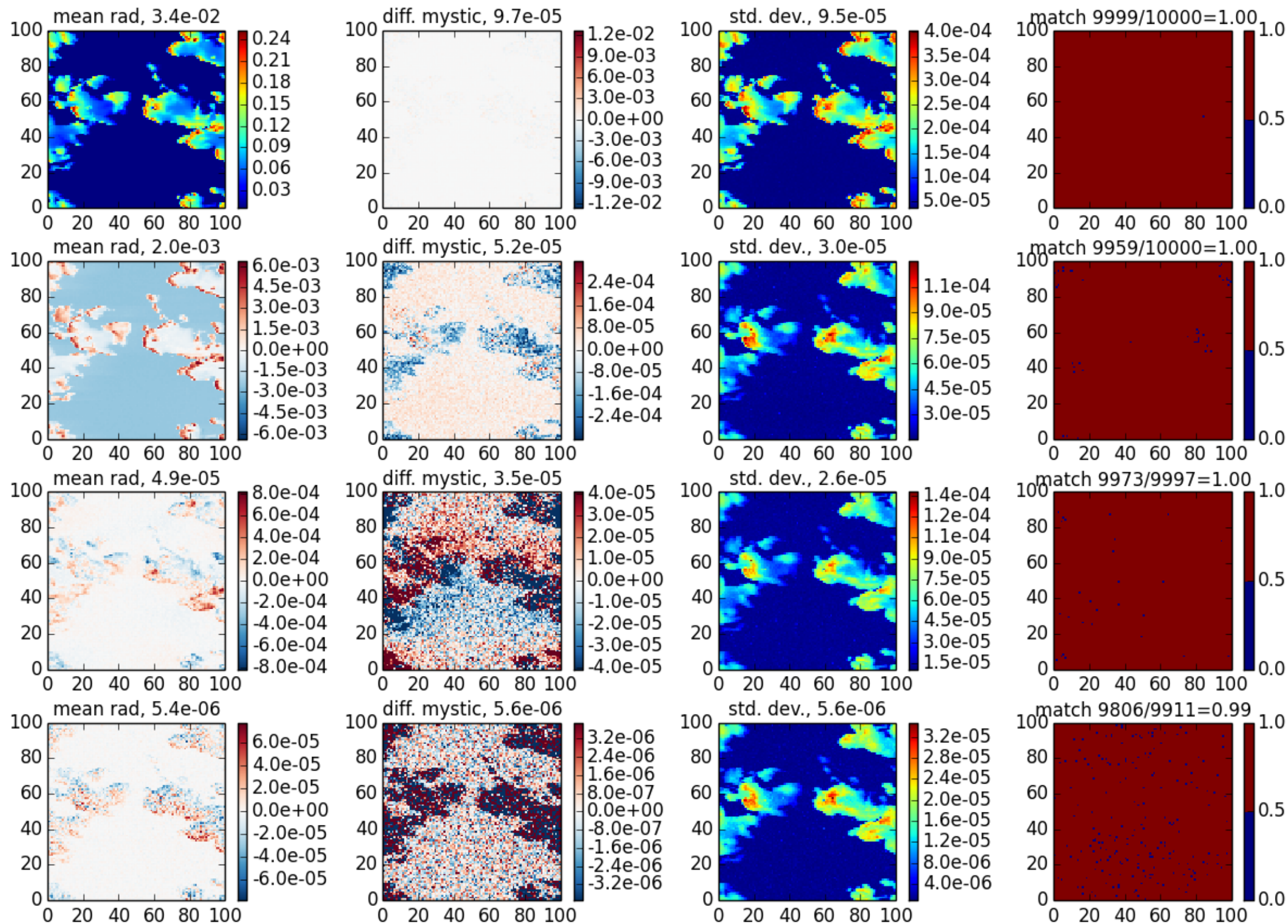
mcart_bmc case 1, \theta_0=20 , z=0 , \theta=40 , \phi=0
