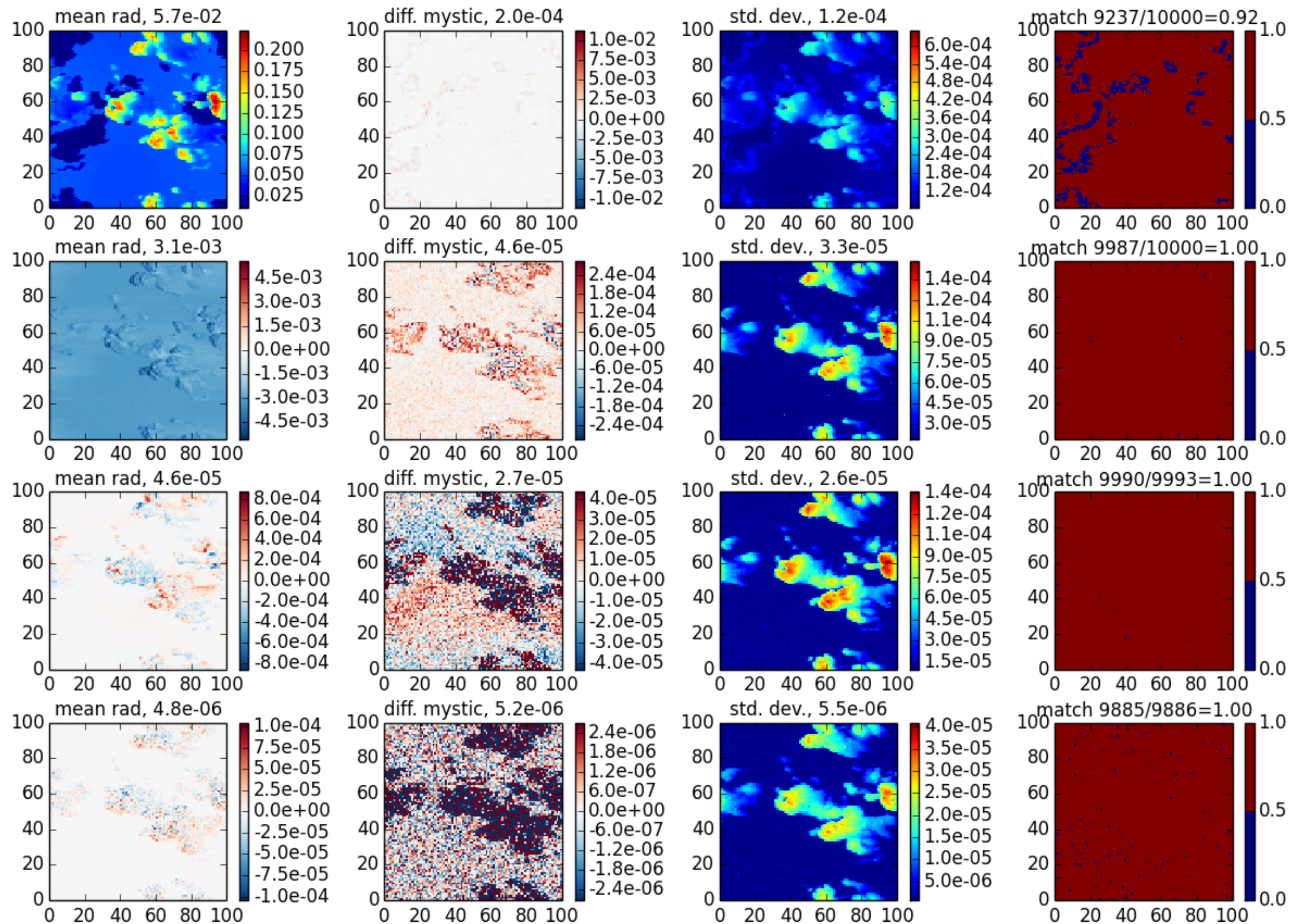
mscart_bmc case 9, \theta_0=40 , z=30 , \theta=140 , \phi=180
