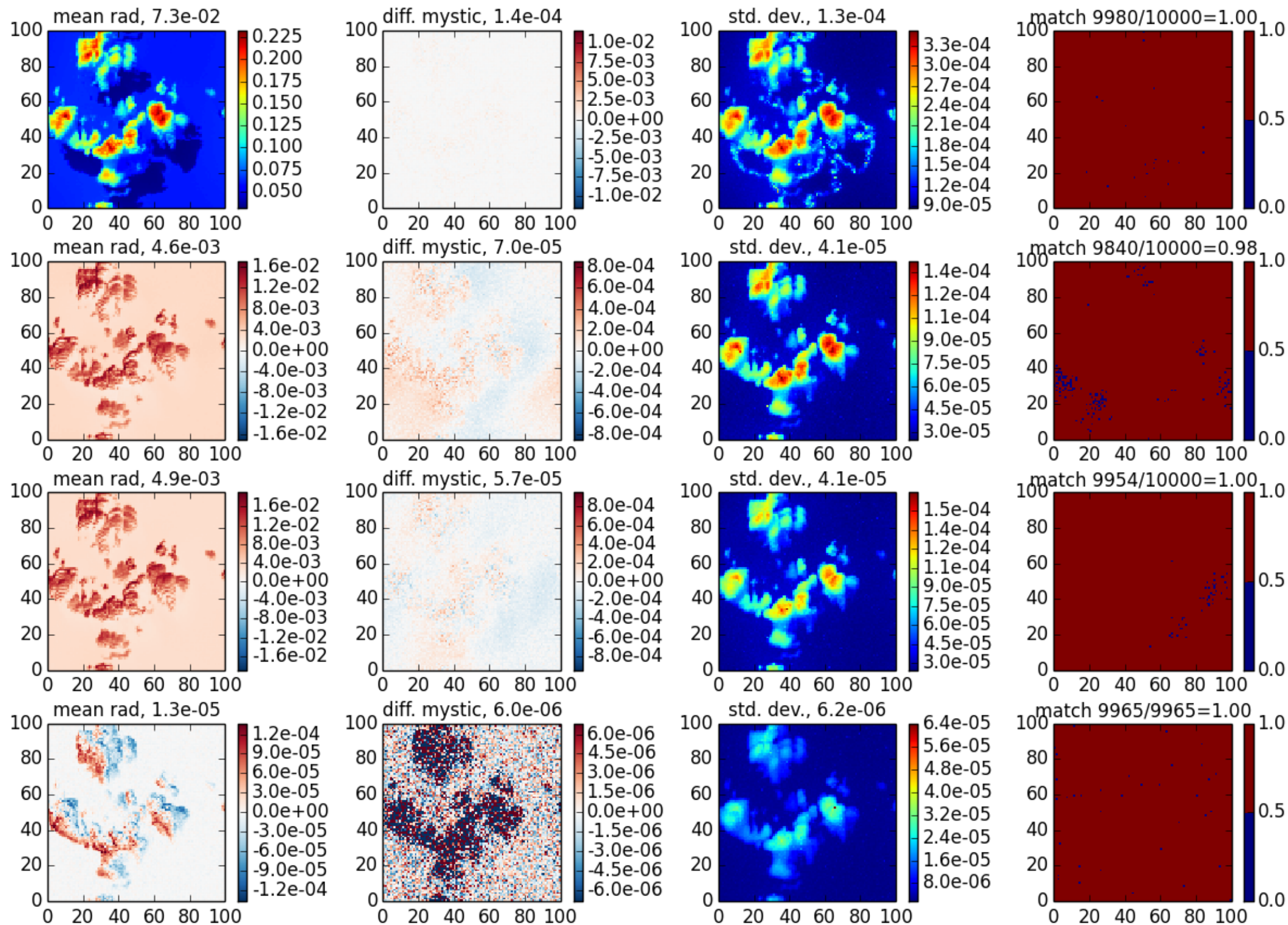
mcart_bmc case 7, \theta_0=40 , z=30 , \theta=140 , \phi=60
