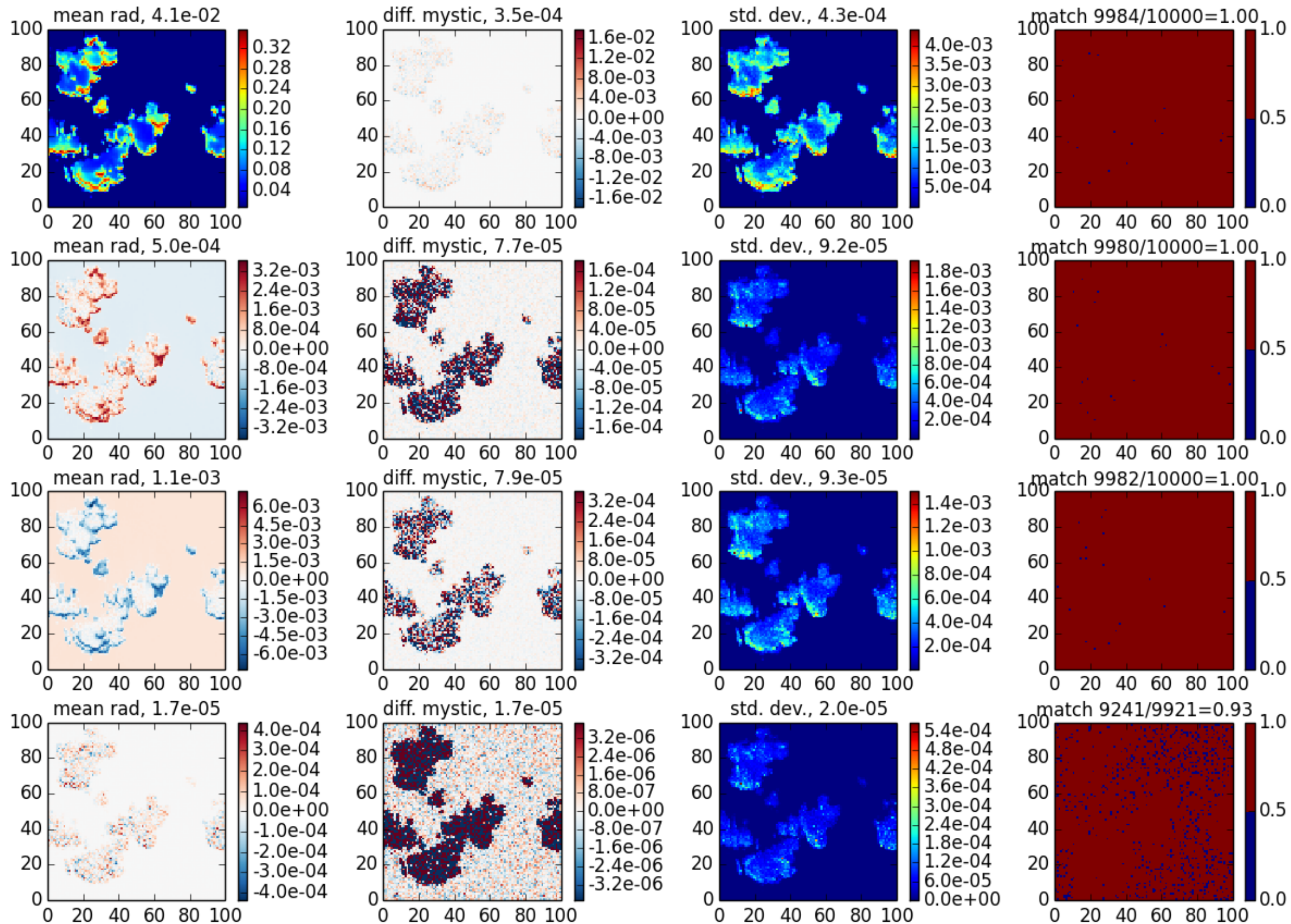
3DMCPOL case 3, \theta_0=20 , z=0 , \theta=40 , \phi=120
