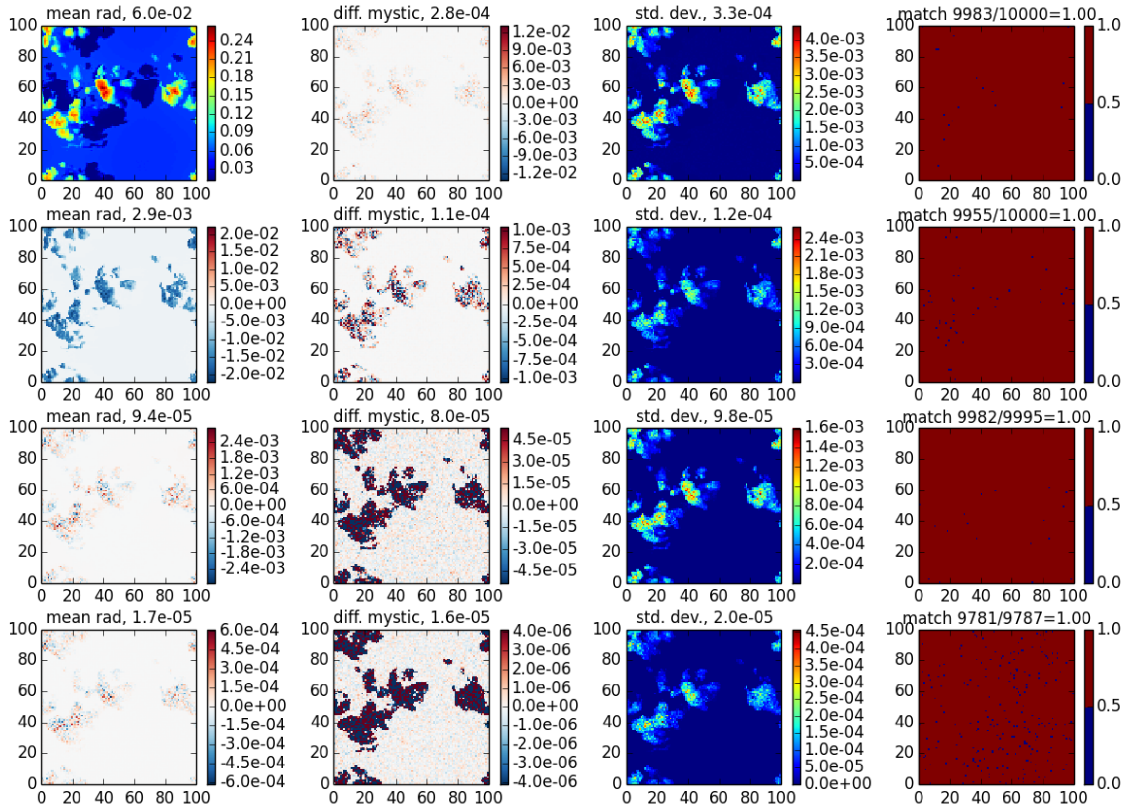
3DMCPOL case 5, \theta_0=40 , z=30 , \theta=180 , \phi=0
