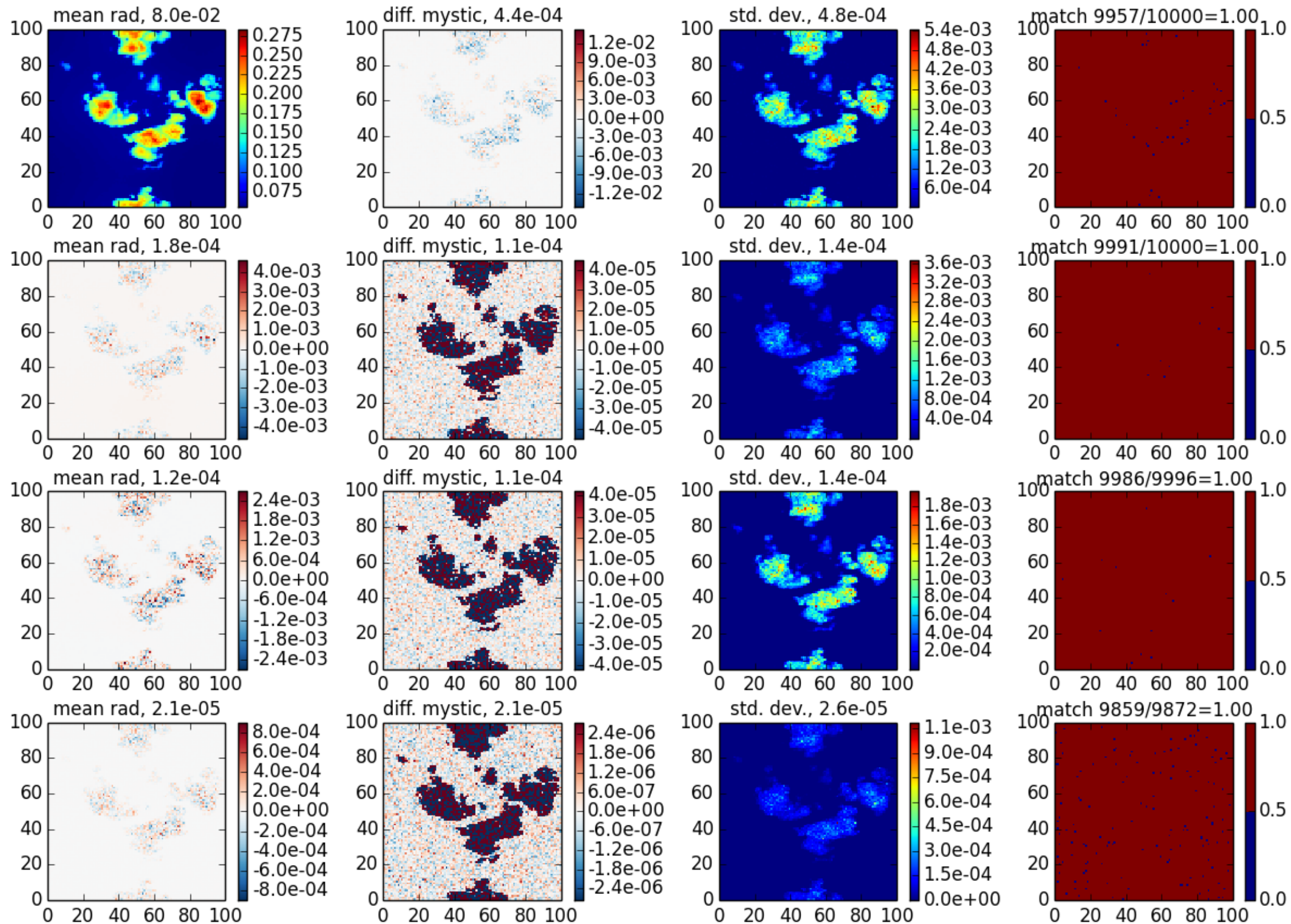
3DMCPOL case 6, \theta_0=40 , z=30 , \theta=140 , \phi=0
