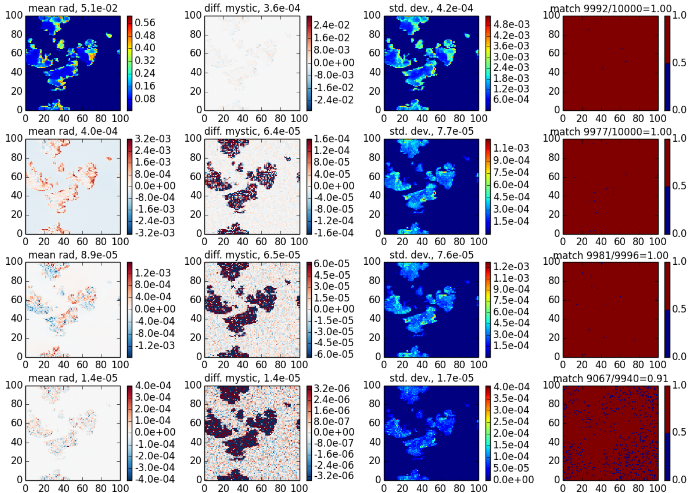
3DMCPOL case 4, \theta_0=20 , z=0 , \theta=40 , \phi=180
