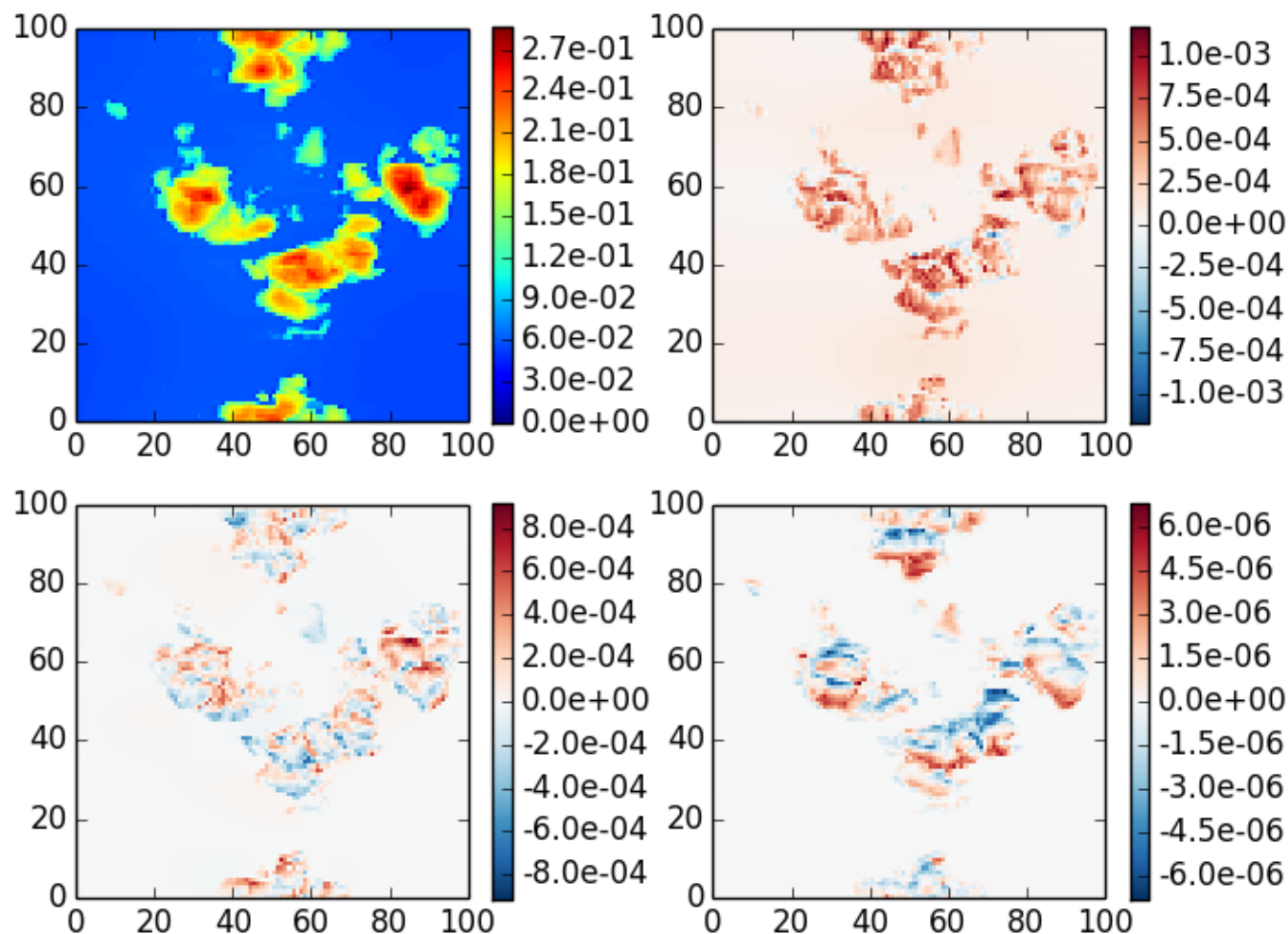
shdom3 case 6, \theta_0=40 , z=30 , \theta=140 , \phi=0
