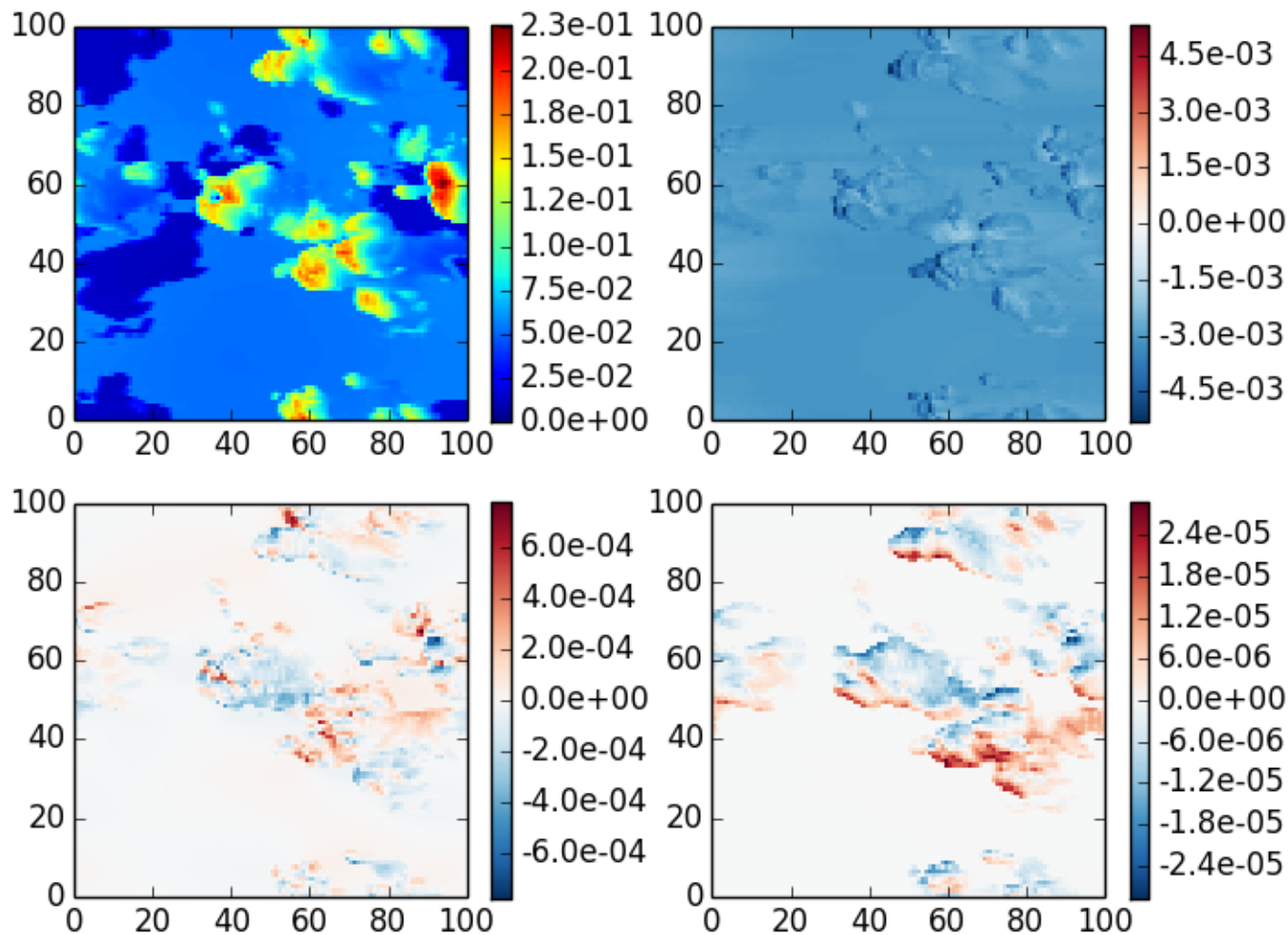
shdom3 case 9, \theta_0=40 , z=30 , \theta=140 , \phi=180
