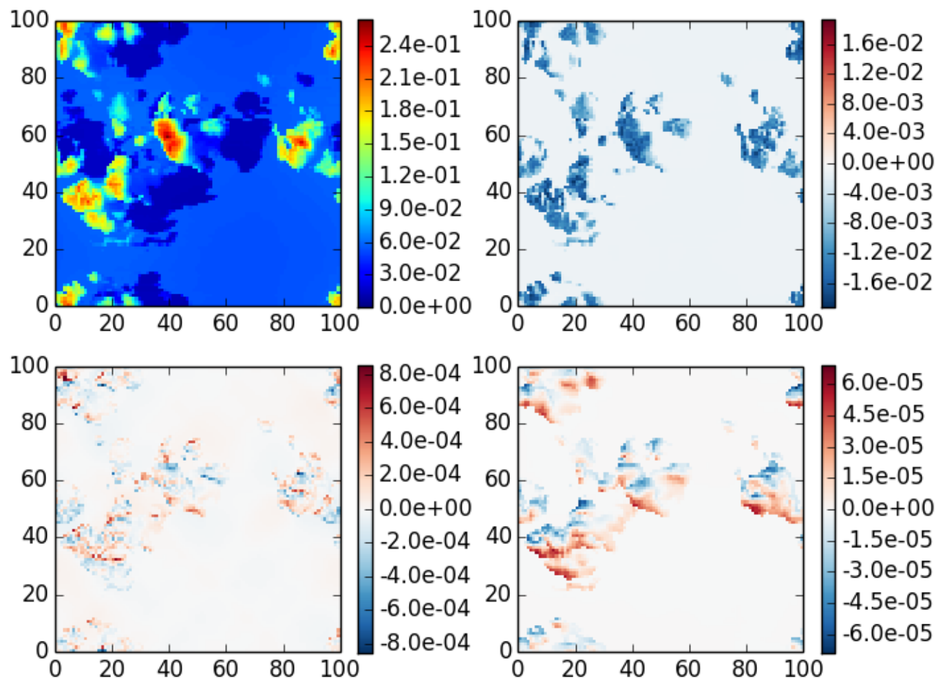
shdom3 case 5, \theta_0=40 , z=30 , \theta=180 , \phi=0
