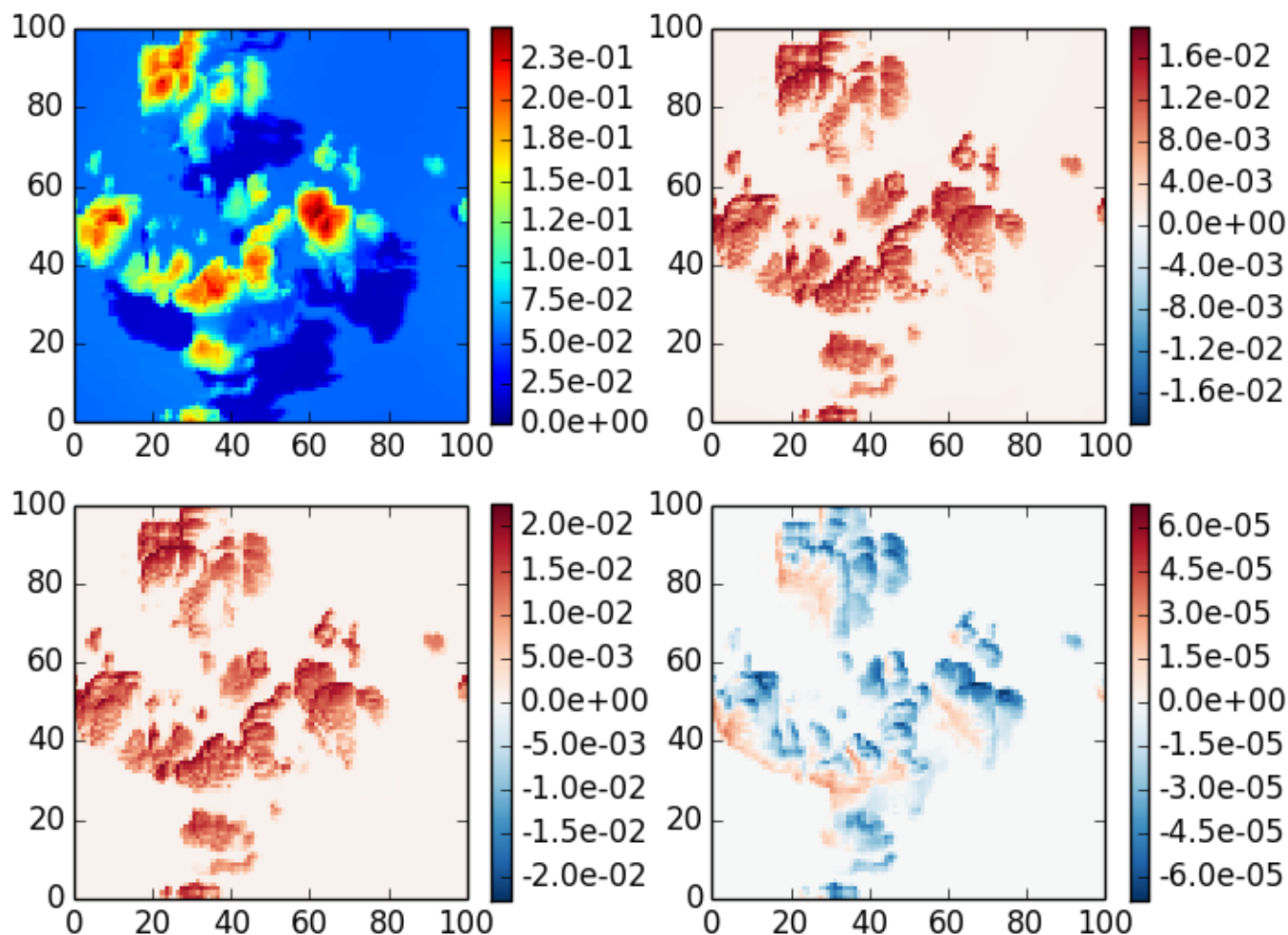
shdom3 case 7, \theta_0=40 , z=30 , \theta=140 , \phi=60
