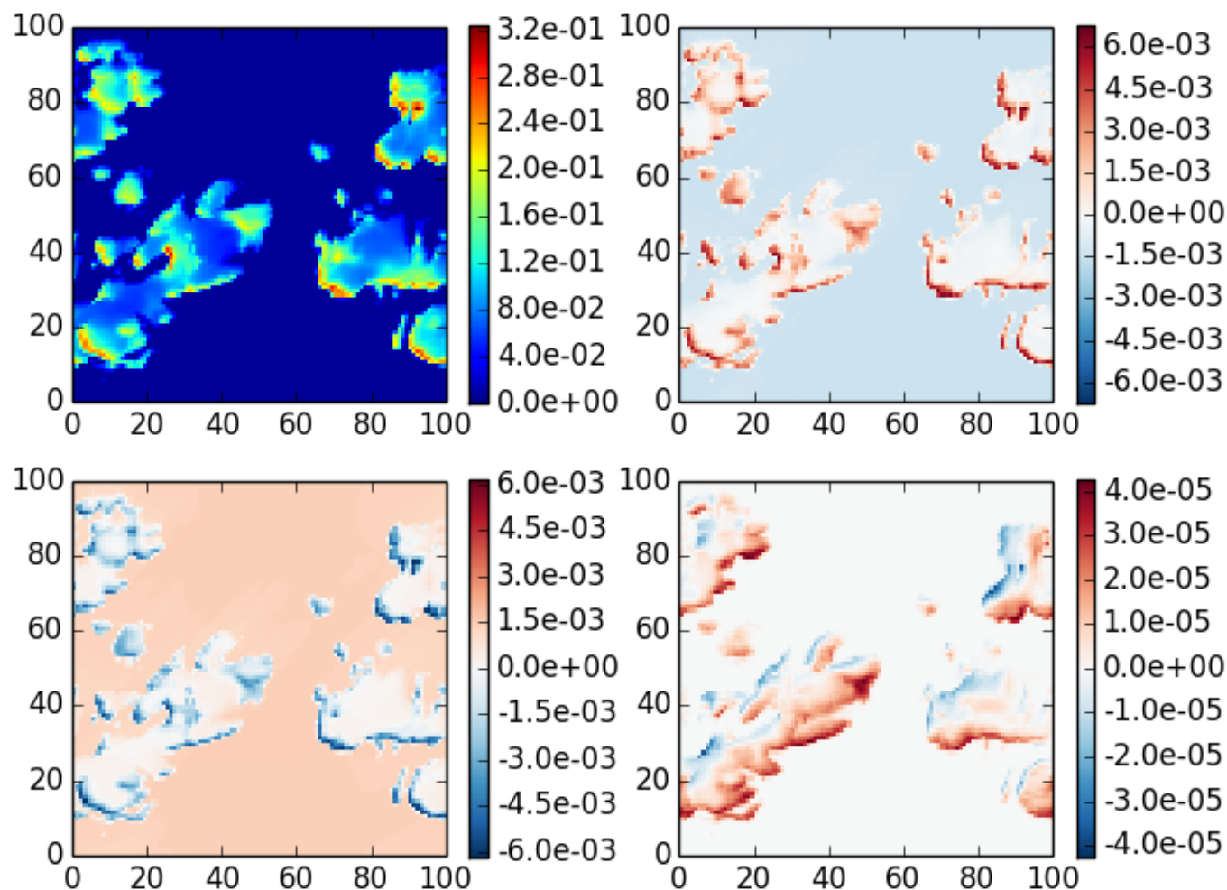
shdom3 case 2, \theta_0=20 , z=0 , \theta=40 , \phi=60
