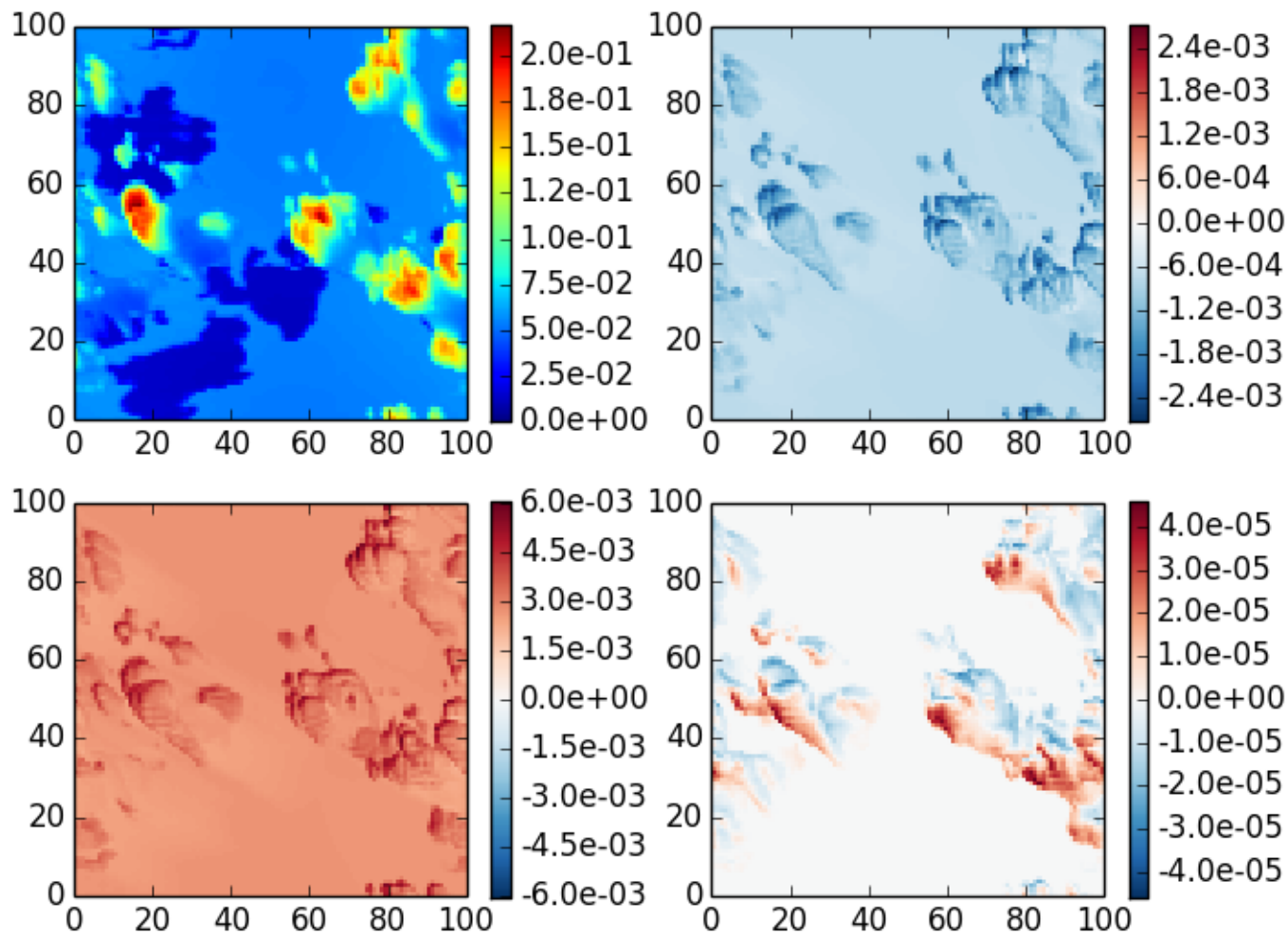
shdom3 case 8, \theta_0=40 , z=30 , \theta=140 , \phi=120
