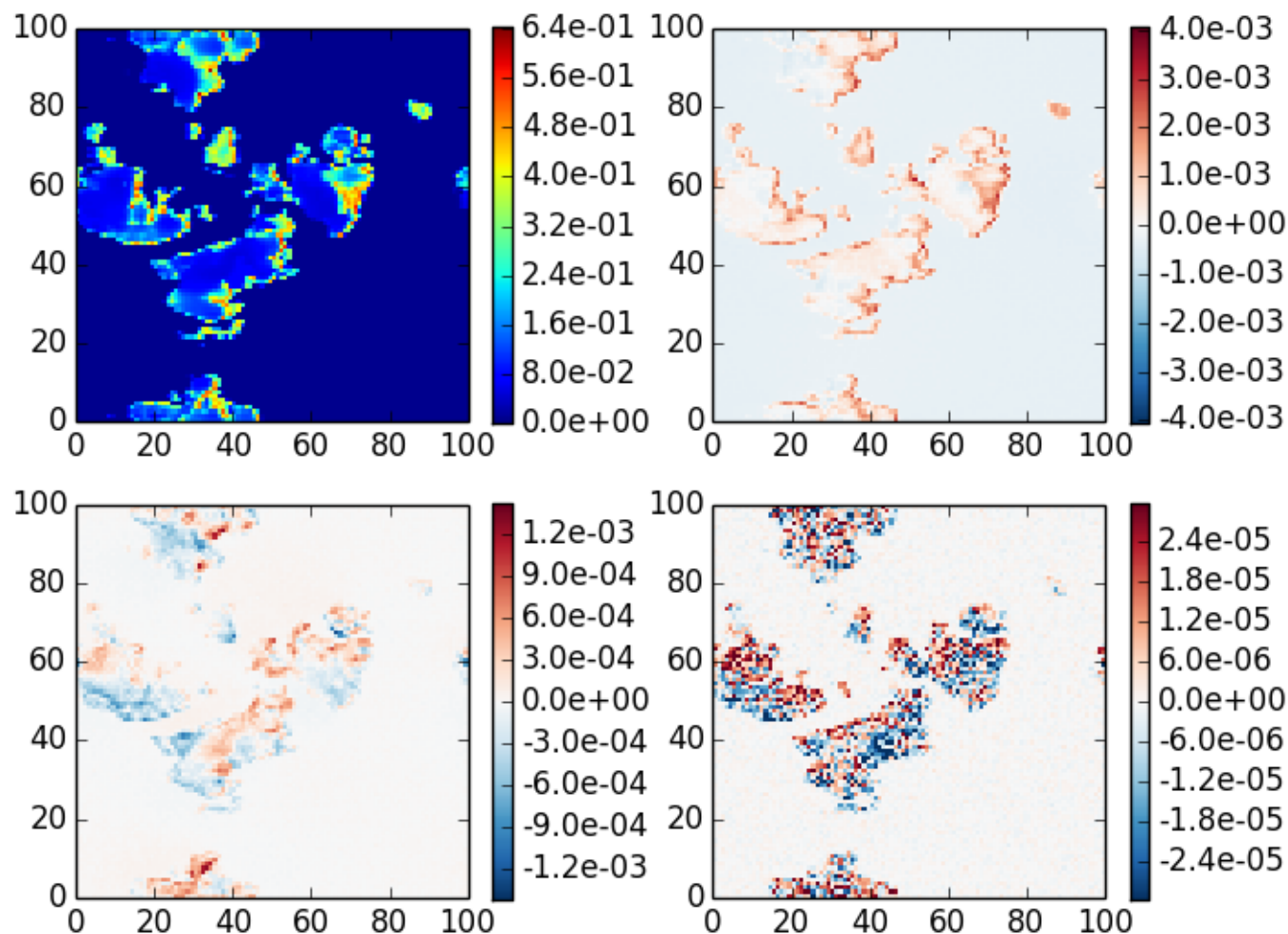
mystic case 4, \theta_0=20 , z=0 , \theta=40 , \phi=180
