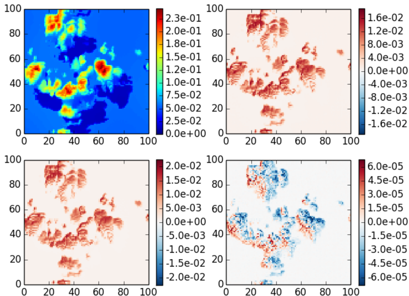
mystic case 7, \theta_0=40 , z=30 , \theta=140 , \phi=60
