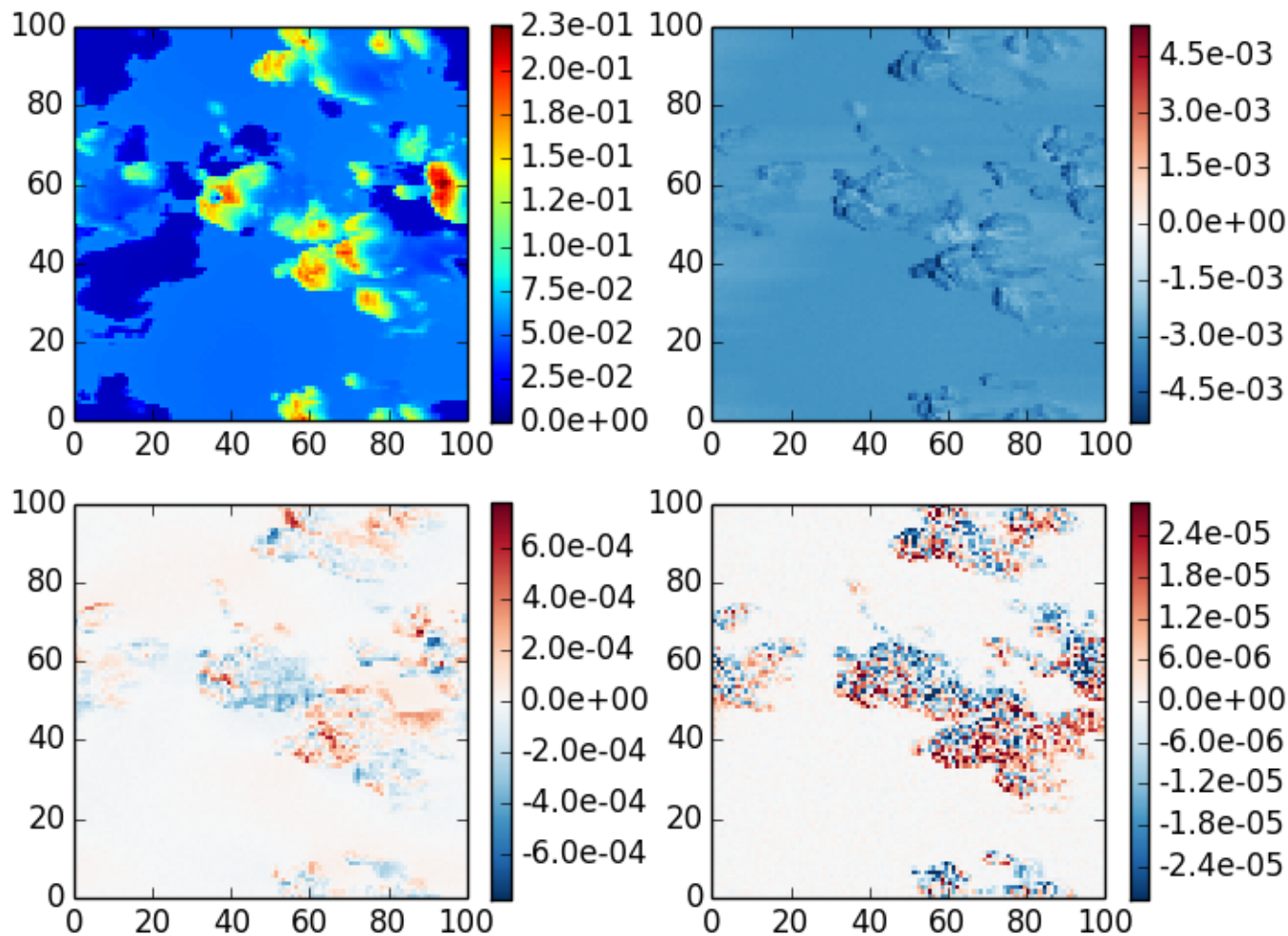
mystic case 9, \theta_0=40 , z=30 , \theta=140 , \phi=180
