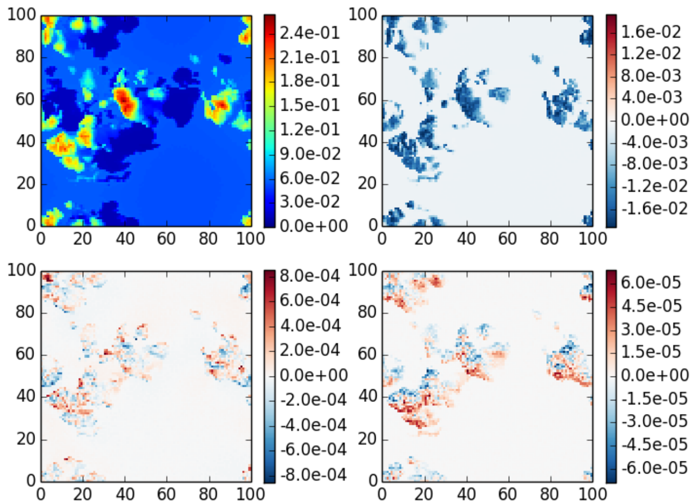
mystic case 5, \theta_0=40 , z=30 , \theta=180 , \phi=0
