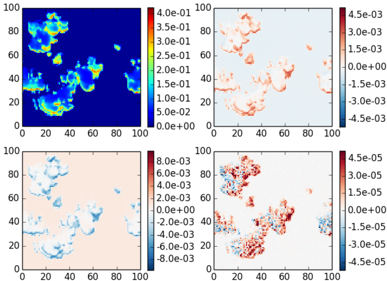
mystic case 3, \theta_0=20 , z=0 , \theta=40 , \phi=120
