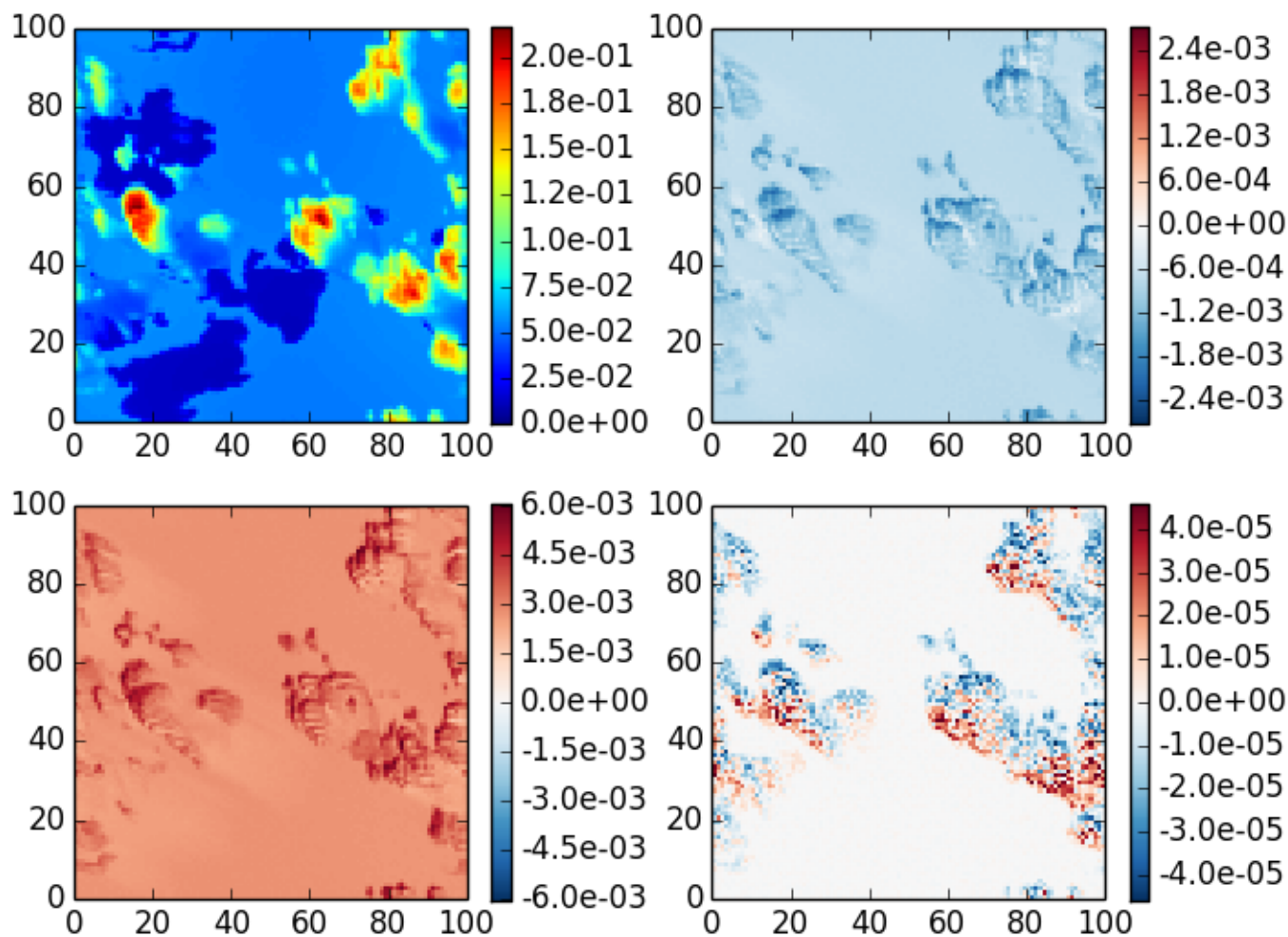
mystic case 8, \theta_0=40 , z=30 , \theta=140 , \phi=120
