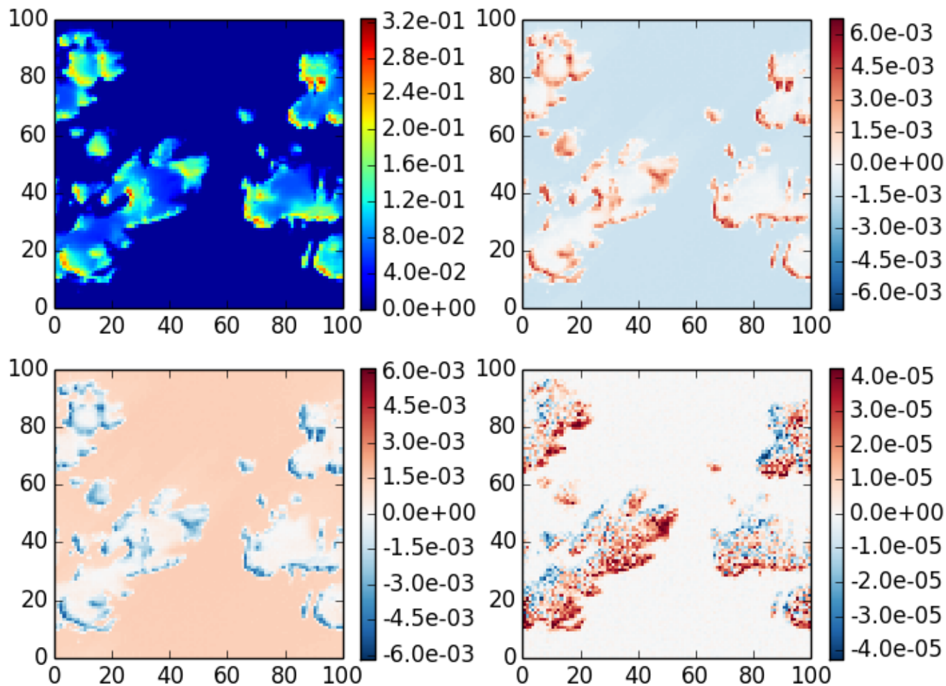
mystic case 2, \theta_0=20 , z=0 , \theta=40 , \phi=60
