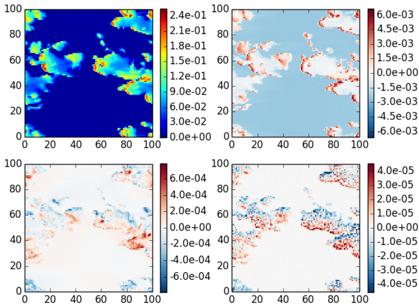
mystic case 1, \theta_0=20 , z=0 , \theta=40 , \phi=0
