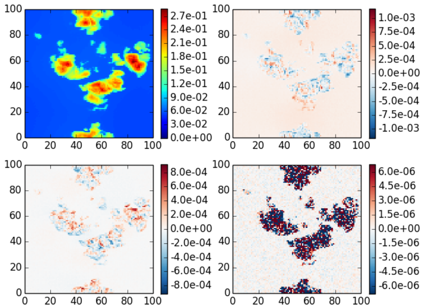
mystic case 6, \theta_0=40 , z=30 , \theta=140 , \phi=0
