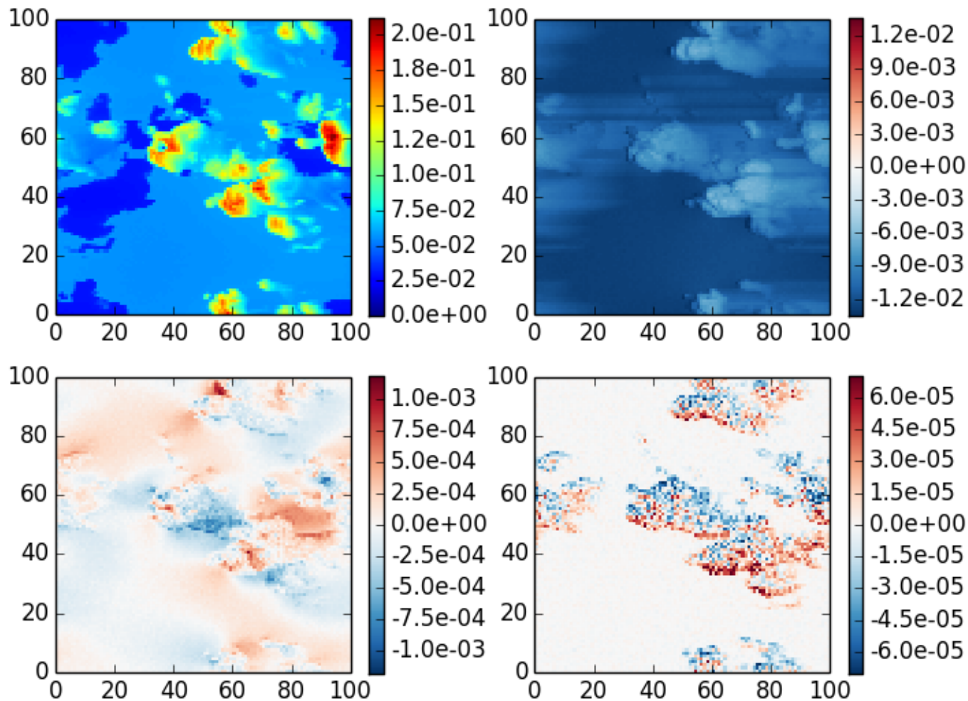
mscart_fm case 9, \theta_0=40 , z=30 , \theta=140 , \phi=180
