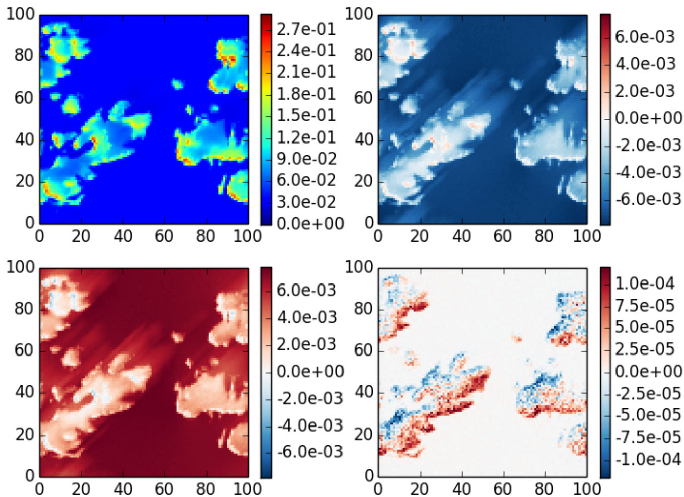
mscart_fm case 2, \theta_0=20 , z=0 , \theta=40 , \phi=60
