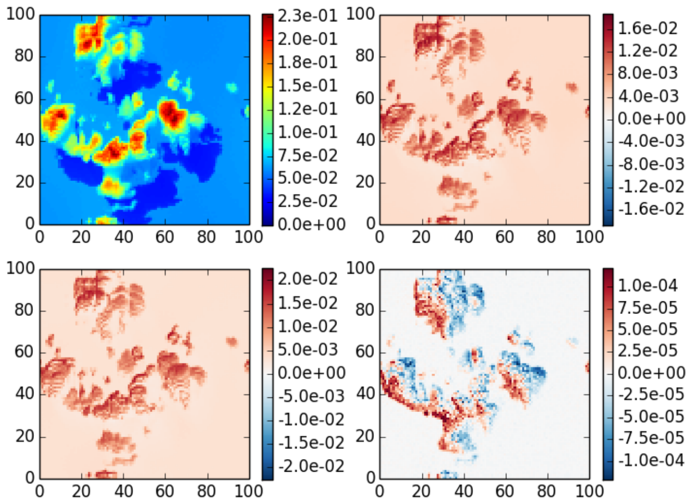
mscart_fmc case 7, \theta_0=40 , z=30 , \theta=140 , \phi=60
