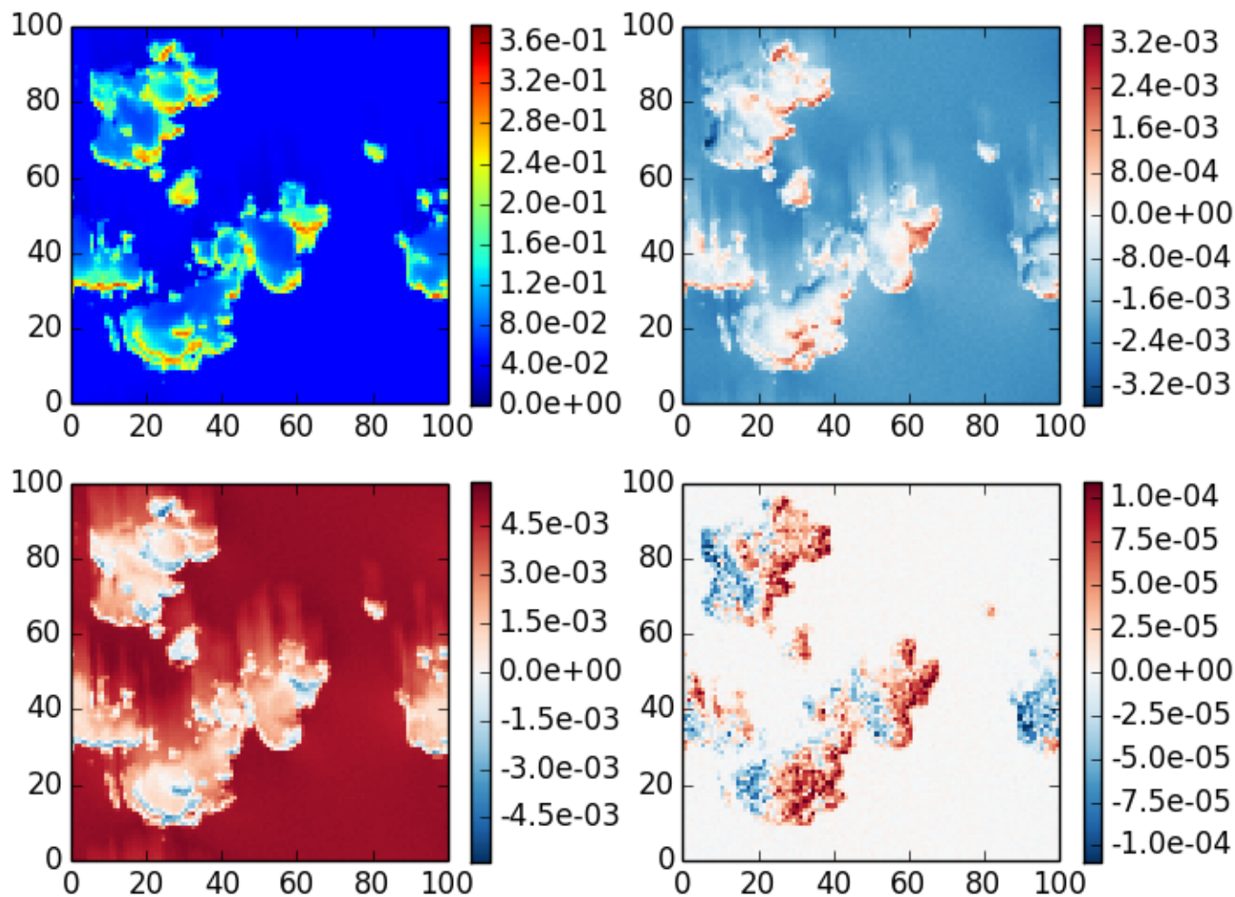
mscart_fmc case 3, \theta_0=20 , z=0 , \theta=40 , \phi=120
