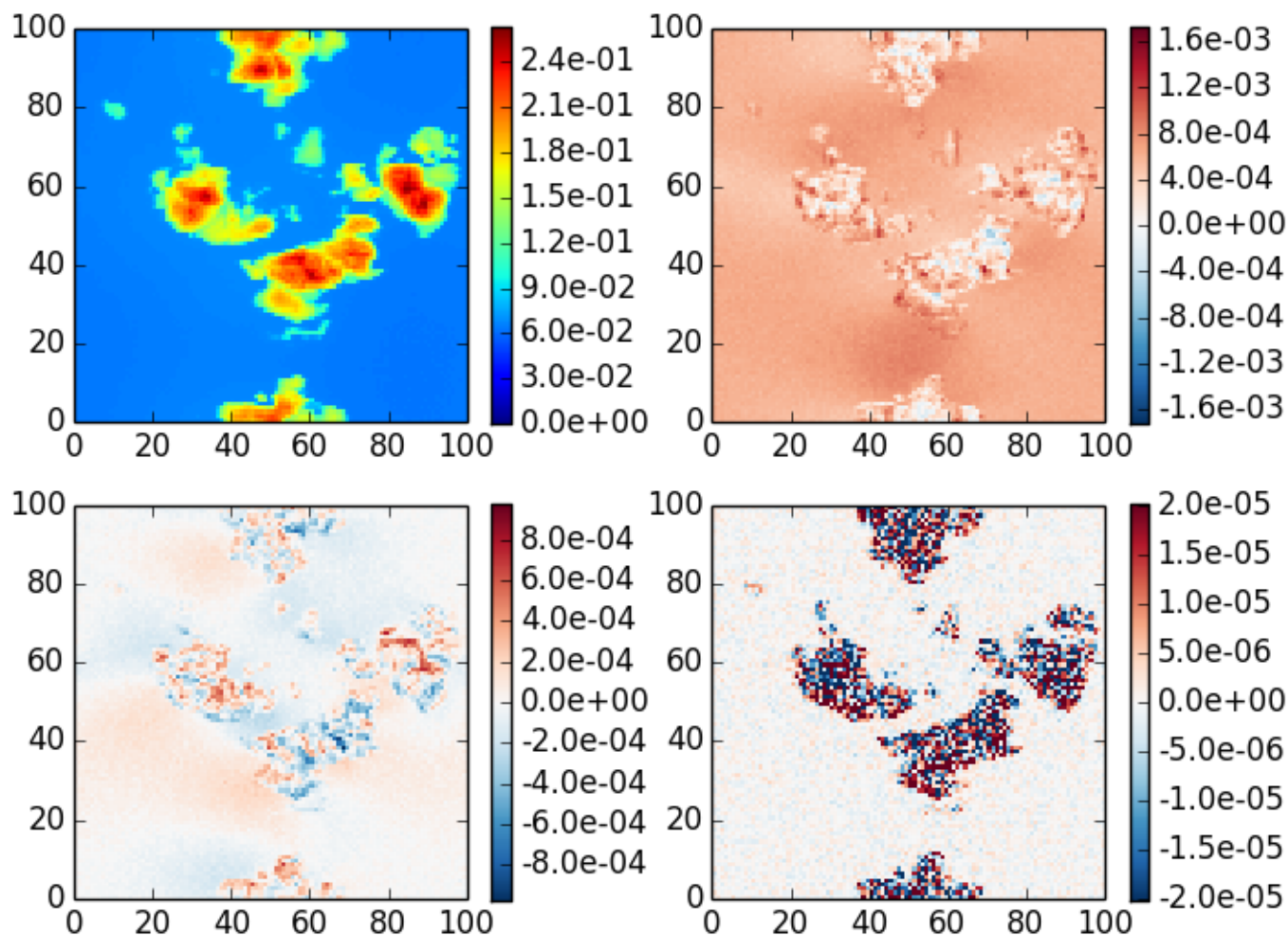
mcart_fm case 6, \theta_0=40 , z=30 , \theta=140 , \phi=0
