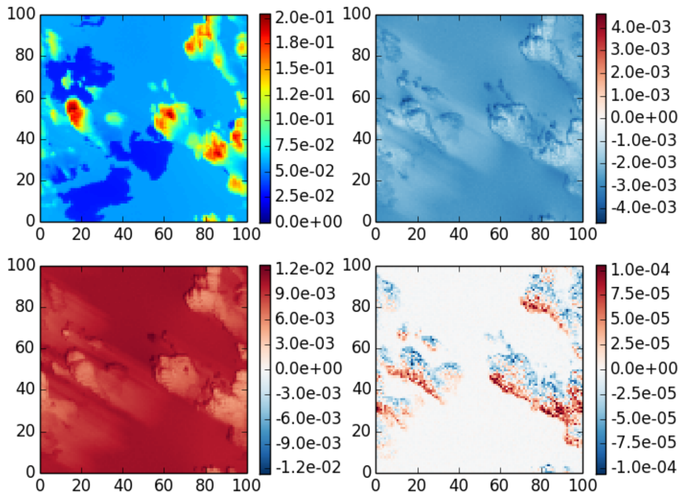
mscart_fm case 8, \theta_0=40 , z=30 , \theta=140 , \phi=120
