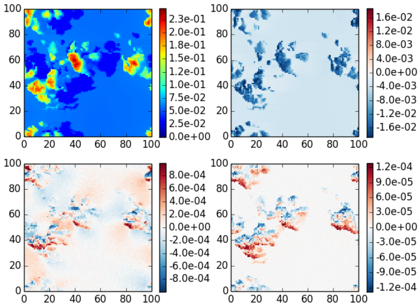
mcart_bmc case 5, \theta_0=40 , z=30 , \theta=180 , \phi=0
