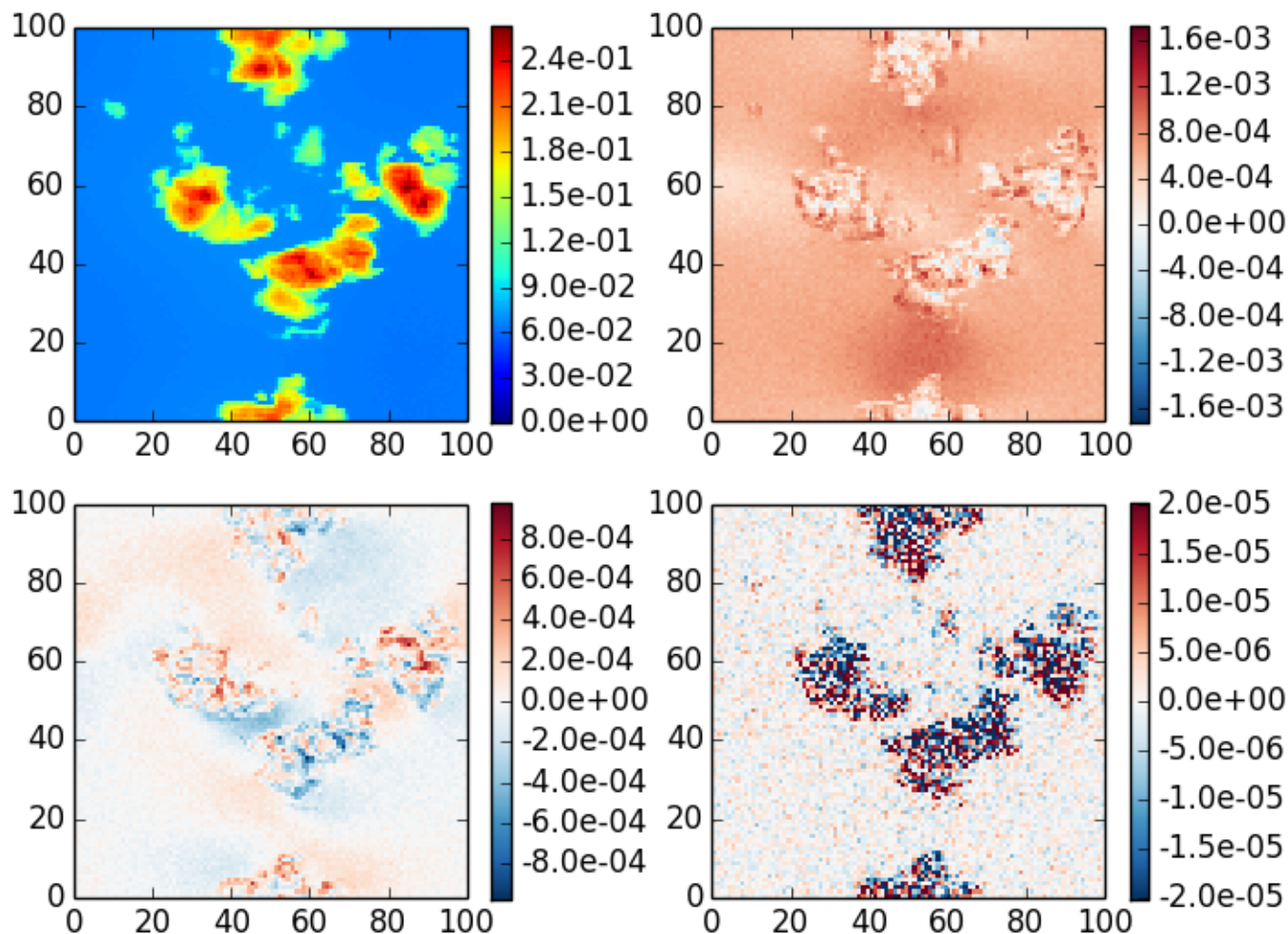
mscart_bmc case 6, \theta_0=40 , z=30 , \theta=140 , \phi=0
