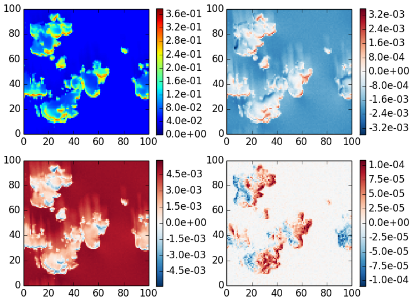
mscart_bmc case 3, \theta_0=20 , z=0 , \theta=40 , \phi=120
