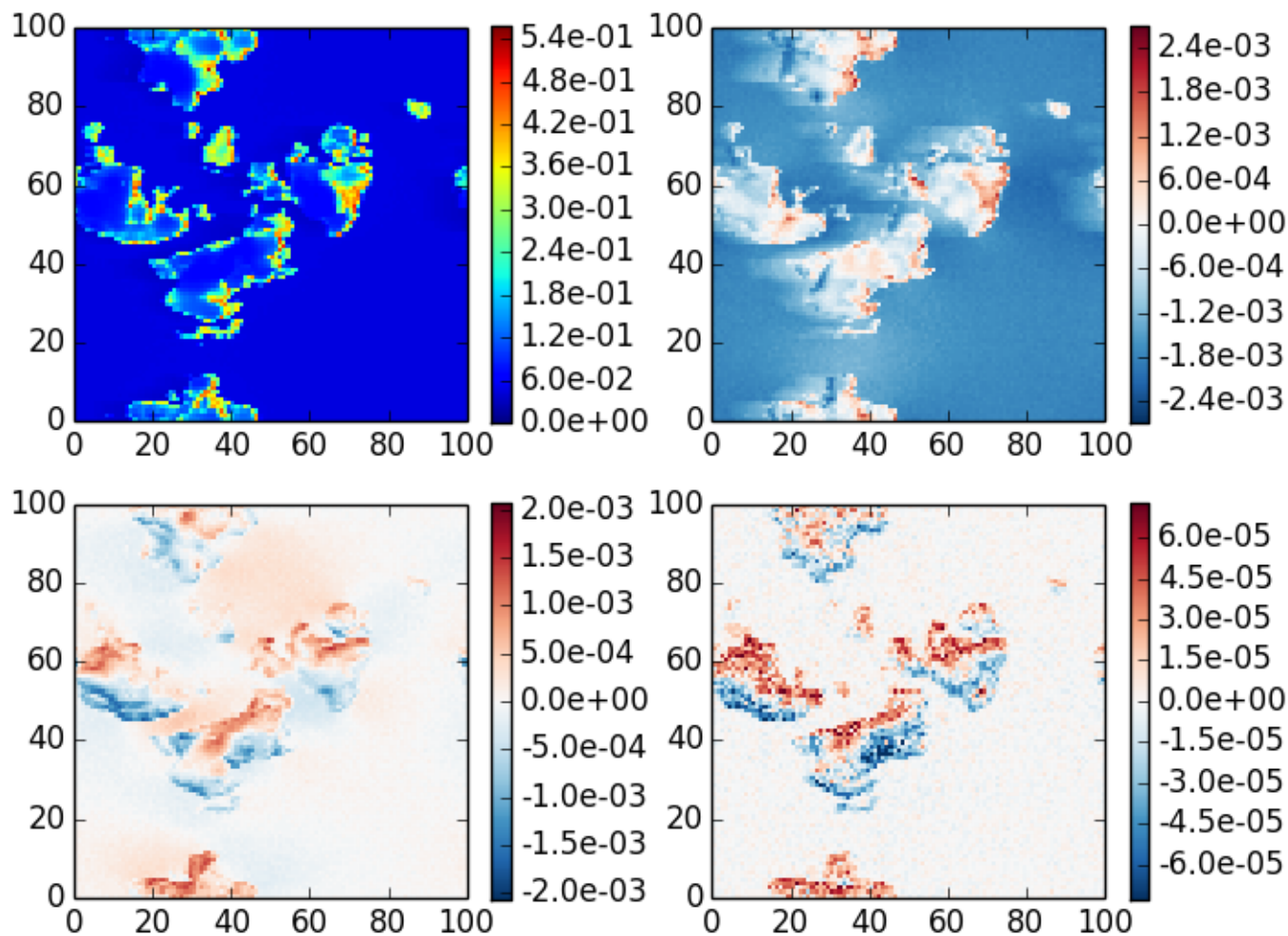
mcart_bmc case 4, \theta_0=20 , z=0 , \theta=40 , \phi=180
