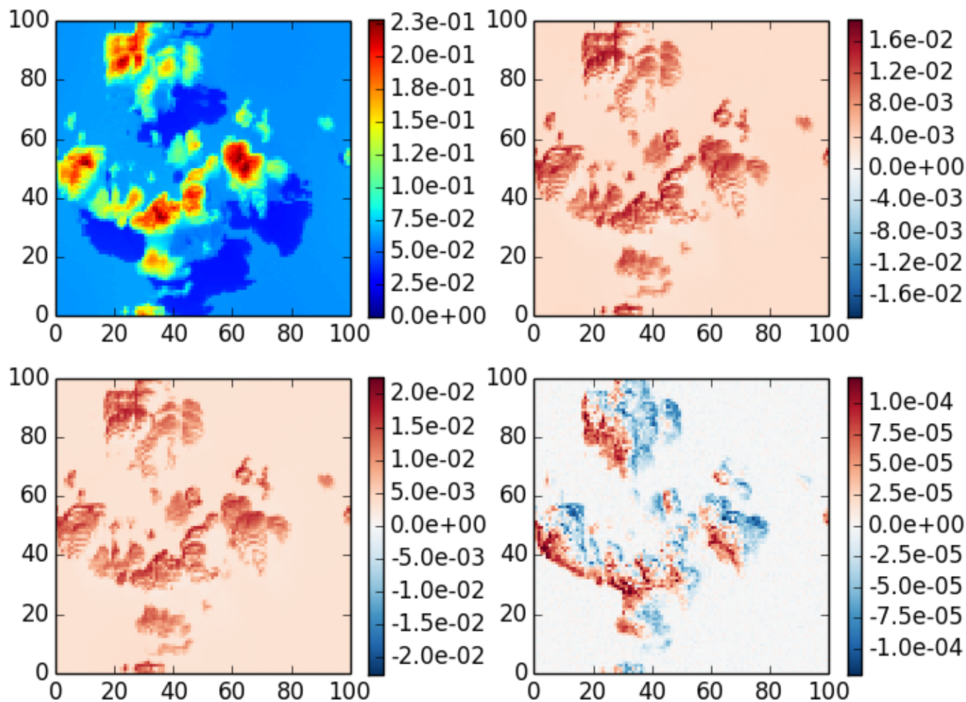
mcart_bmc case 7, \theta_0=40 , z=30 , \theta=140 , \phi=60
