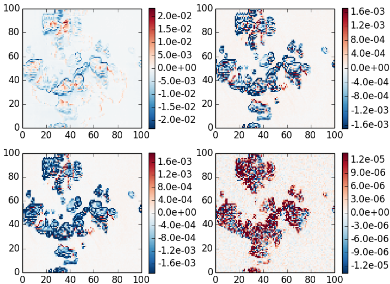
absolute difference case 7, \theta_0=40 , z=30 , \theta=140 , \phi=60
