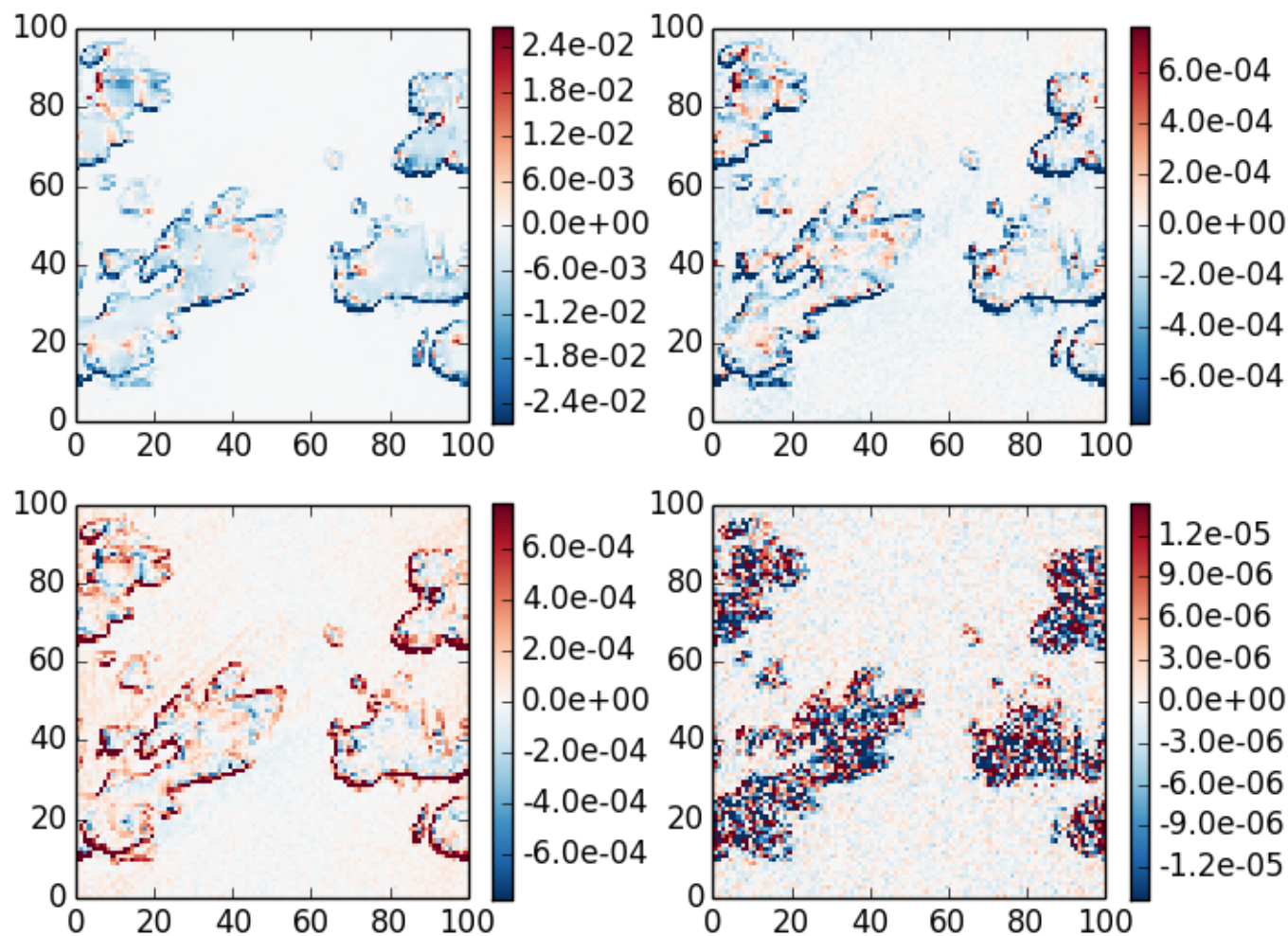
absolute difference case 2, \theta_0=20 , z=0 , \theta=40 , \phi=60
