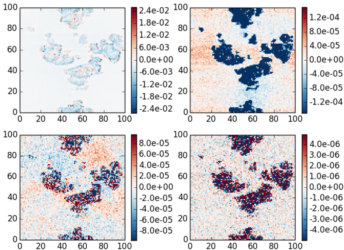
absolute difference case 6, \theta_0=40 , z=30 , \theta=140 , \phi=0
