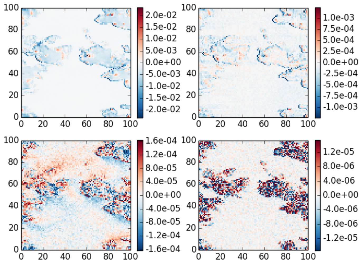
absolute difference case 1, \theta_0=20 , z=0 , \theta=40 , \phi=0
