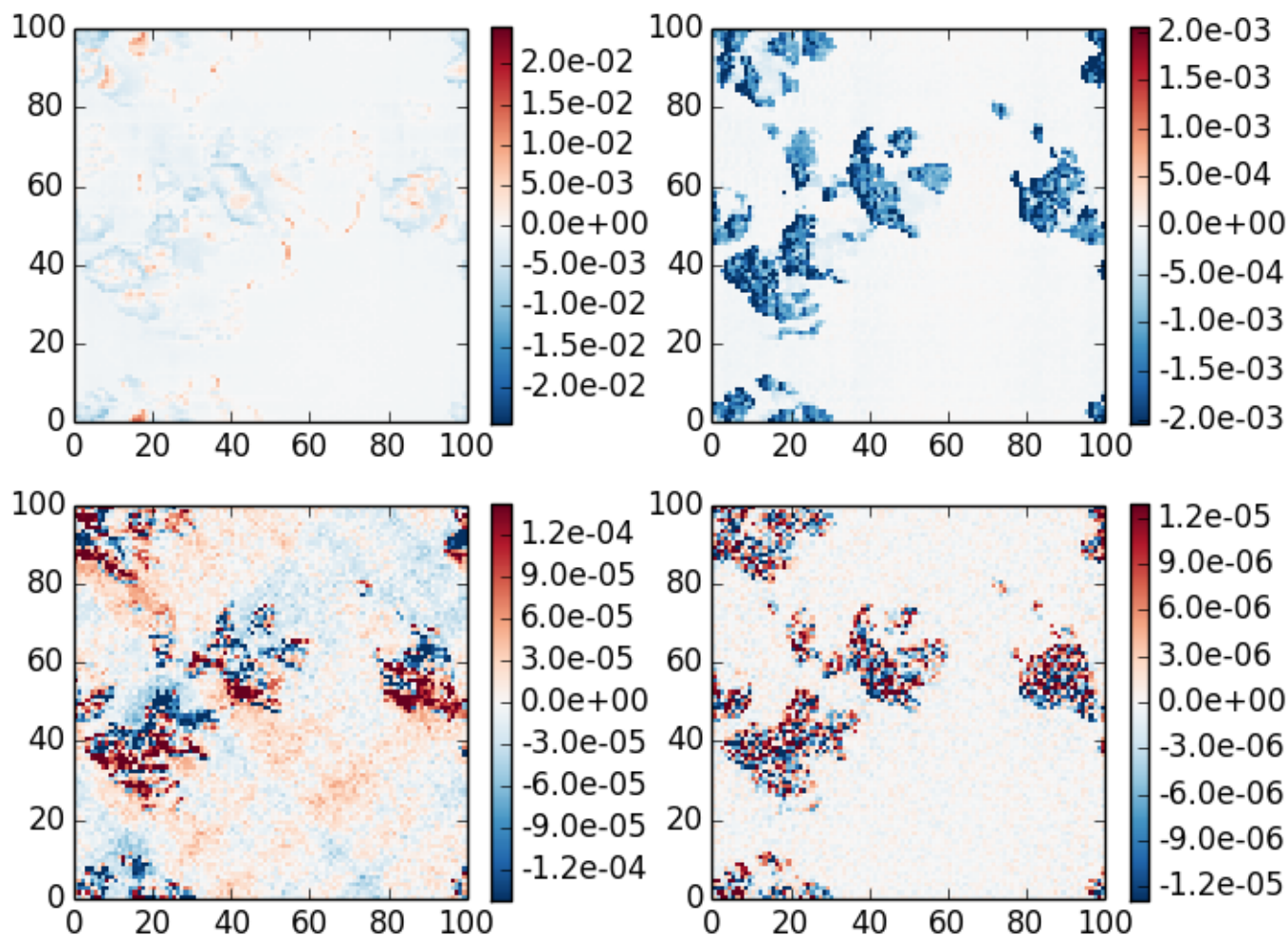
absolute difference case 5, \theta_0=40 , z=30 , \theta=180 , \phi=0
