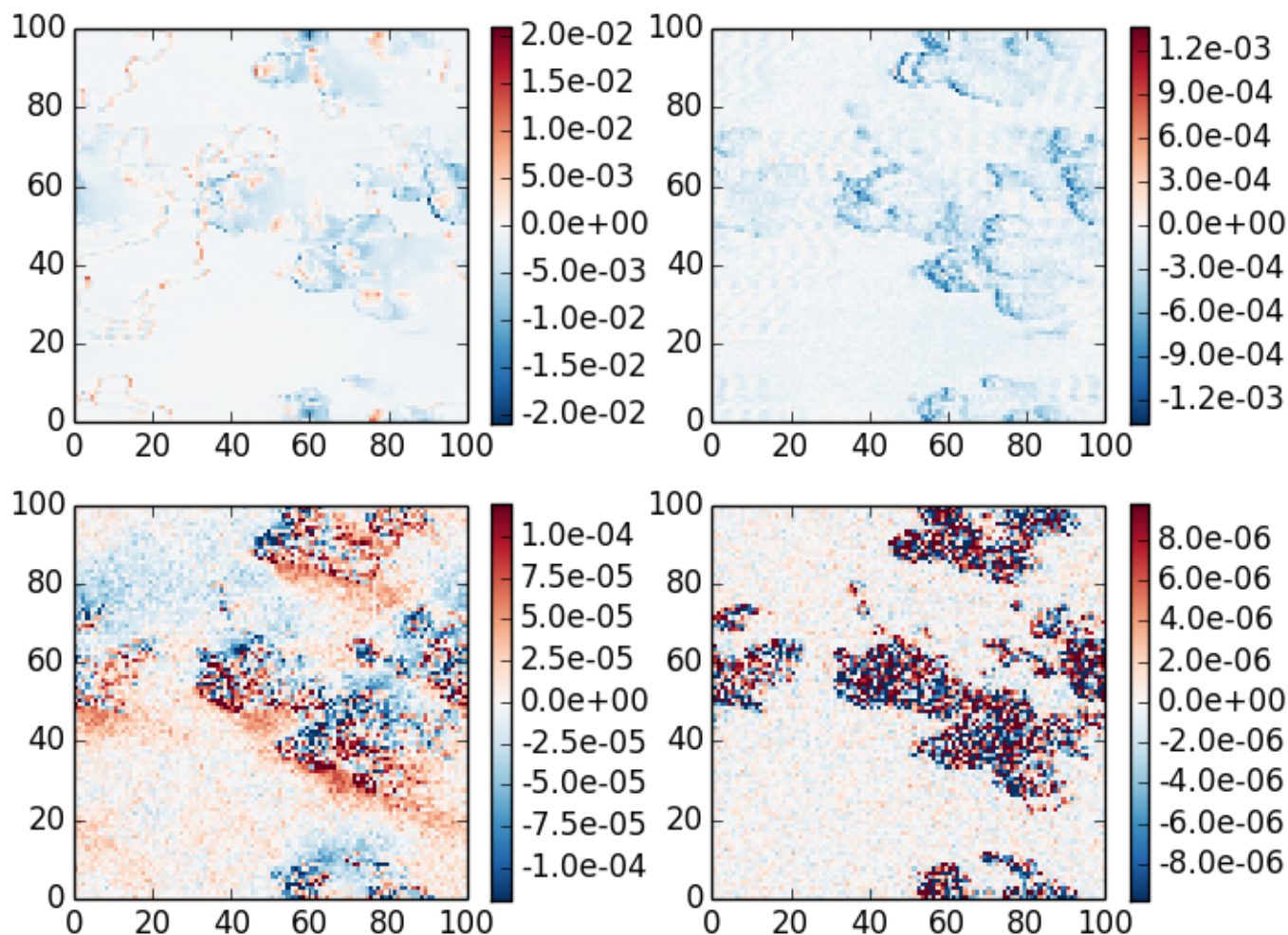
absolute difference case 9, \theta_0=40 , z=30 , \theta=140 , \phi=180
