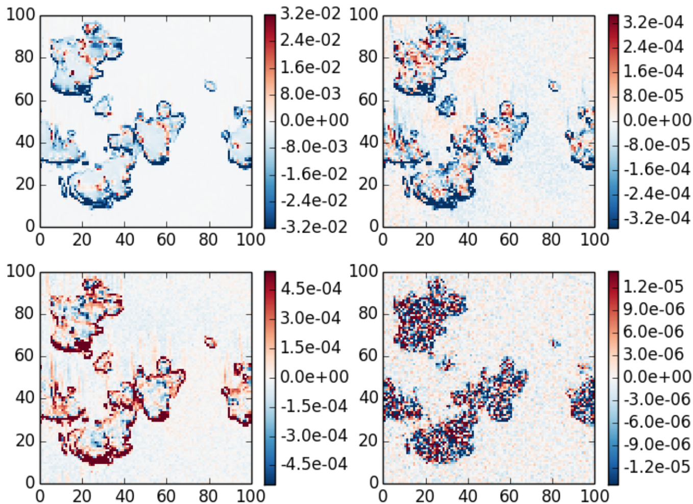
absolute difference case 3, \theta_0=20 , z=0 , \theta=40 , \phi=120
