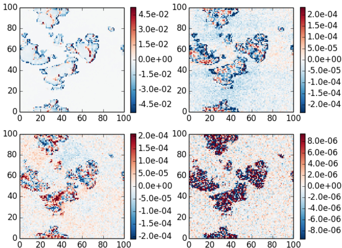
absolute difference case 4, \theta_0=20 , z=0 , \theta=40 , \phi=180
