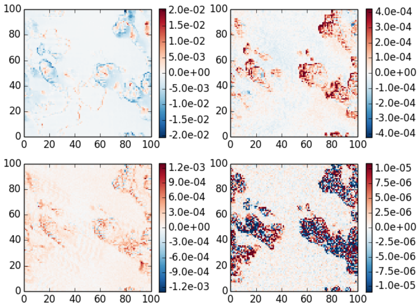
absolute difference case 8, \theta_0=40 , z=30 , \theta=140 , \phi=120
