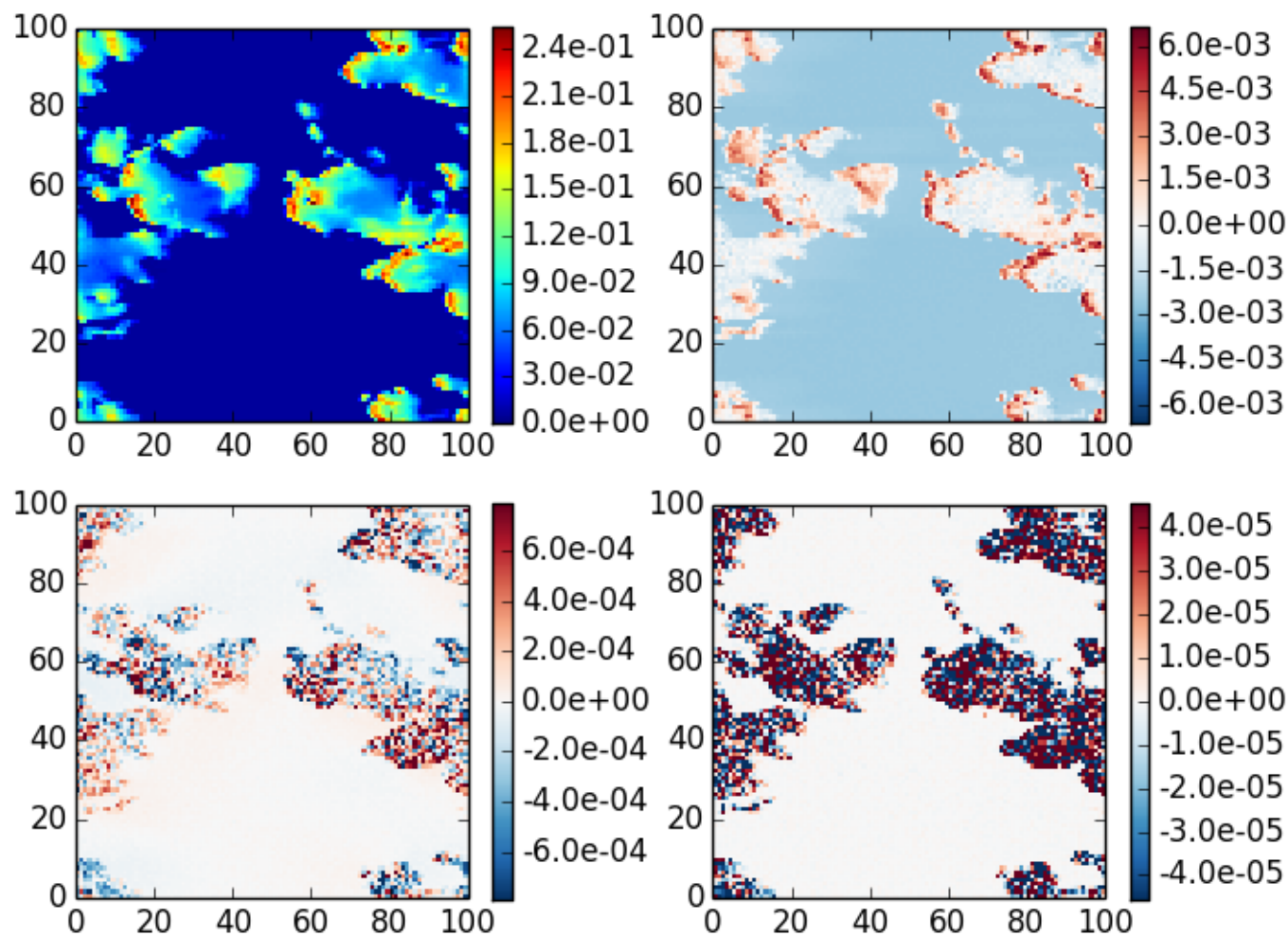
3DMCPOL case 1, \theta_0=20 , z=0 , \theta=40 , \phi=0
