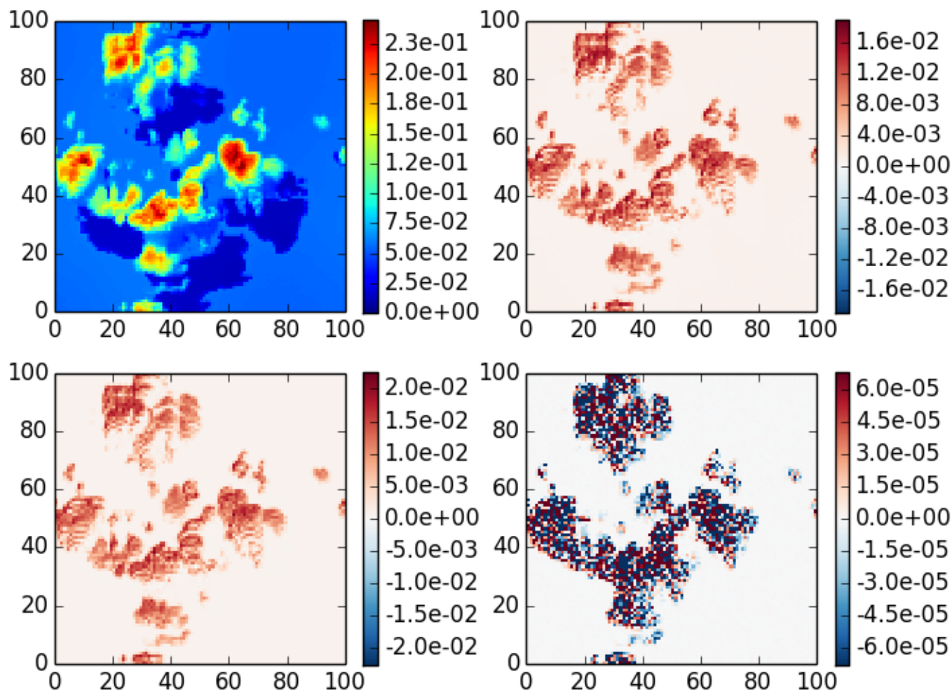
3DMCPOL case 7, \theta_0=40 , z=30 , \theta=140 , \phi=60
