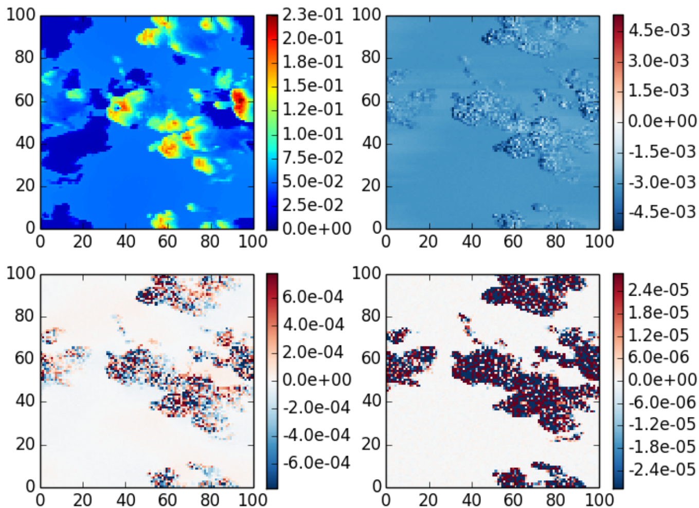
3DMCPOL case 9, \theta_0=40 , z=30 , \theta=140 , \phi=180
