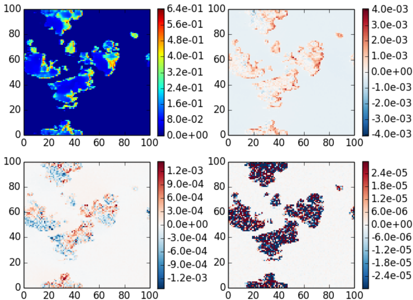
3DMCPOL case 4, \theta_0=20 , z=0 , \theta=40 , \phi=180
