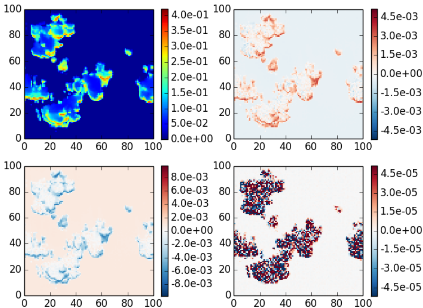
3DMCPOL case 3, \theta_0=20 , z=0 , \theta=40 , \phi=120
