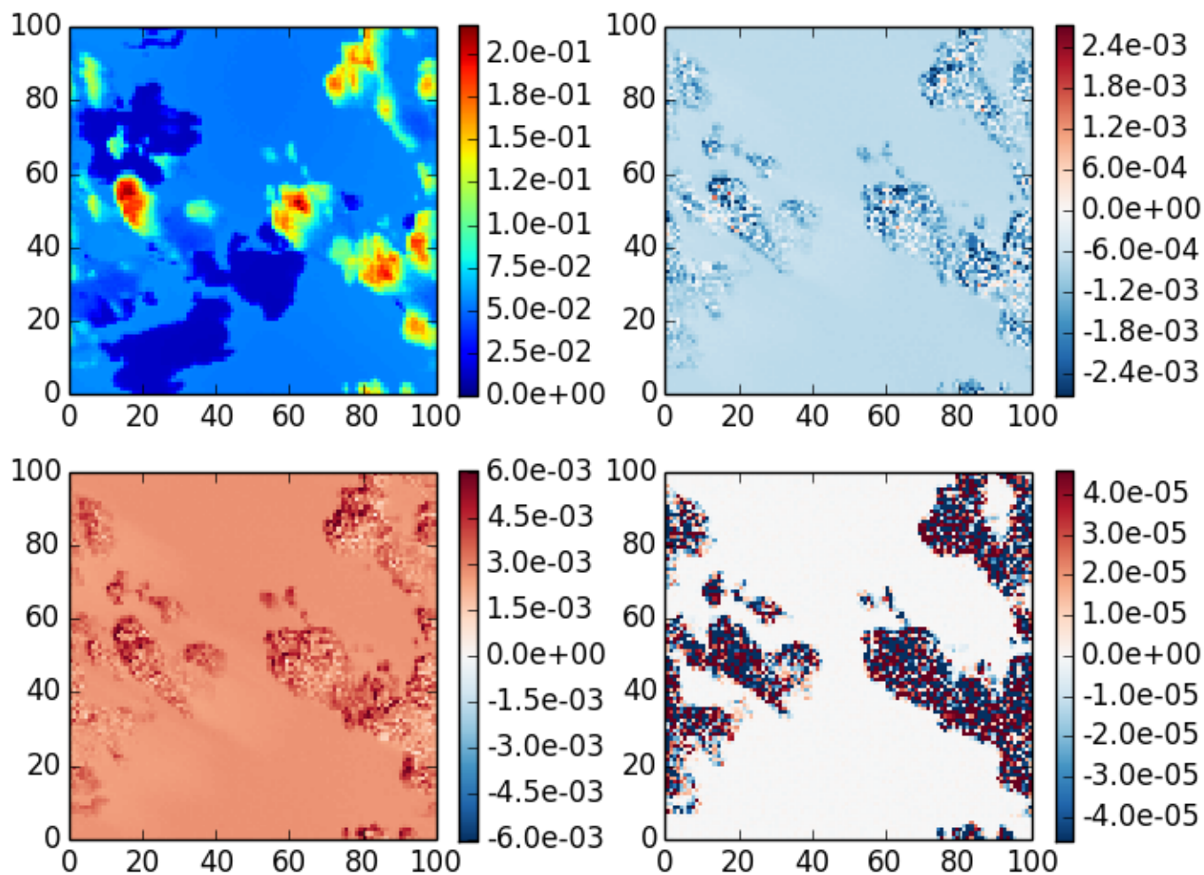
3DMCPOL case 8, \theta_0=40 , z=30 , \theta=140 , \phi=120
