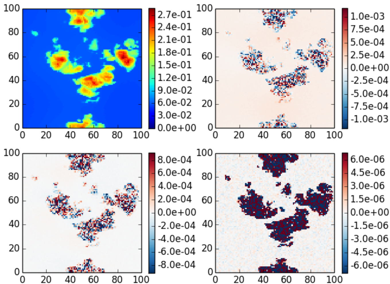
3DMCPOL case 6, \theta_0=40 , z=30 , \theta=140 , \phi=0
