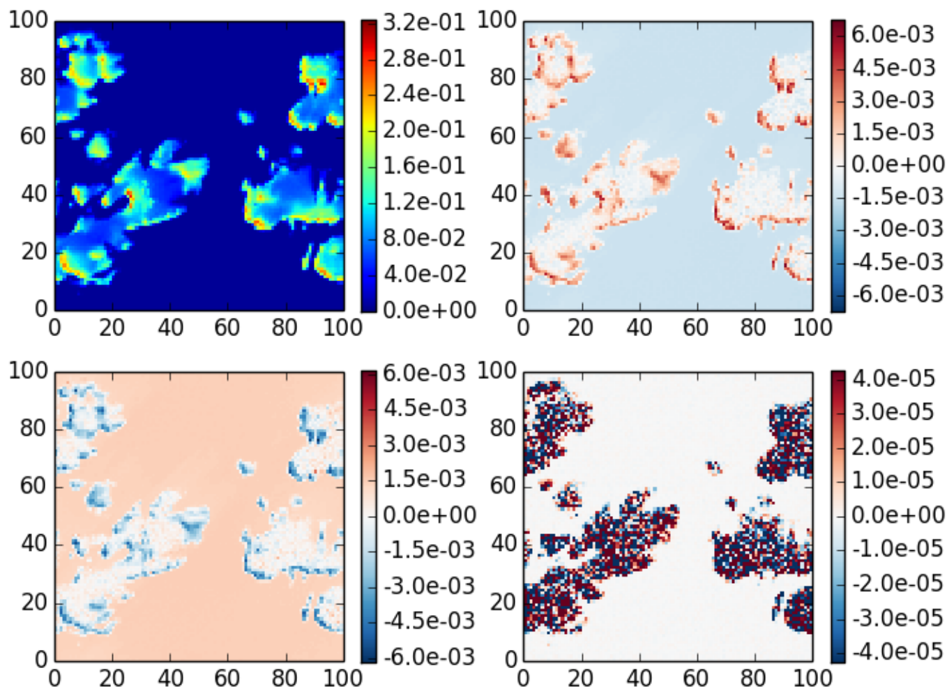
3DMCPOL case 2, \theta_0=20 , z=0 , \theta=40 , \phi=60
