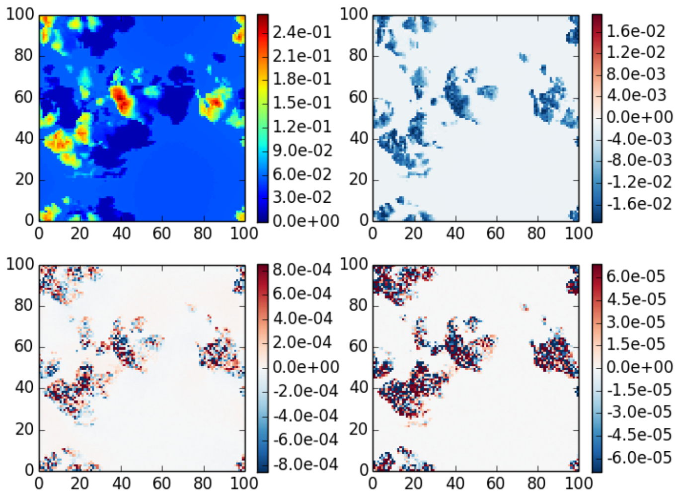
3DMCPOL case 5, \theta_0=40 , z=30 , \theta=180 , \phi=0
