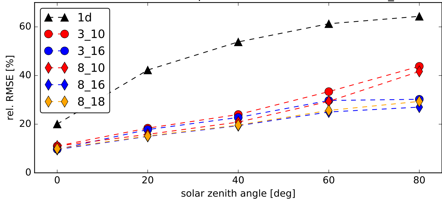
srfc irradiance errors cmped to MYSTIC for scene `menno_710`
