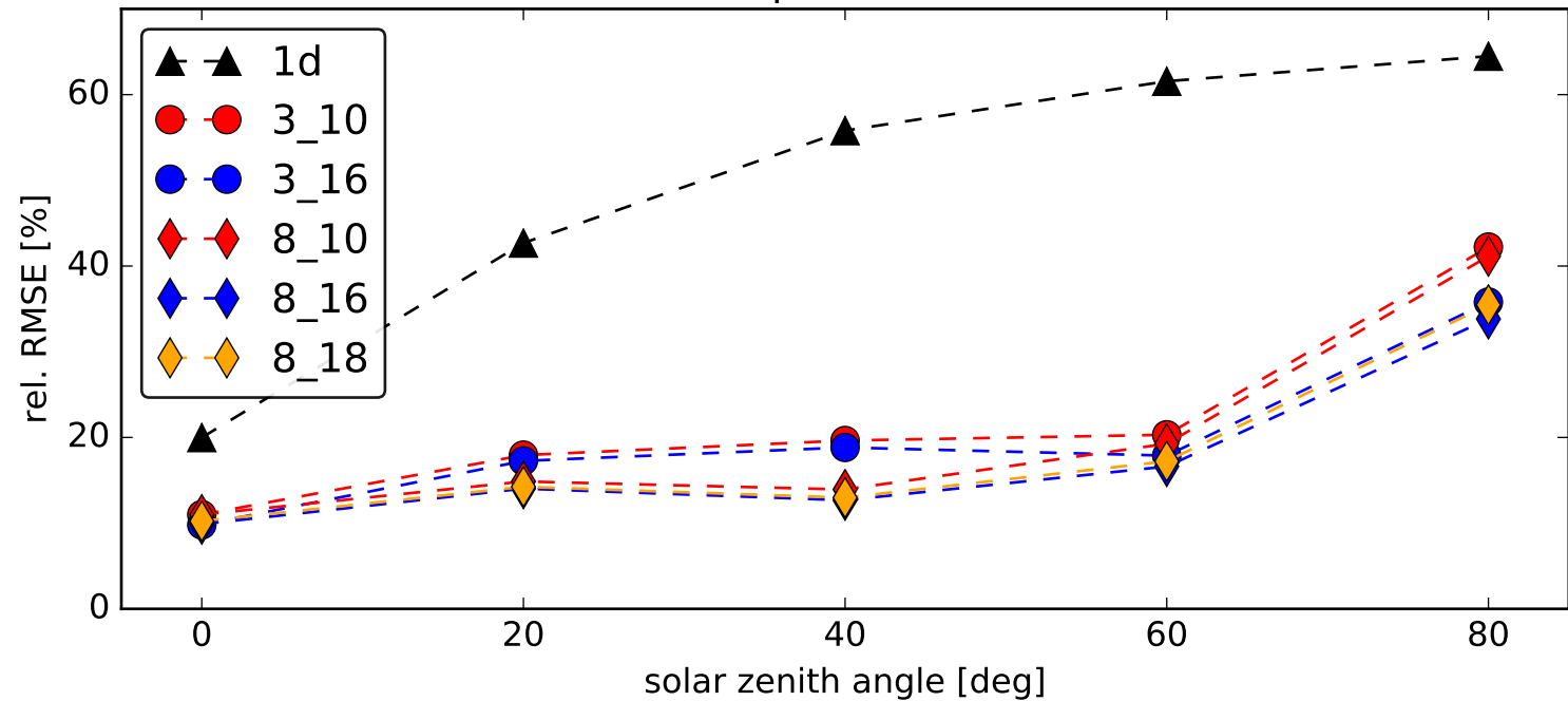
srfc irradiance errors cmped to MYSTIC for scene `i3rc1`
