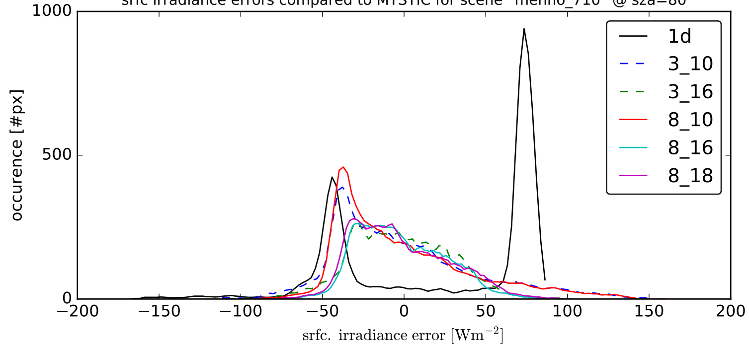
srfc irradiance errors compared to MYSTIC for scene `menno_710` @ sza=80
