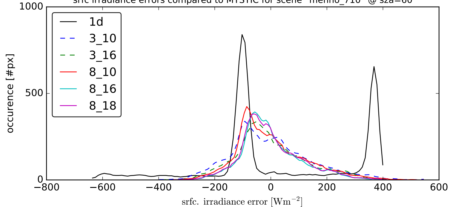
srfc irradiance errors compared to MYSTIC for scene `menno_710` @ sza=60
