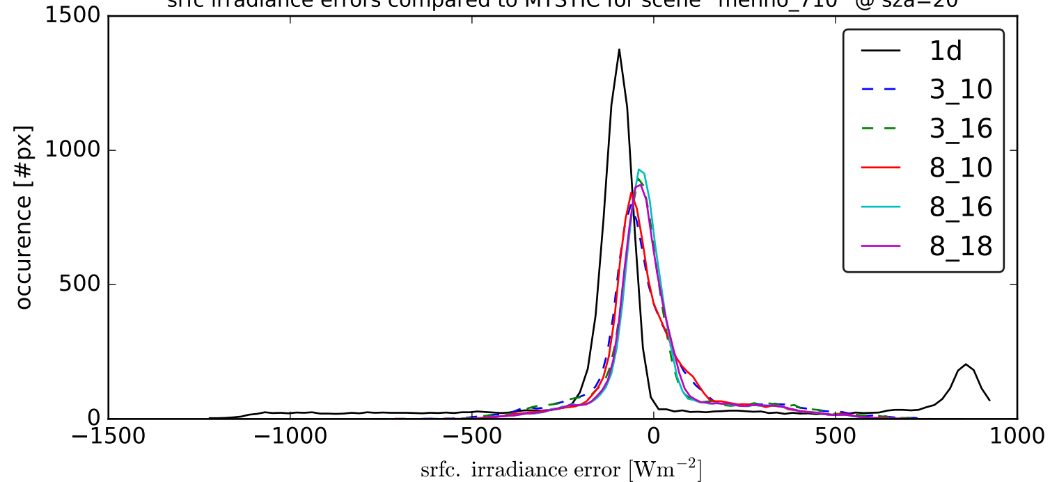
srfc irradiance errors compared to MYSTIC for scene `menno_710` @ sza=20
