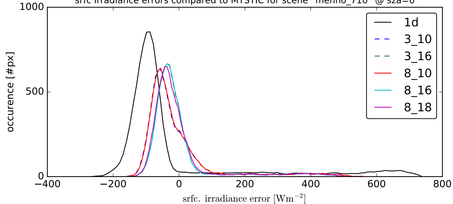
srfc irradiance errors compared to MYSTIC for scene `menno_710` @ sza=0
