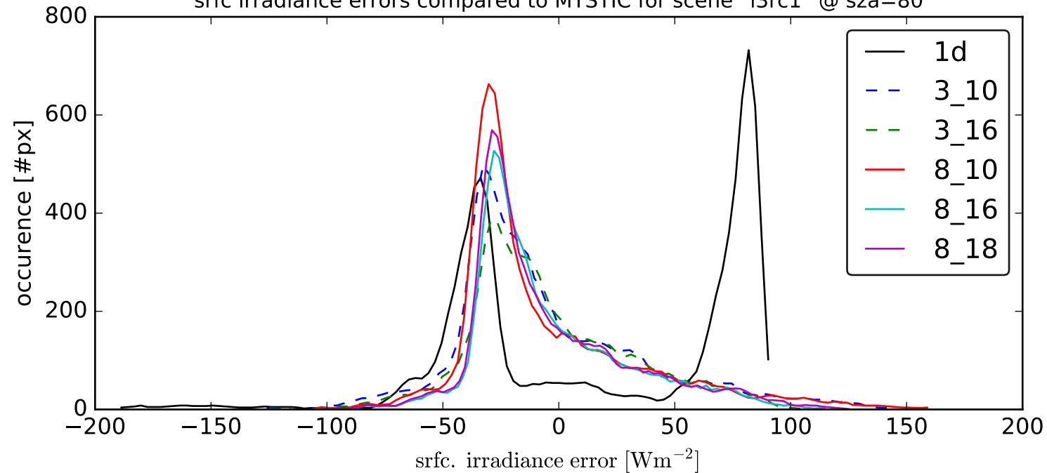
srfc irradiance errors compared to MYSTIC for scene `i3rc1` @ sza=80
