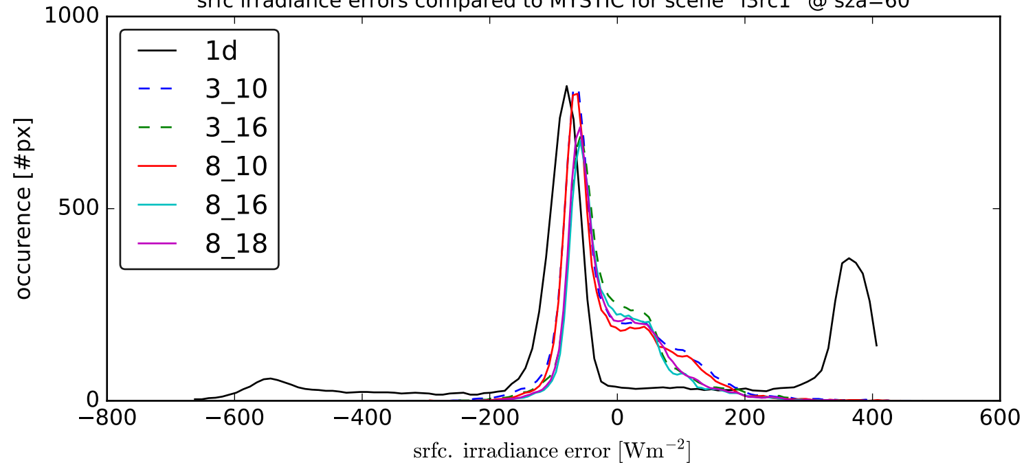
srfc irradiance errors compared to MYSTIC for scene `i3rc1` @ sza=60
