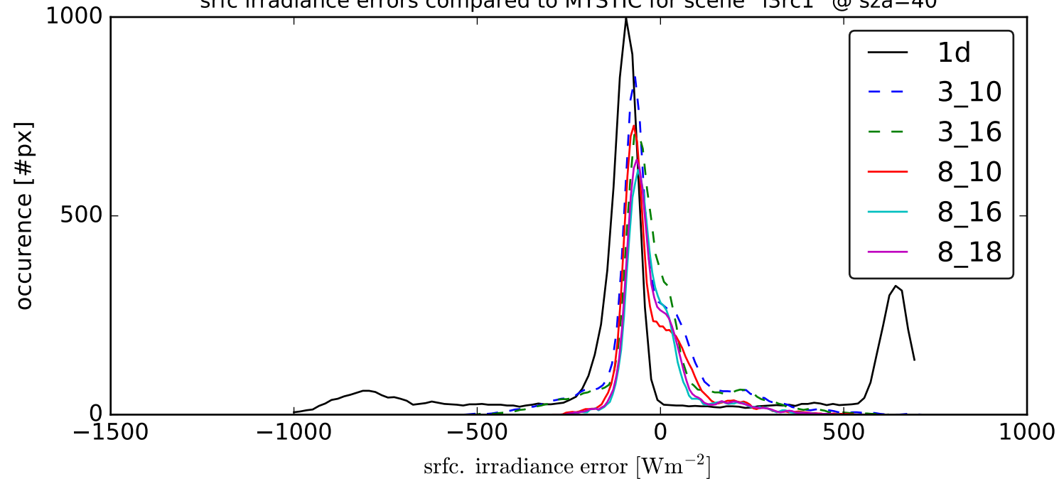
srfc irradiance errors compared to MYSTIC for scene `i3rc1` @ sza=40
