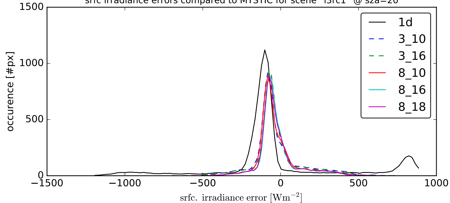
srfc irradiance errors compared to MYSTIC for scene `i3rc1` @ sza=20
