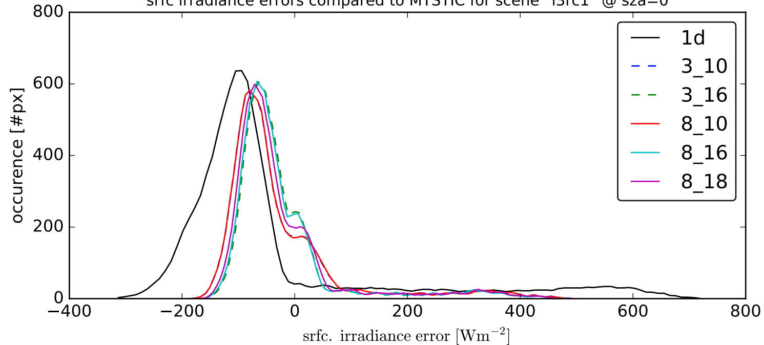
srfc irradiance errors compared to MYSTIC for scene `i3rc1` @ sza=0
