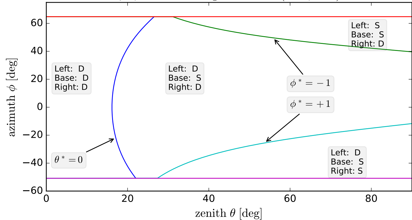
\phi^*, \theta^* Phase Diagram for C = (0.80, 0.97)
