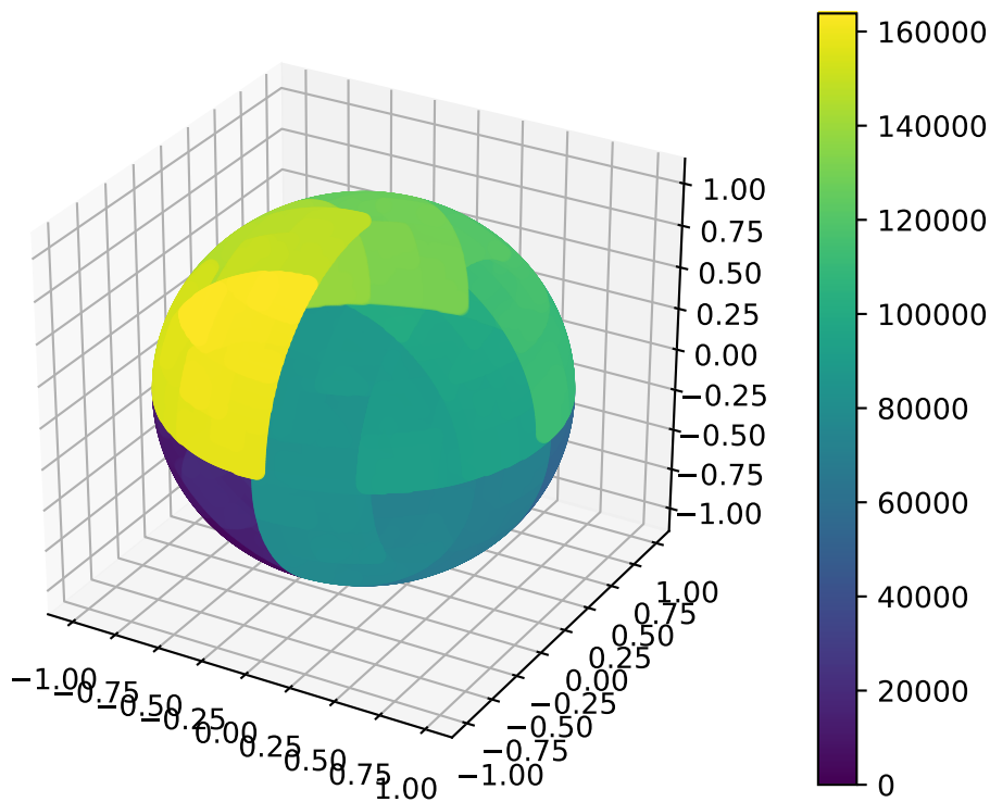
hilbert-curve mesh
