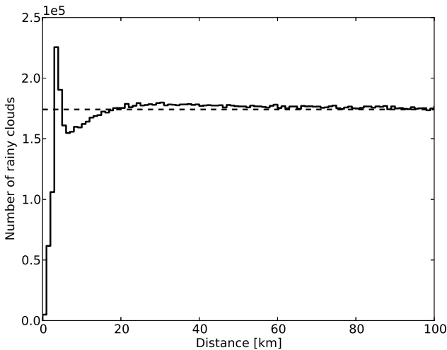
Figure 6: Distribution of distance between different clouds.
