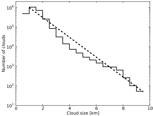
Figure 5: Logarithmic cloud size distribution for clouds with a height above 90.04.
