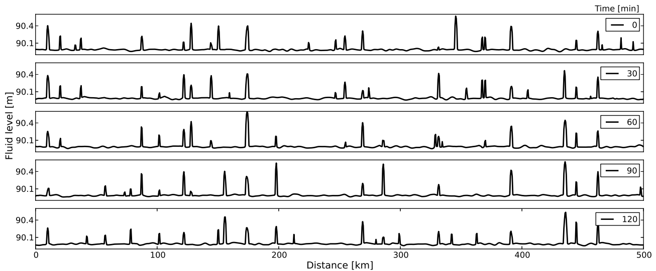
Figure 4: Typical evolution of the cloud field in the whole model domain.
