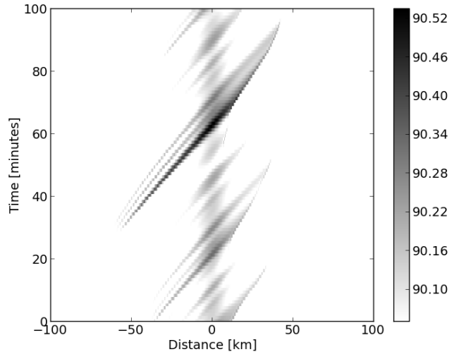
Figure 7: Hovmöller diagram for a mean wind of 30 \text{ m s}^{-1} . Marked are only gridpoints where the water level is above 90.05 m.
