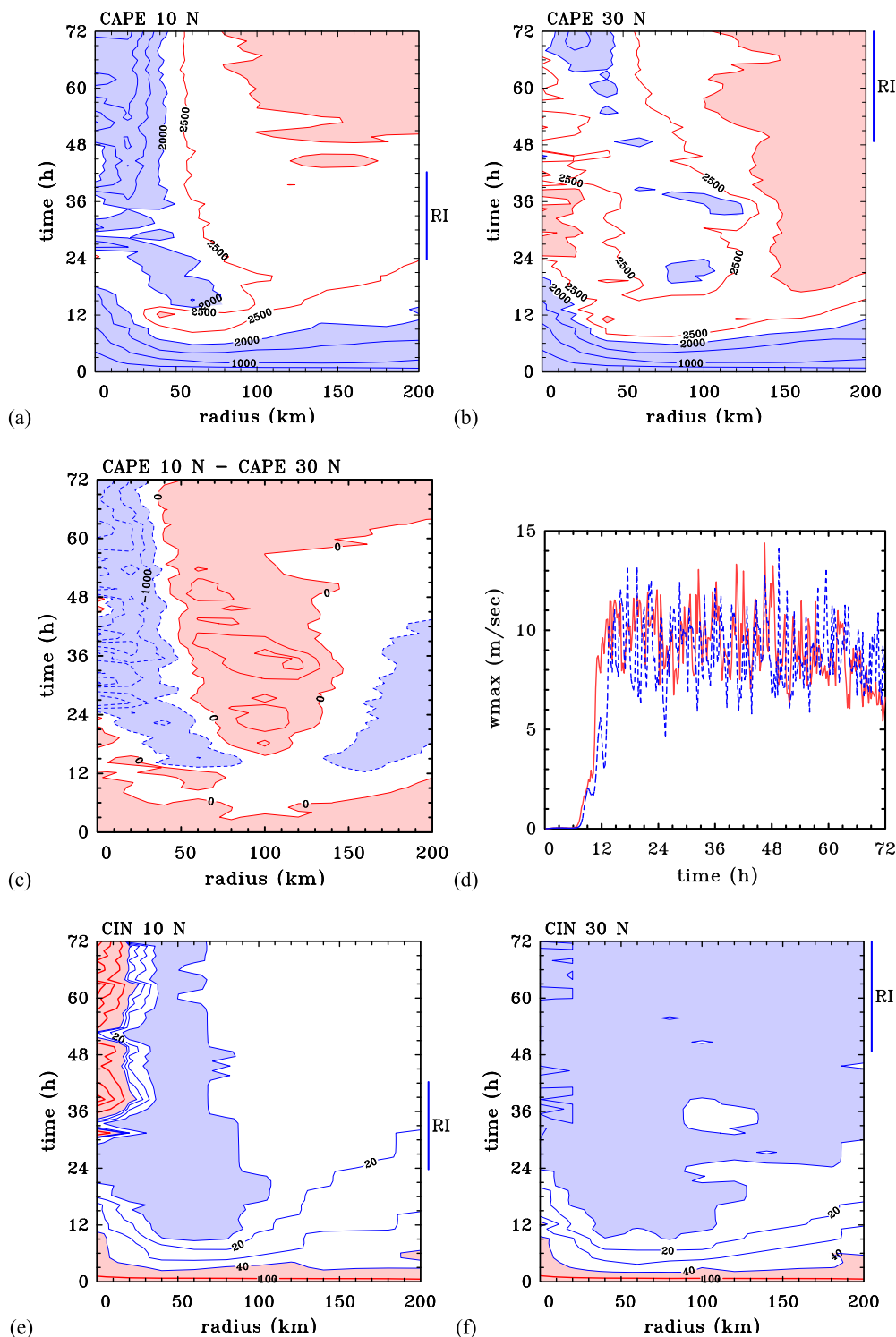
FIG. 6. Time-radius plots of CAPE based on azimuthally averaged thermodynamic data in the MM5 calculations of section 2 at (a) 10° and (b) 30°N; the contour interval is 500 J kg -1 , values below 2000 J kg -1 are shaded light blue, and values ≥ 3000 J kg -1 are shaded pink. (c) A similar plot of the difference in CAPE between these two calculations; the contour interval is 500 J kg -1 , values ≤ -500 J kg -1 are shaded light blue, and positive values are shaded pink. (d) A time series of the maximum vertical velocity (not azimuthally averaged) in the two calculations. (e),(f) The corresponding plots of CIN at 10° and 30°N, respectively (contours: 100, 40, 30, 20, and 10 J kg -1 ). Regions of CIN with values < 10 J kg -1 are shaded light blue, and values > 40 J kg -1 are shaded pink. The vertical lines to the right of (a),(b),(e), and (f) show the period of rapid intensification at the particular latitude (see Fig. 1).
