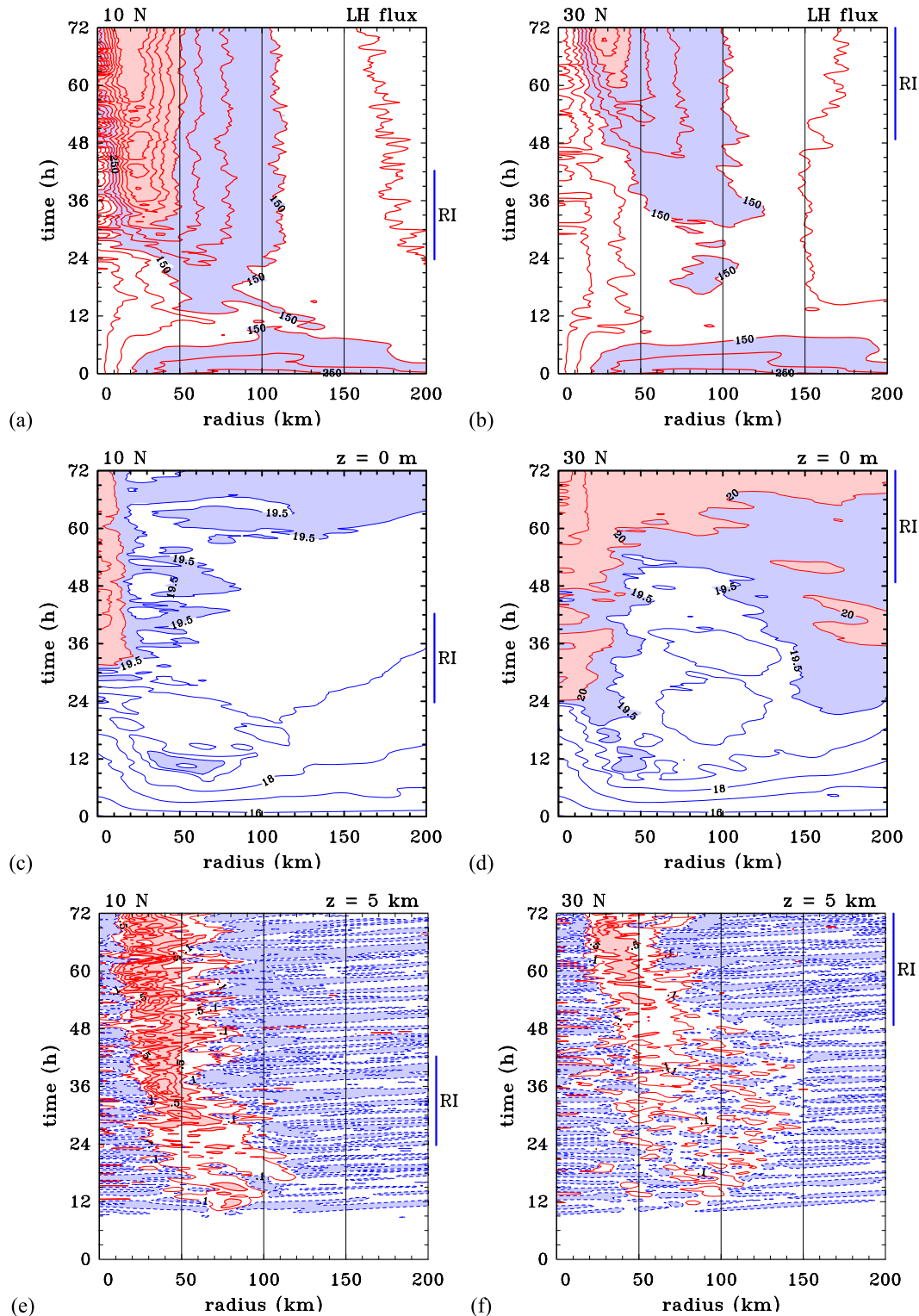
FIG. 4. Time–radius plots of azimuthally averaged surface latent heat fluxes in the MM5 calculations of section 2 at (a) 10^\circ and (b) 30^\circ\text{N} . (c),(d) The corresponding plots of specific humidity at the surface ( 0 \text{ m} ) and (e),(f) the contours of vertical velocity at a height of 5 \text{ km} . Contour intervals in (a) and (b) are 50 \text{ W m}^{-2} , values between 150 and 300 \text{ W m}^{-2} are shaded light blue, and values \geq 300 \text{ W m}^{-2} are shaded pink. Contour intervals in (c) and (d) are 1 \text{ g kg}^{-1} , values between 19.5 and 20 \text{ g kg}^{-1} are shaded light blue, and values \geq 20 \text{ g kg}^{-1} are shaded pink. In (e) and (f), the interval for the thick solid contours is 0.5 \text{ m s}^{-1} and values \geq 0.5 \text{ m s}^{-1} are shaded pink; the interval for the thin solid contours is 0.1 \text{ m s}^{-1} and values \leq -0.01 \text{ m s}^{-1} are shaded light blue. The vertical line to the right of each panel shows the period of rapid intensification at the particular latitude (see Fig. 1).
